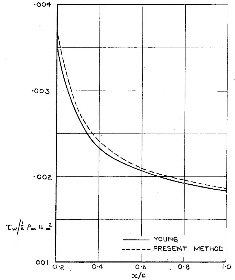
FIG. 2. Skin friction as calculated by two methods, in a particular case at zero heat transfer.
