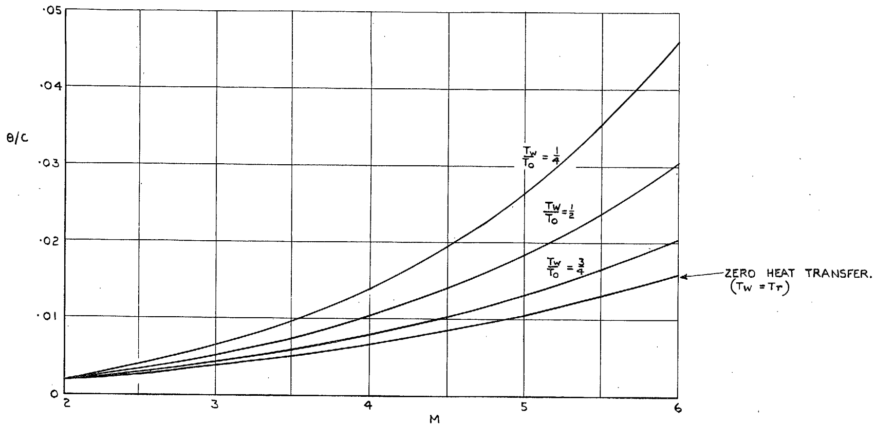
FIG. 3. Calculated growth of momentum thickness in a favourable pressure gradient at different wall temperatures.
