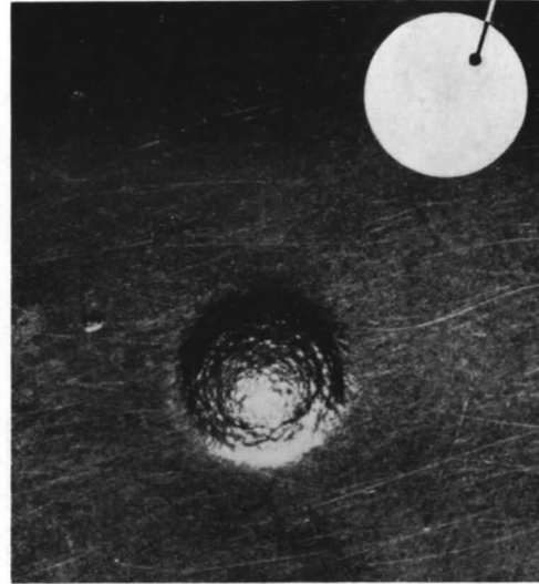
FIG. 25. Mark made on \frac{1}{4} -in. thick aluminium alloy, D.T.D. 423B, by a 2-mm diameter water drop at 3,200 ft/sec.
