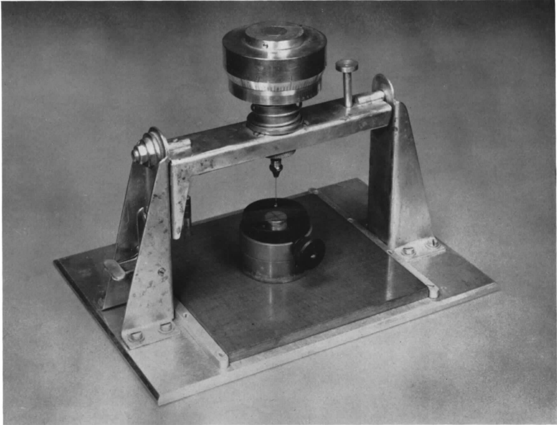
FIG. 22. Micro-burette assembly.
