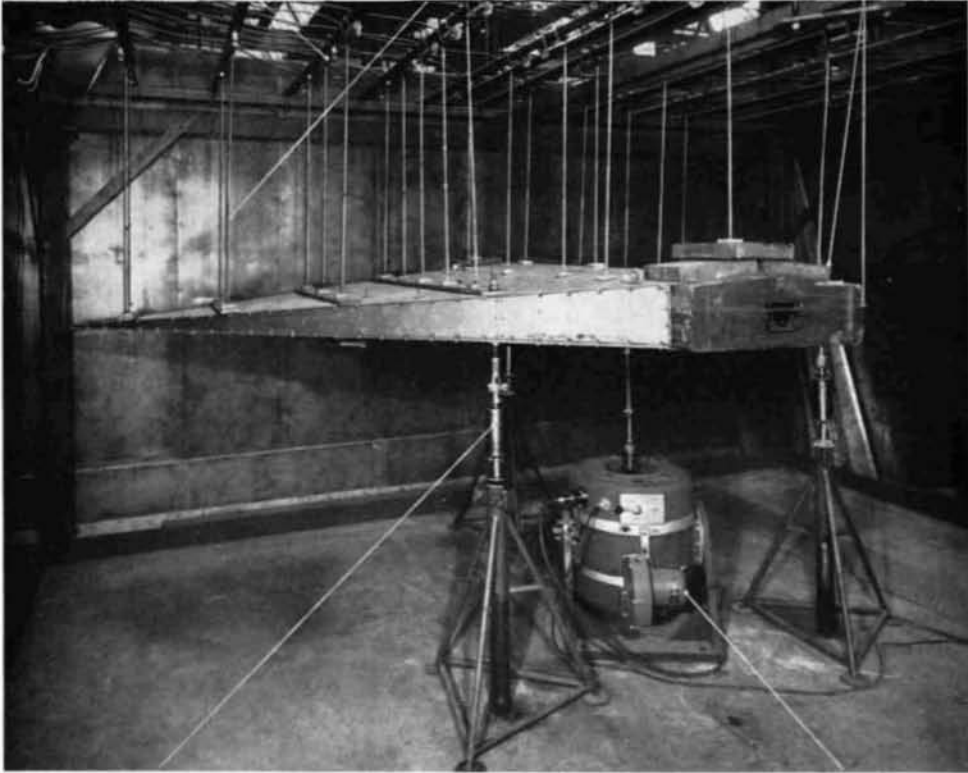
FIG. 2. General view of experimental set-up, model delta.
