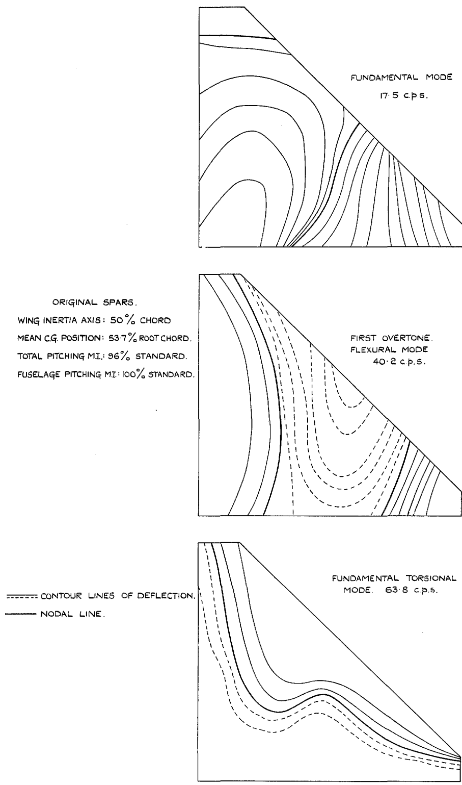
FIG. 9. Modes of vibration of model delta aircraft. Fourth inertia variation.
