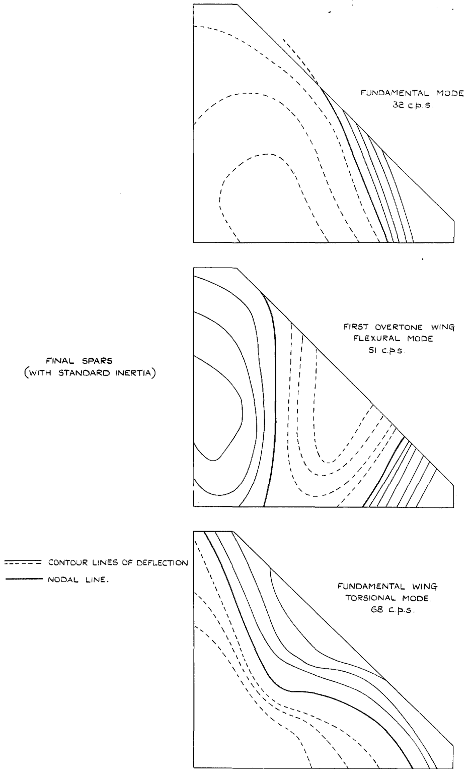
FIG. 6. Modes of vibration of model delta aircraft.
