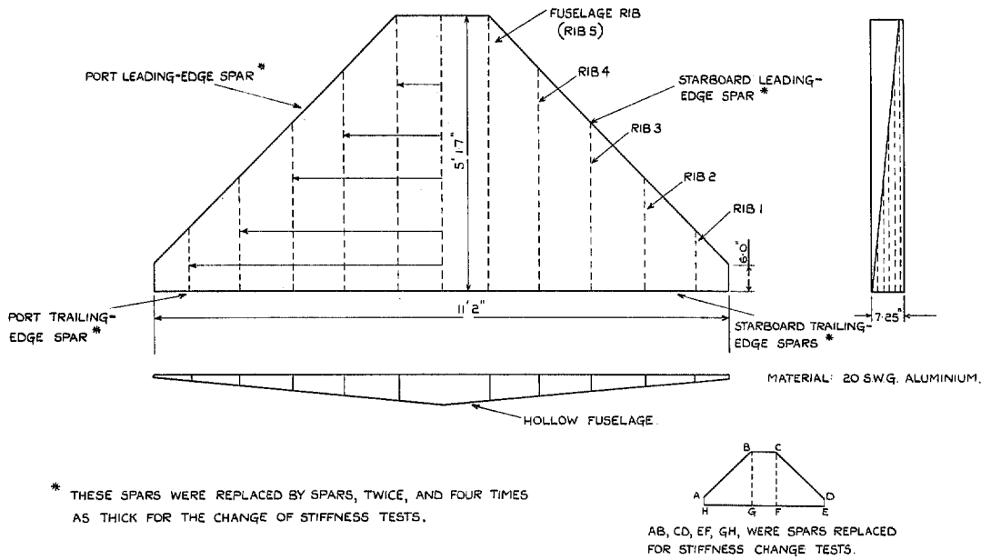
FIG. 1. Model delta aircraft.
