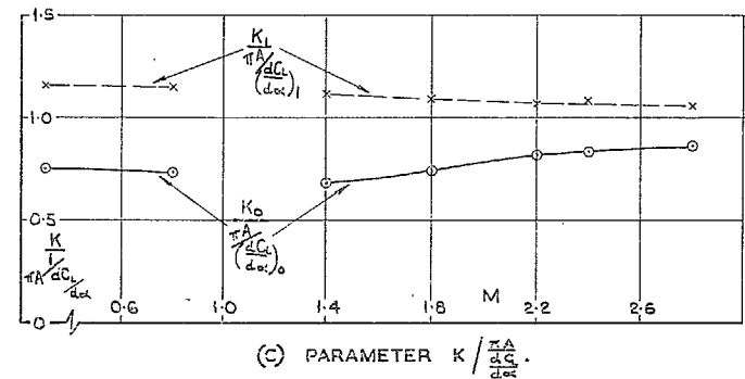
FIG. 20. Basic nose results; variation with Mach number of K , \alpha_K and K / \pi A / (dC_L / d\alpha) .
