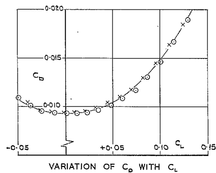
FIG. 9. Typical results showing derivation of mean curve; wing with fin, basic nose and inboard controls ( \eta_e = -4^\circ ), M = 1.8 .
