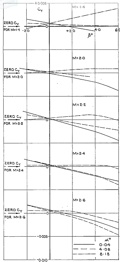
FIG. 39. Variation of C_Y with \beta at supersonic speeds; basic nose, no fin.
