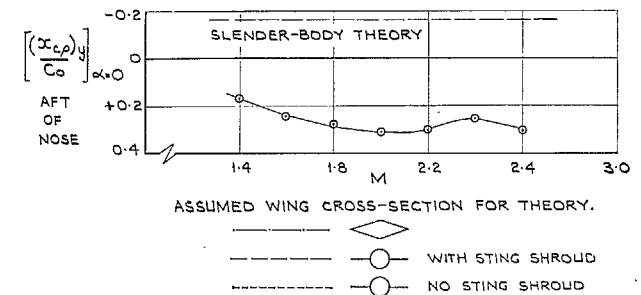
FIG. 47. Comparison with theory, (y_v)_{\alpha=0} , (n_v)_{\alpha=0} and [(x_{c.p.})_y / c_0]_{\alpha=0} ; basic nose, no fin.
