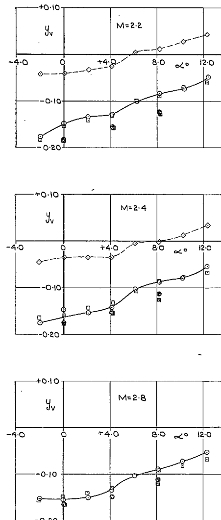
FIG. 55b. Effect of fin and canopy nose on y_v at supersonic speeds.
