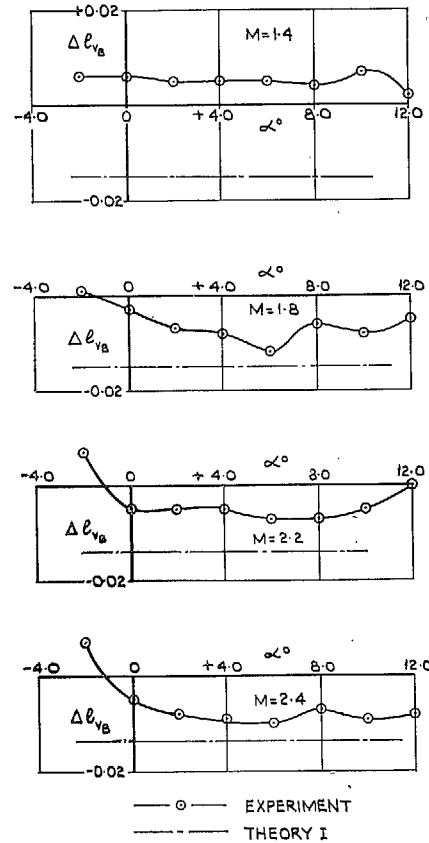
FIG. 60. Fin effectiveness; variation of \Delta l_{vB} due to fin with \alpha , basic nose.
