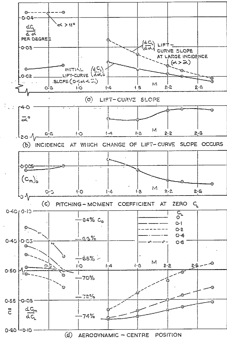
FIG. 15. Basic nose results; variation with Mach number of dC_L/d\alpha , \alpha , (C_m)_{C_L=0} and dC_m/dC_L .
