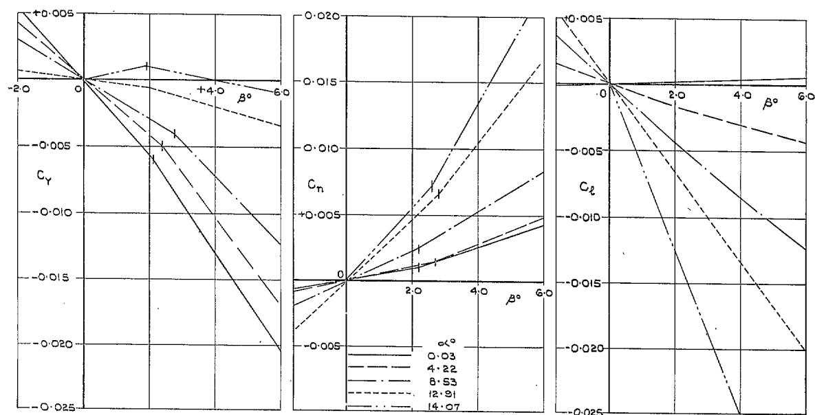
FIG. 65. Variation of C_Y , C_n and C_l with \beta at M = 0.3 , R = 8 \times 10^6 per ft; basic nose, with fin.
