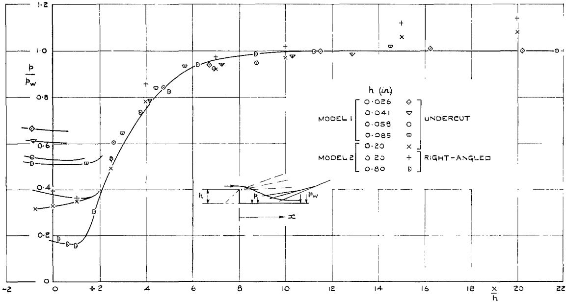
FIG. 6. Floor pressure distributions behind steps of various heights at a Mach number of 3.10.
