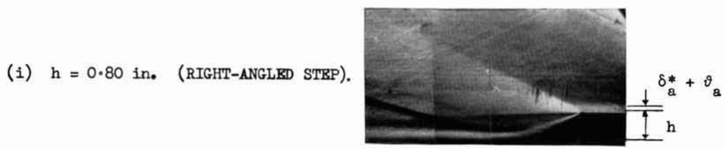
FIG. 7—concluded. Schlieren photographs of turbulent flow down steps; M_w = 2.41 , \delta_a^* = 0.0684 in., \vartheta_a = 0.0177 in.
