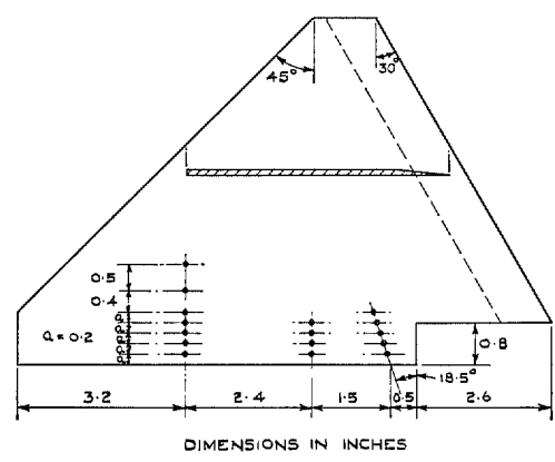
(b) LEADING DIMENSIONS OF REFLECTION PLATE.
