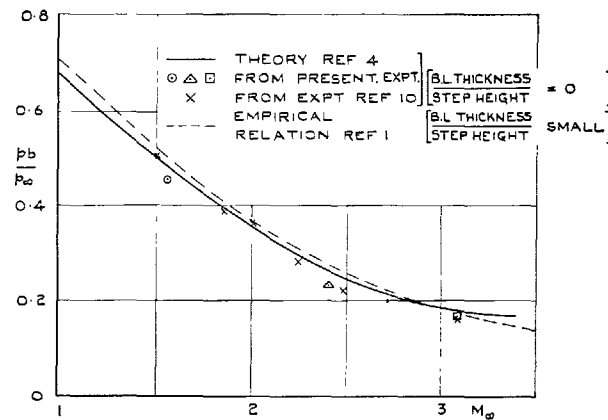
FIG. 14. Two-dimensional base-pressure ratios vs. Mach number for (boundary-layer thickness/step height) \rightarrow 0 .
