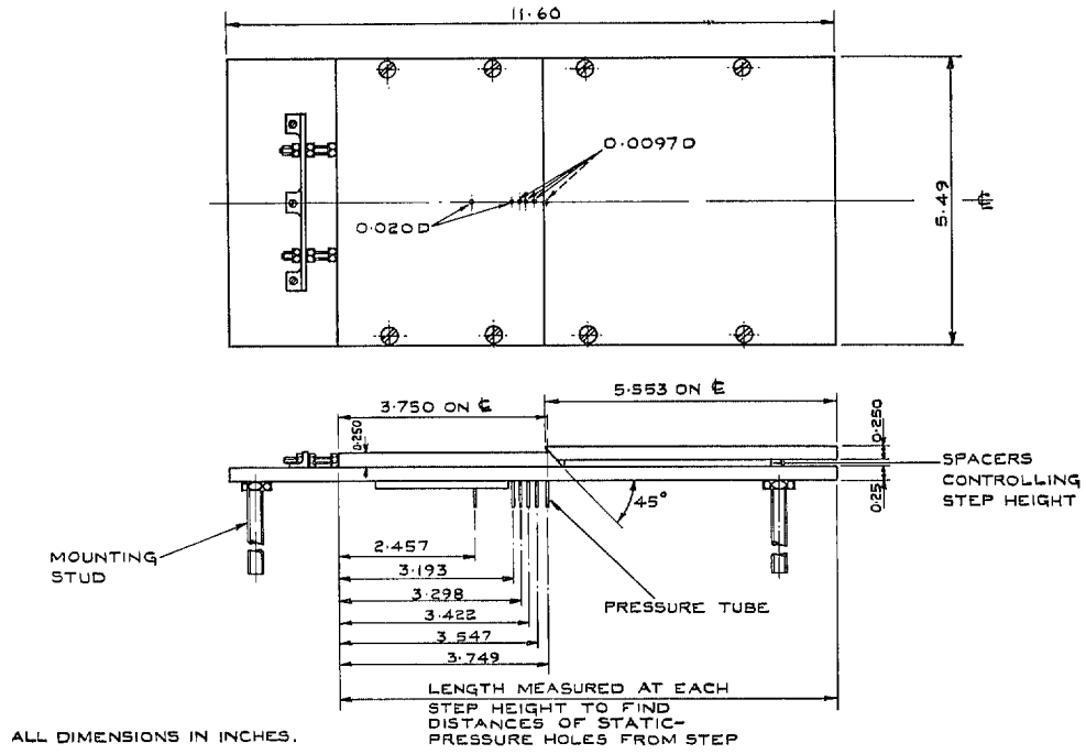
FIG. 1. Rearward-facing step model No. 1.
