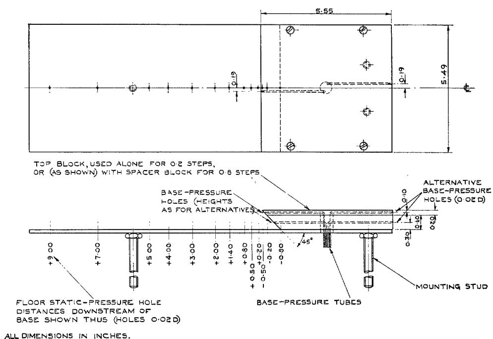
FIG. 2. Rearward-facing step model No. 2.
