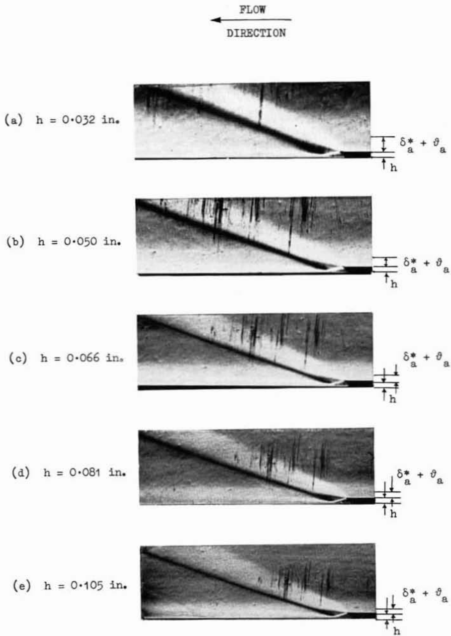
FIG. 7. Schlieren photographs of turbulent flow down steps; M_w = 2.41 , \delta_a^* = 0.0684 in., \vartheta_a = 0.0177 in.
