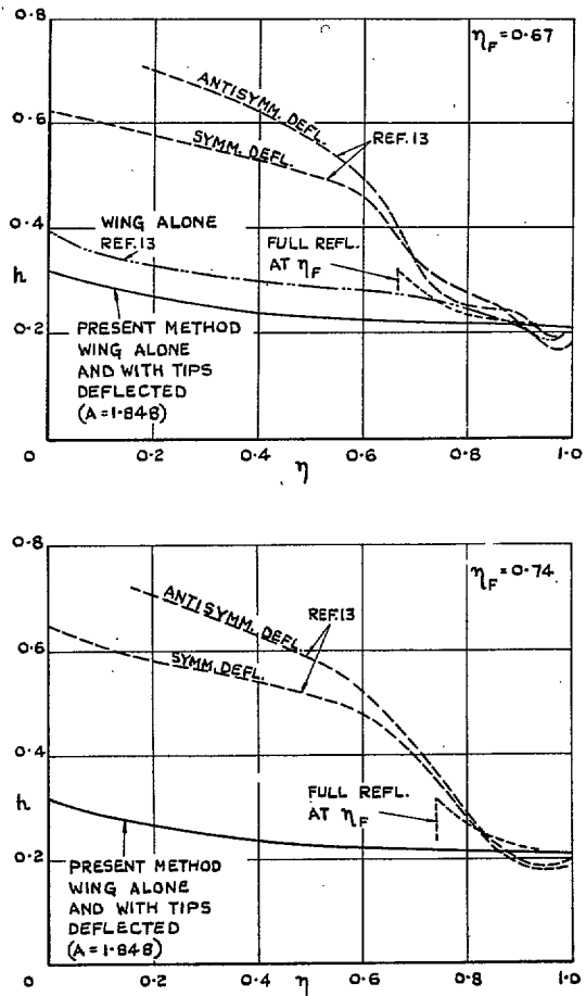
FIG. 21. Spanwise variation of the local aerodynamic centre for a delta wing with all-moving tip. A = 1.848 .
