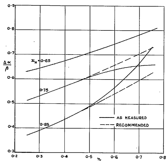
FIG. 11. Variation of equivalent incidence with ( \eta ).
