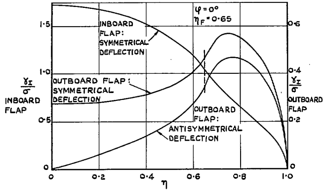
FIG. 5. Some typical Multhopp spanwise loading functions for discontinuous incidence.
