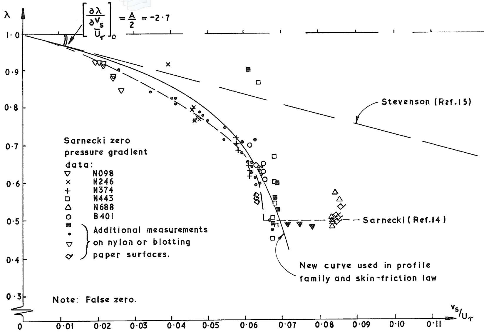
FIG. 2. Correlation of zero pressure gradient Bilog. profile parameter \lambda .
