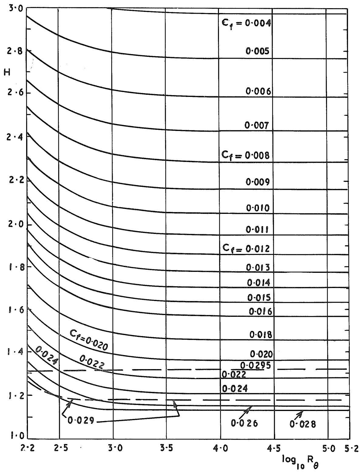
FIG. 19. Skin-friction chart for \frac{v_s}{U_1} = 0.015 .
