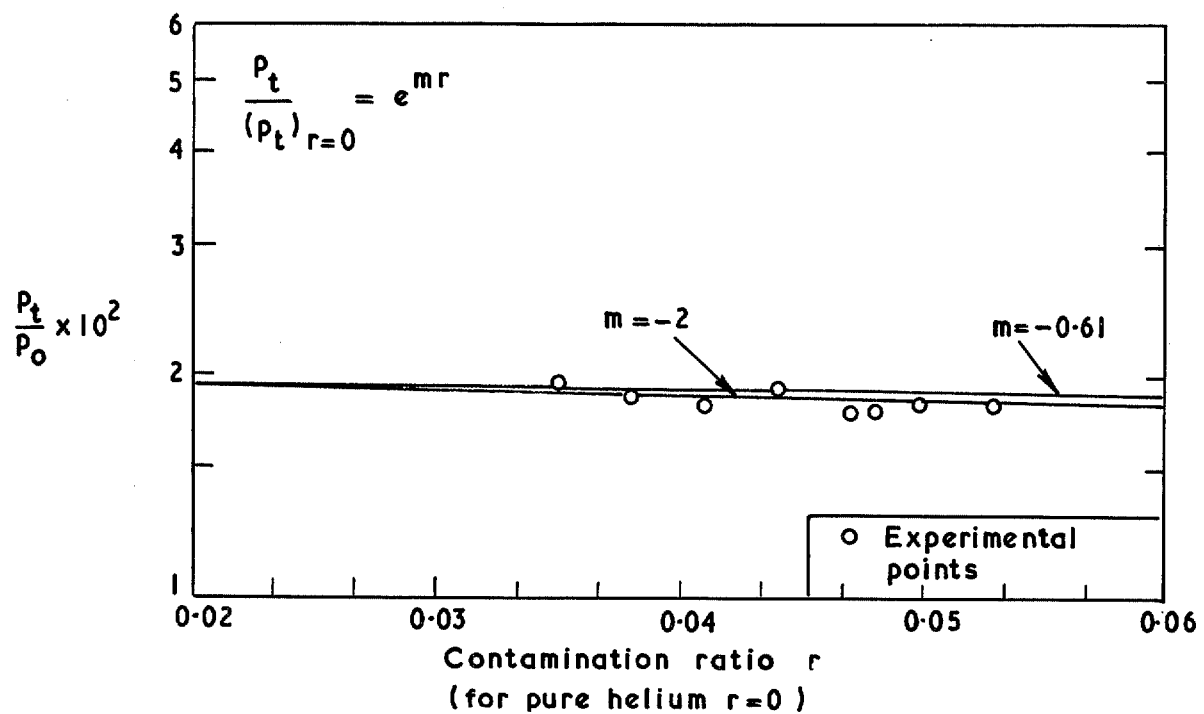
FIG. 3. Working section pitot pressure divided by reservoir pressure plotted as a function of contamination ratio, r ( M_\infty = 10.22 ).
