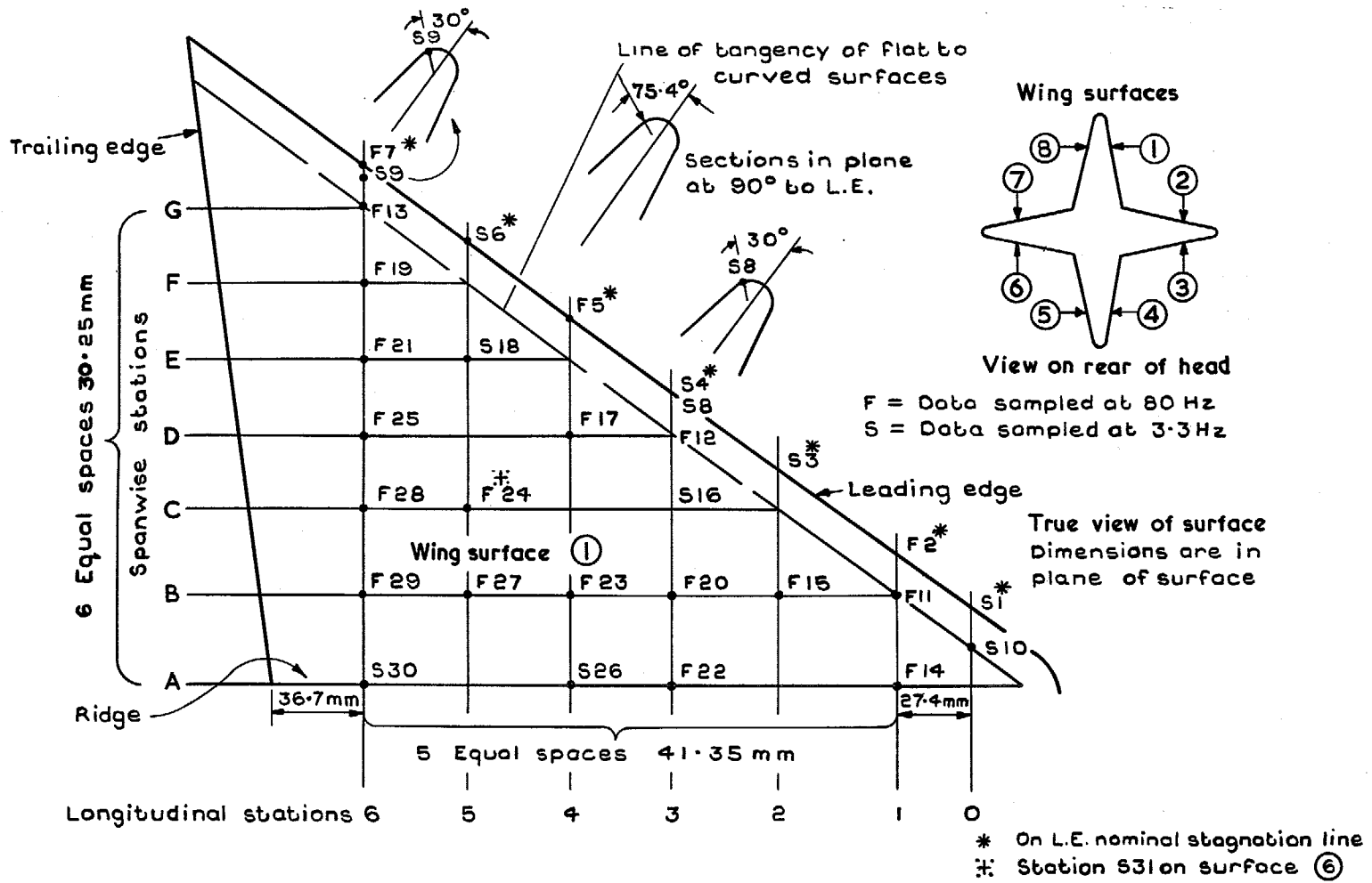
FIG. 20. Thermocouple locations.
