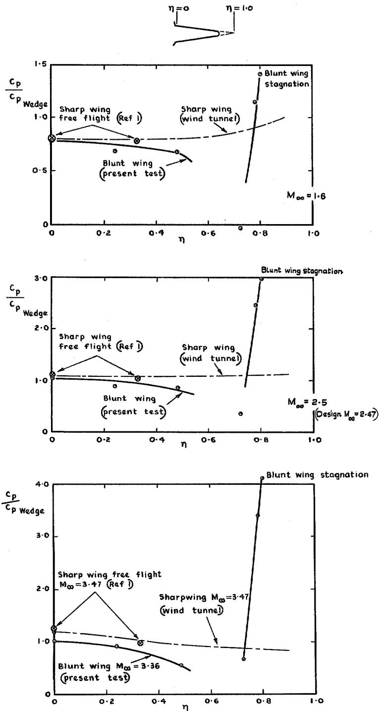
FIG. 17. Sharp/blunt wing comparison of spanwise pressure distribution—blunt wing data from longitudinal station 3 (Fig. 5) (accelerating flight).
