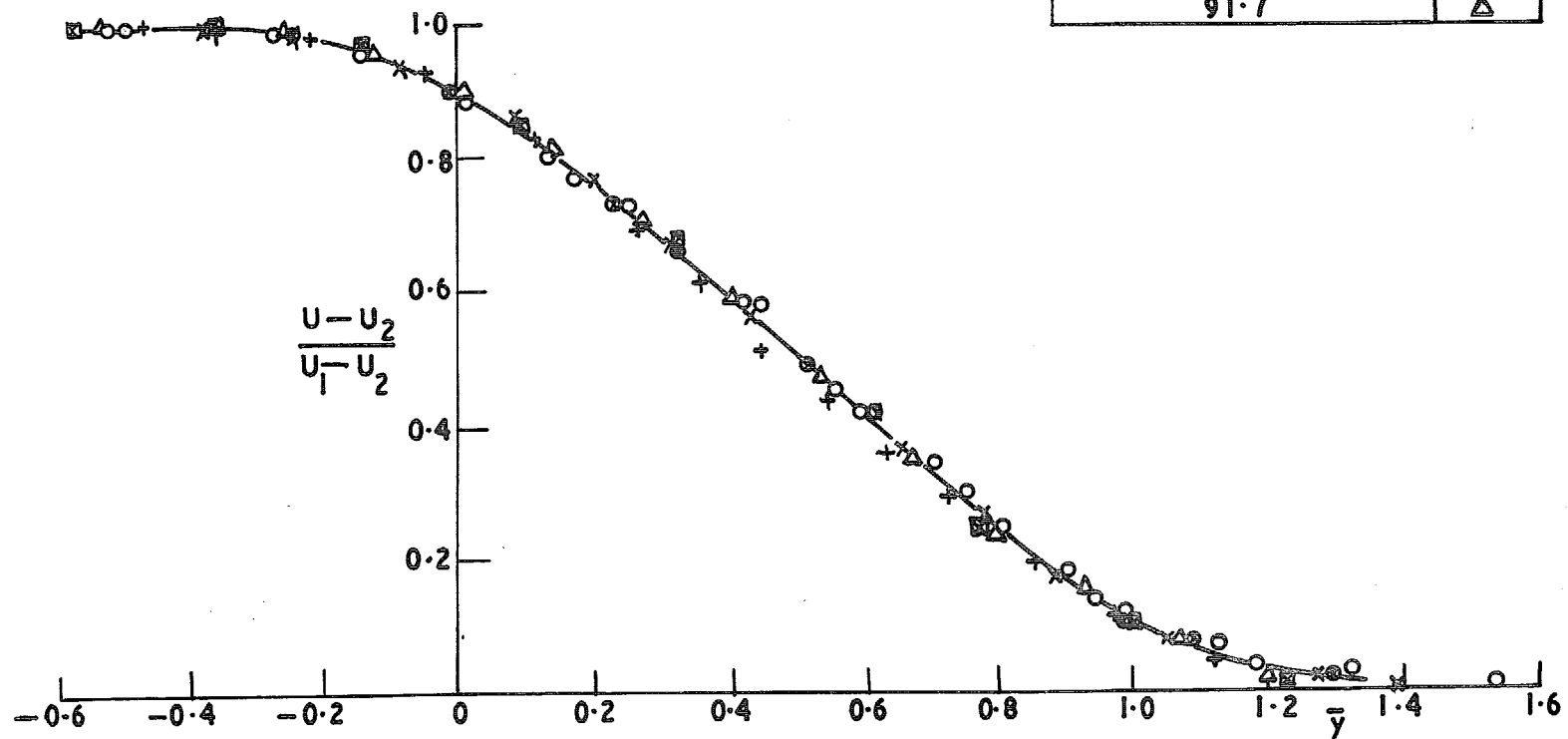
FIG. 4. Mean velocity measurements; U_2/U_1 = 0.61 .
