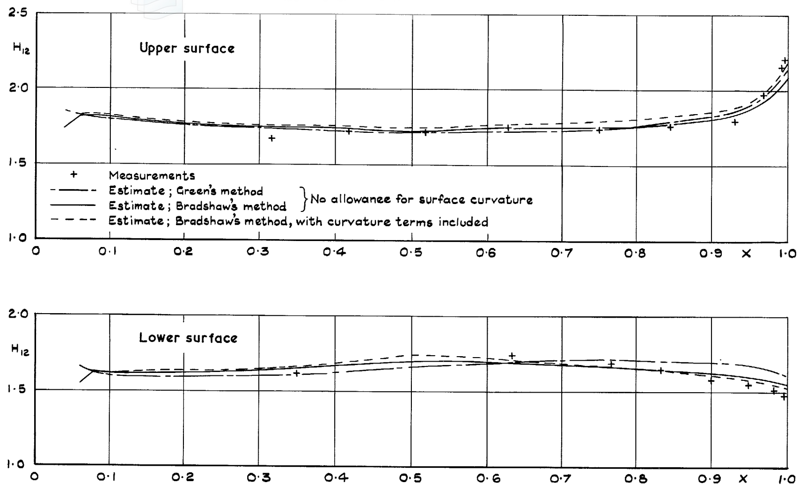
FIG. 18. Section 2814; boundary layer shape parameter, H_{12} .
