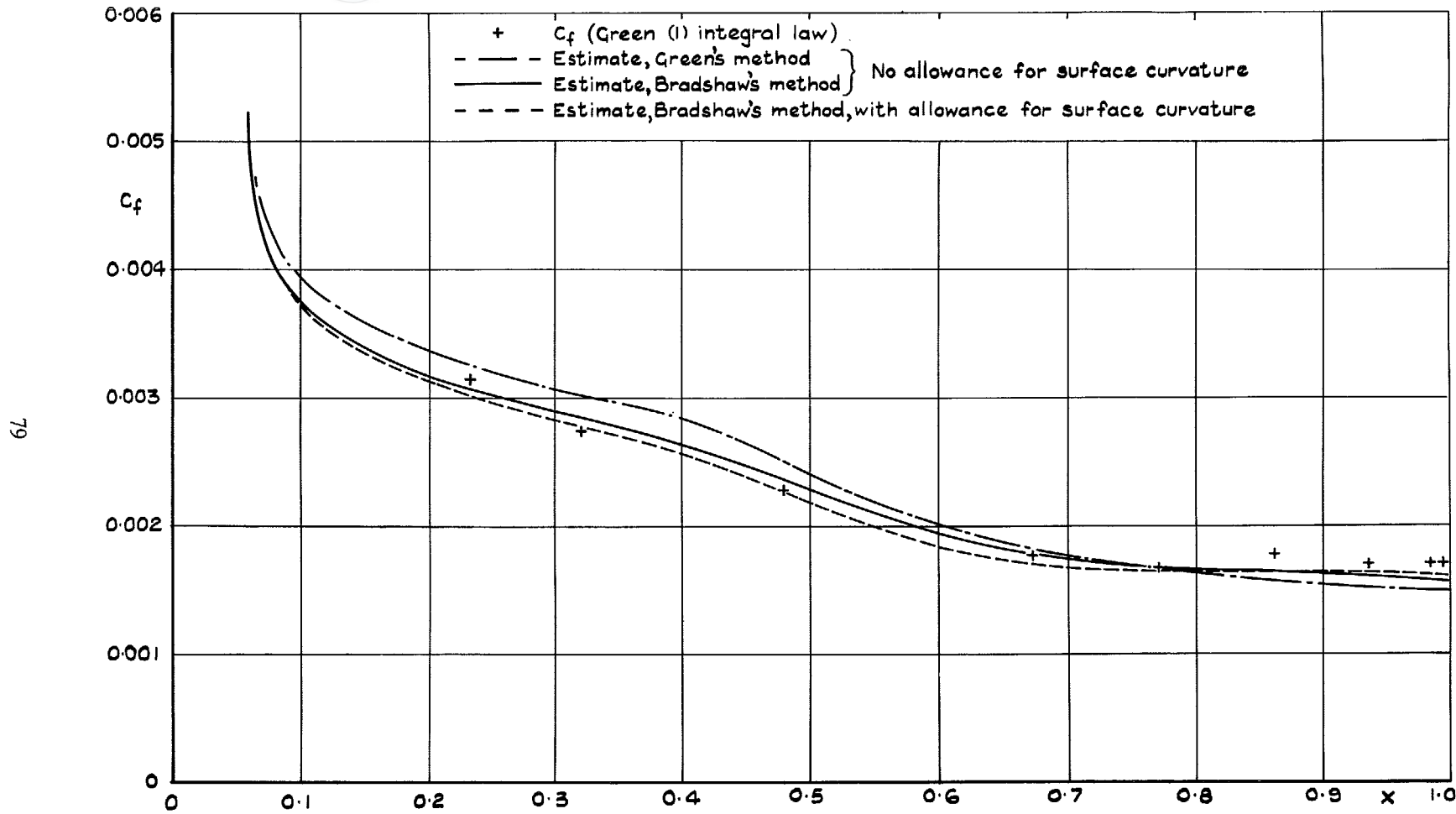
FIG. 24. Section 2815, C_L = 0.51 , lower surface: skin friction.
