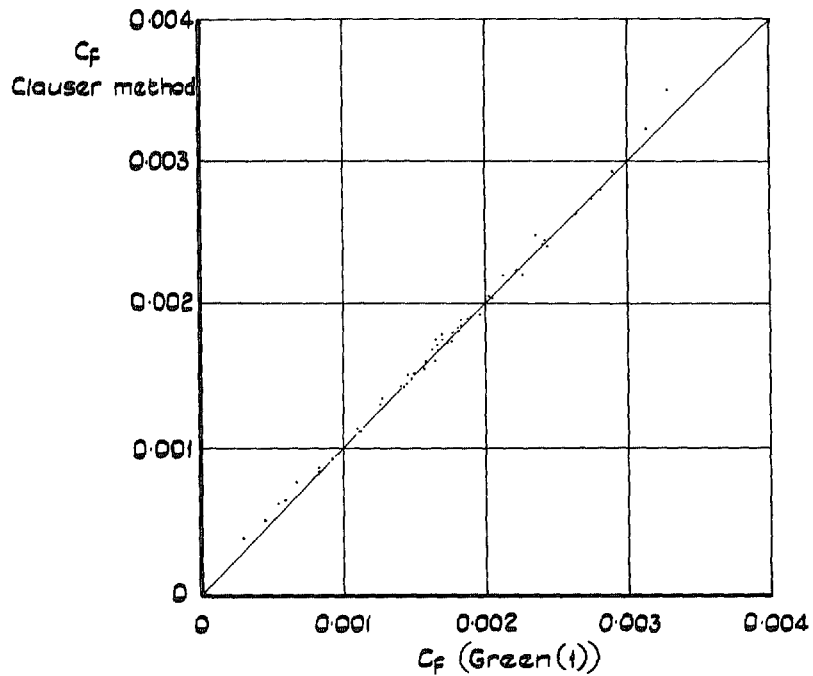
c Clauser method v Green(l) integral law
