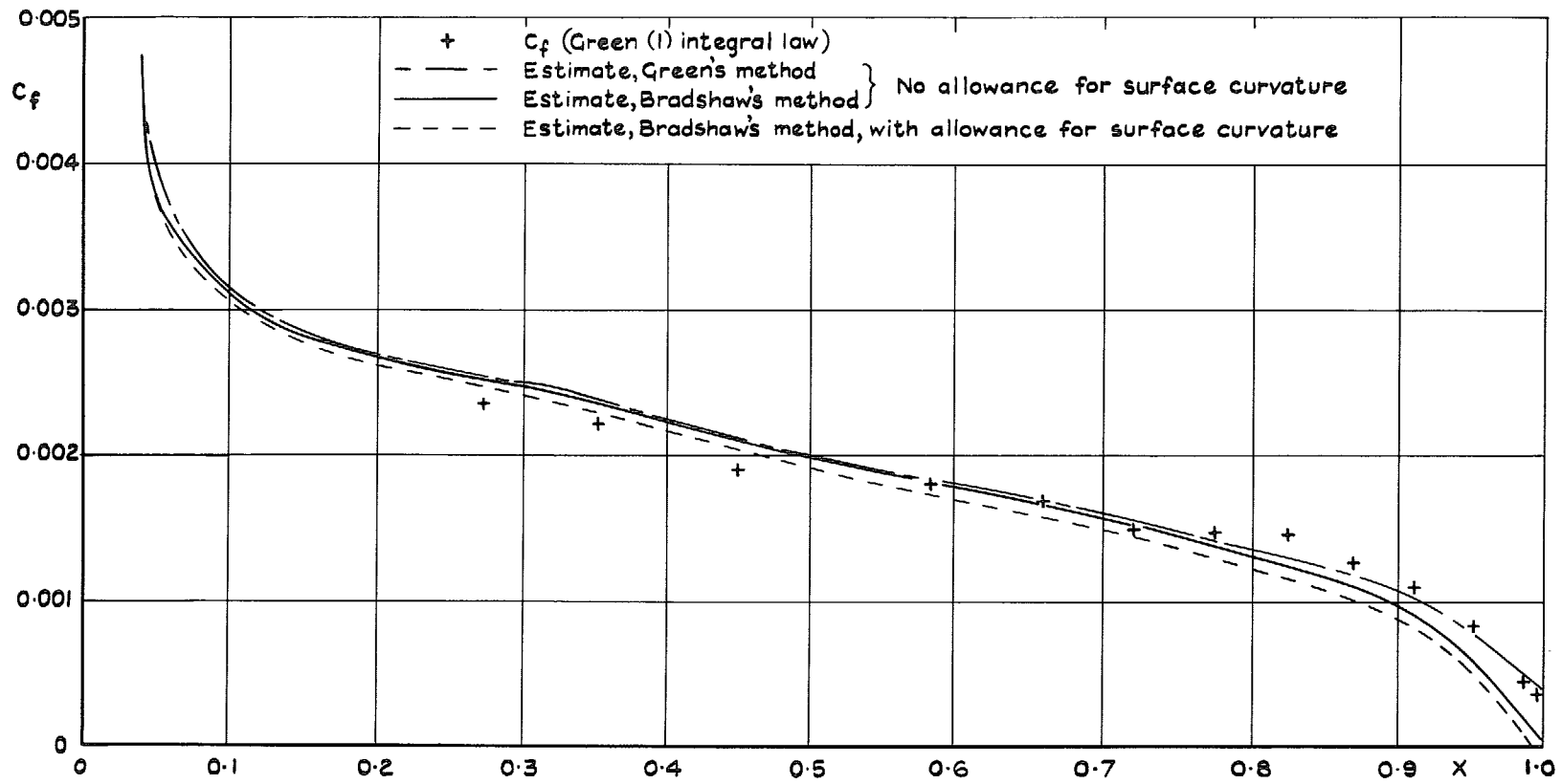
FIG. 23. Section 2815, C_L = 0.51 , upper surface: skin friction.
