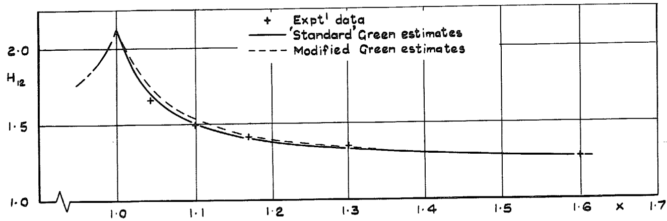
FIG. 31. Section 2815, C_L = 0.51 : wake development.
