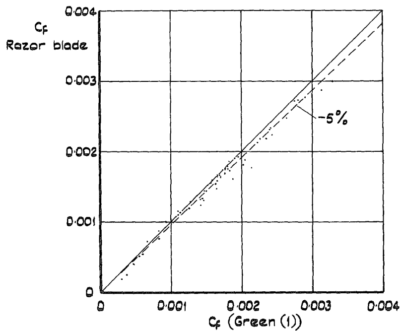
d Razor blade method v Green(l) integral law
