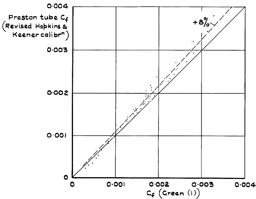
f Preston tube (revised Hopkins & Keener calibr n ) v Green (I) integral law
