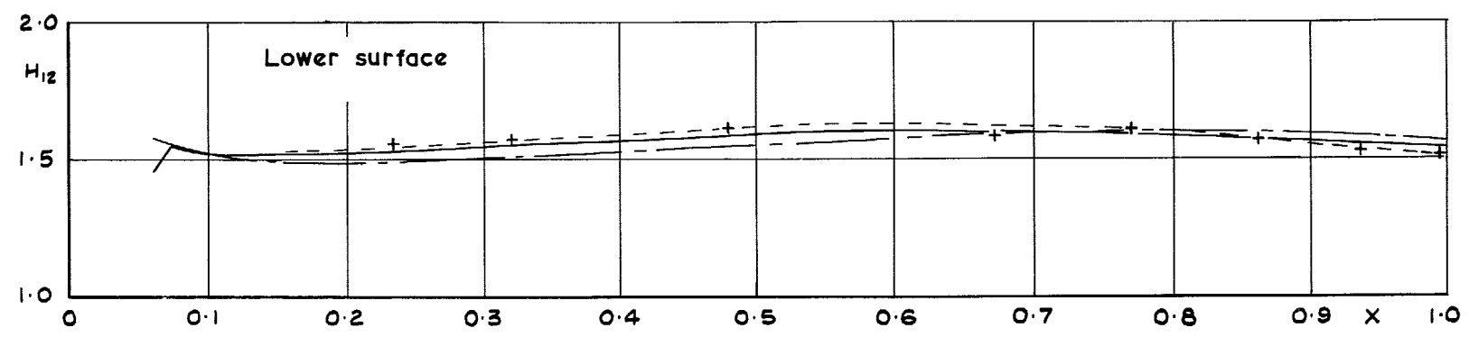
FIG. 20. Section 2815, C_L = 0.70 : boundary layer shape parameter.
