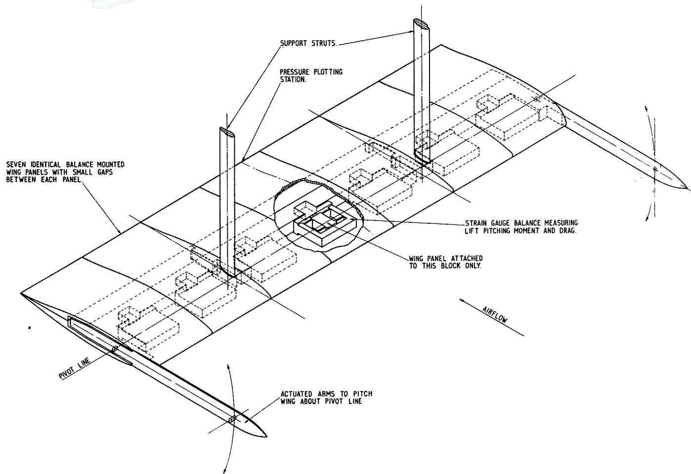
FIG. 3. Isometric sketch of wing and support system.
