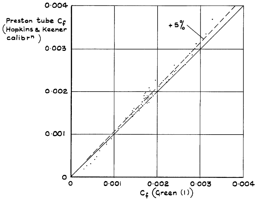
e Preston tube (Hopkins & Keener calibr n ) v Green (I) integral law
