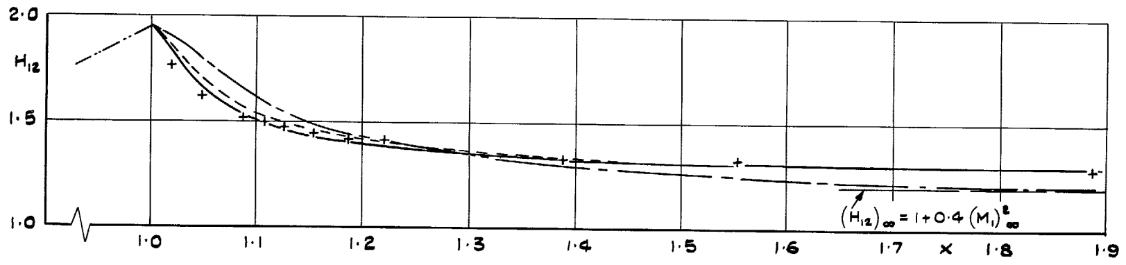
FIG. 30. Section 2814: wake development.
