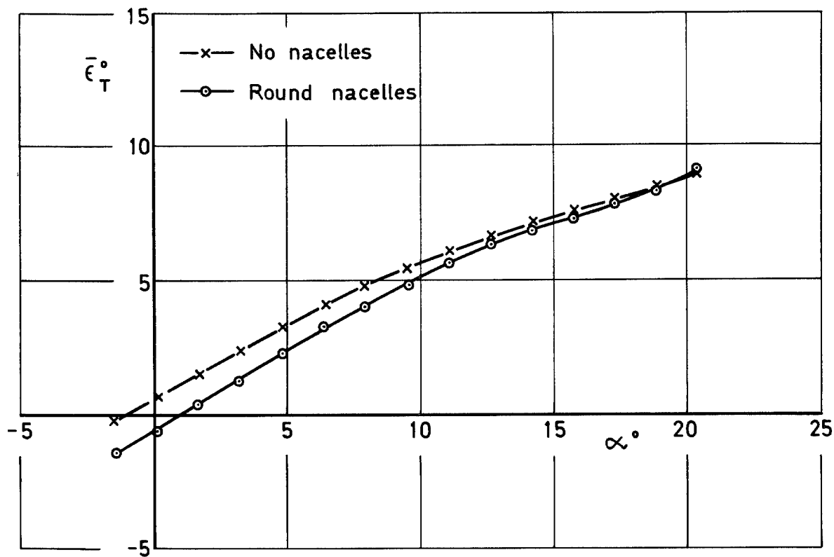
FIG. 48. Effect of nacelles on mean downwash angle at tailplane for high-wing model with slats 25^\circ and flaps 10^\circ .
