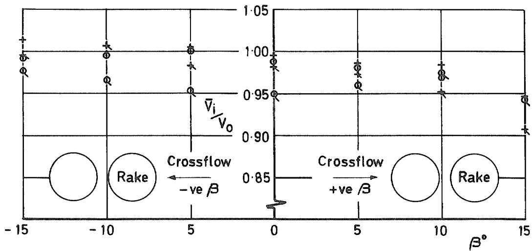
FIG. 15. Variation of entry velocity ratio with sideslip for round nacelles, slats 25° and flaps 40°.
