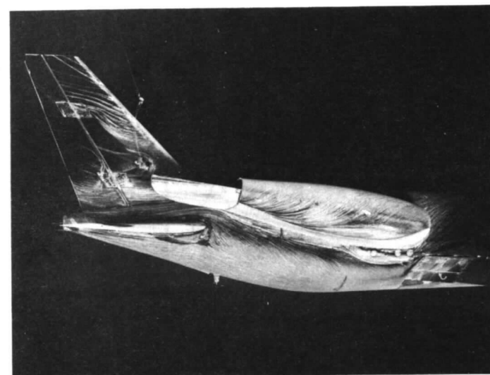
FIG. 45 a and b. Surface flow patterns at \alpha = 10^\circ on flat nacelles and adjacent surfaces, with low-wing model slats 25^\circ and flaps 40^\circ , \eta_B = 0^\circ .
