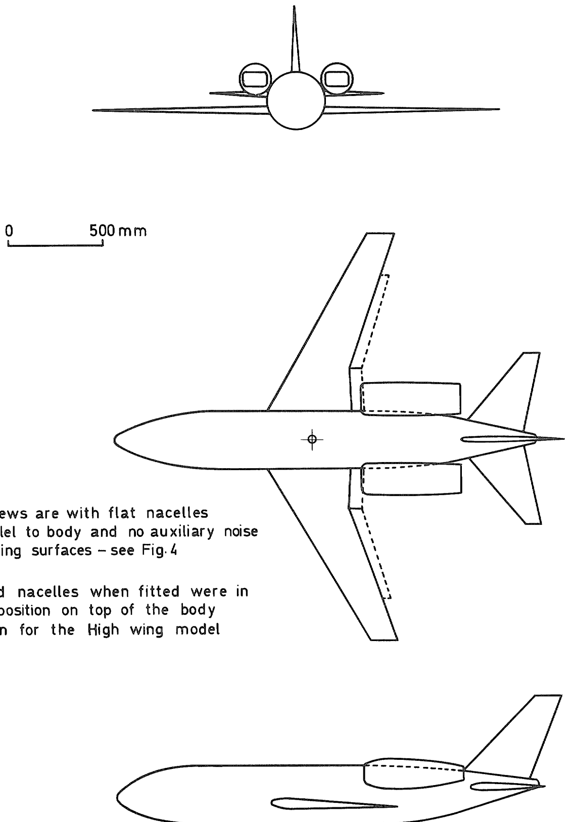
FIG. 2. G.A. of low-wing model.
