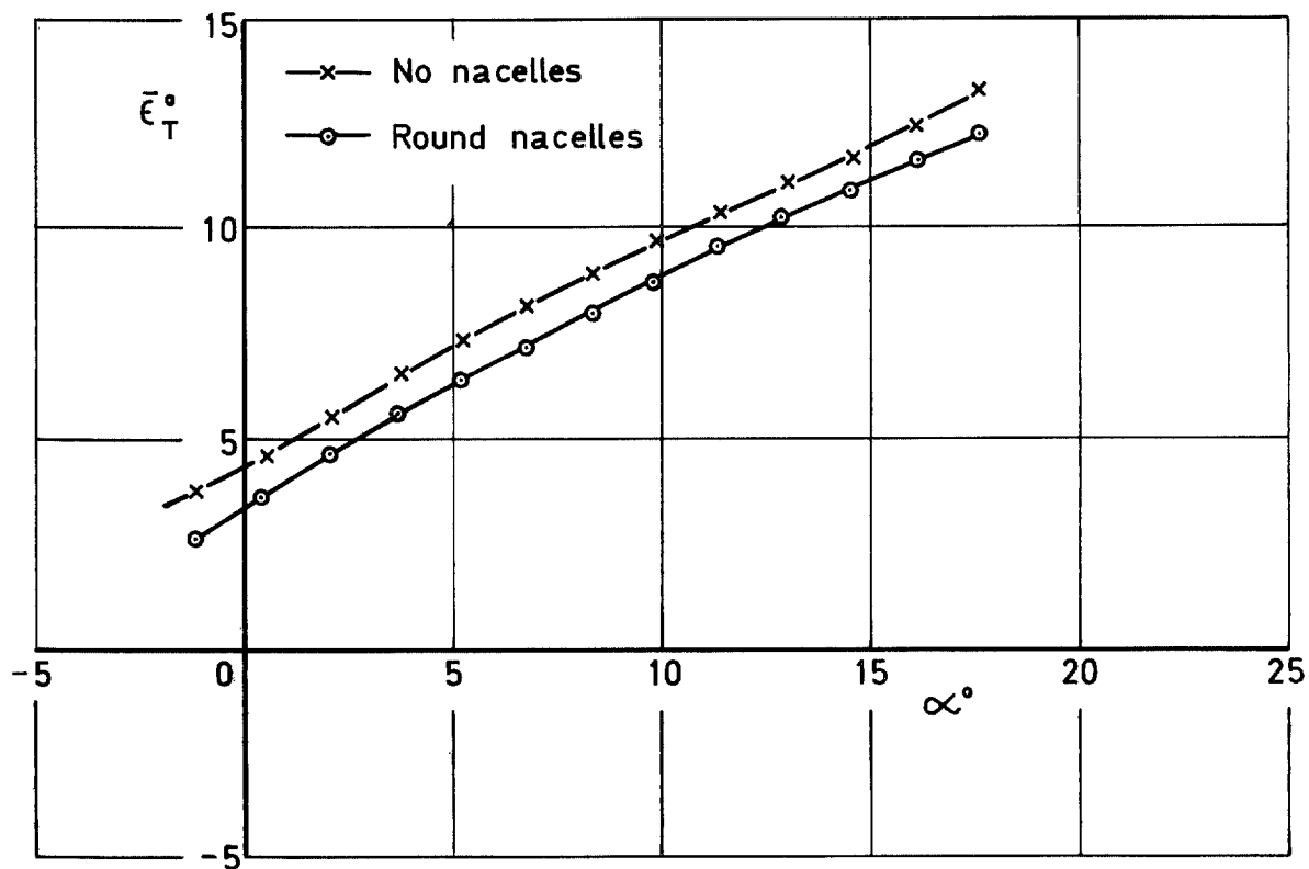
FIG. 49. Effect of nacelles on mean downwash angle at tailplane for high-wing model with slats 25^\circ and flaps 40^\circ .
