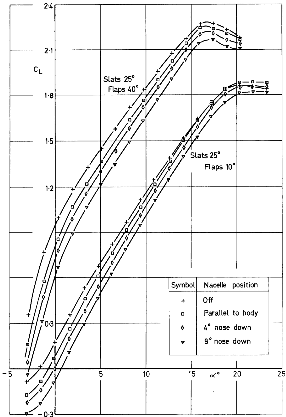
FIG. 33. Effect of flat nacelles on lift coefficient of low-wing model without tailplane, flaps 10° and 40°.
