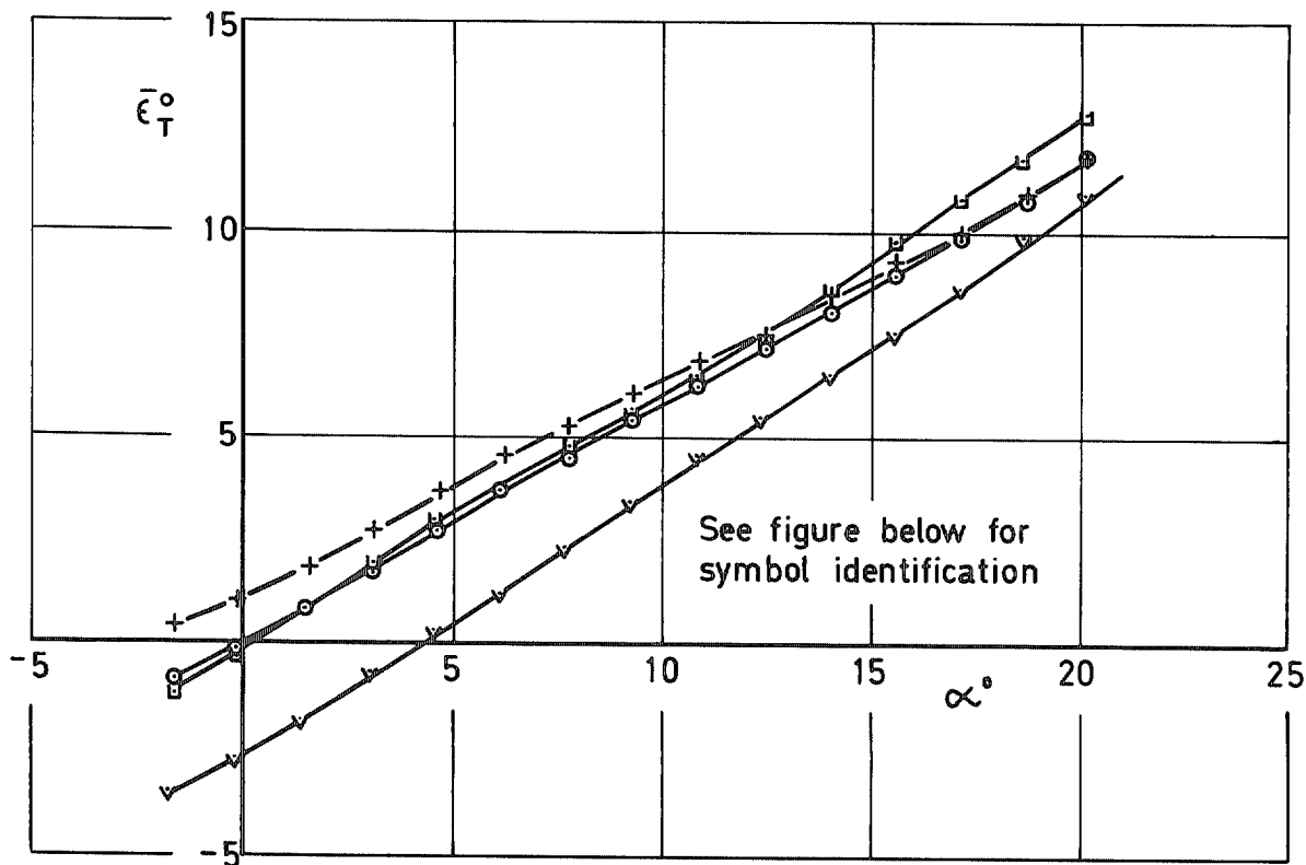
FIG. 50. Effect of nacelles on mean downwash angle at tailplane for low-wing model with slats 25° and flaps 10°.
