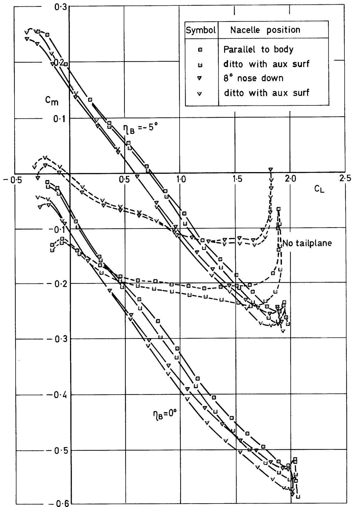
FIG. 41. Effect of adding auxiliary noise-shielding surfaces on pitching moment coefficient of low-wing model with flat nacelles, slats 25^\circ and flaps 10^\circ .
