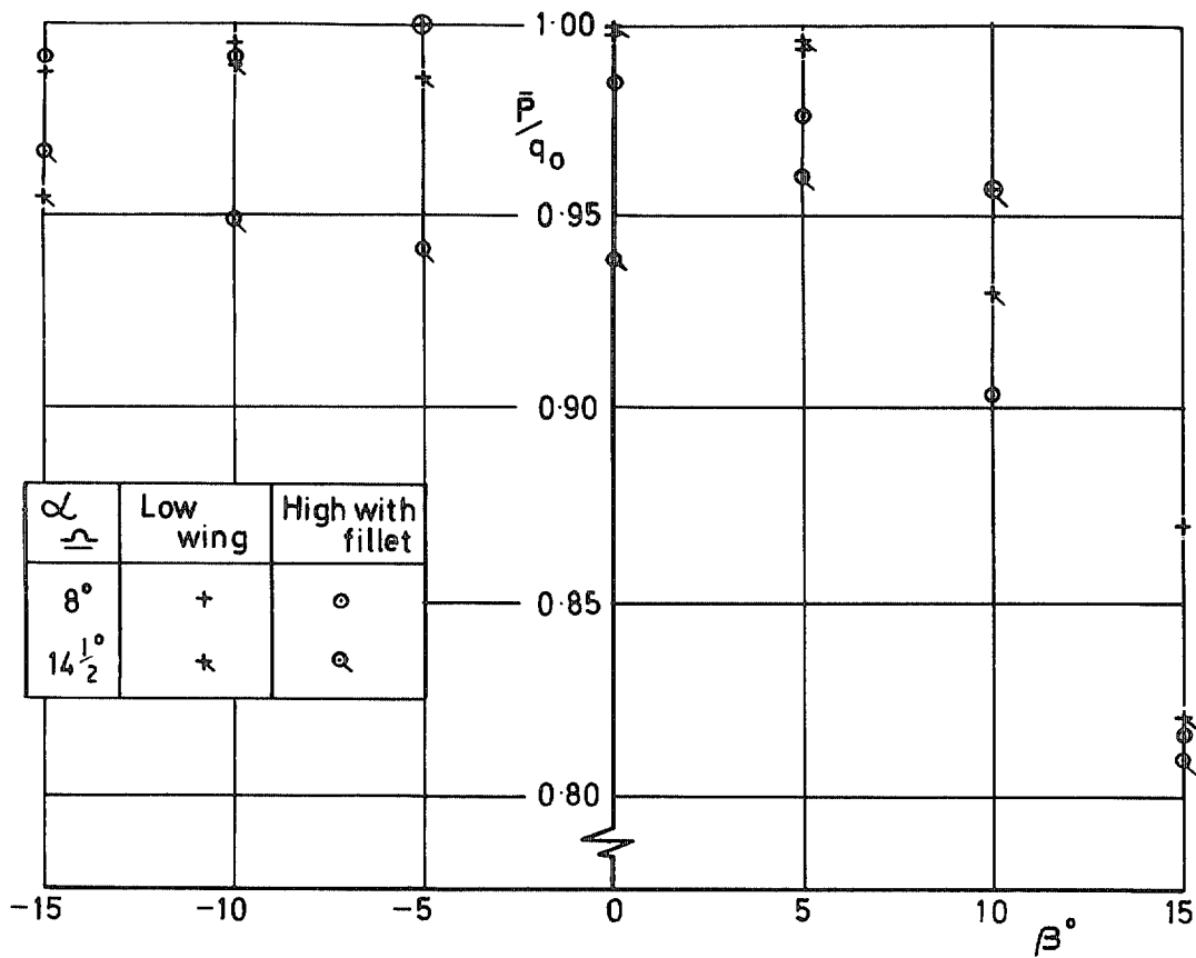
FIG. 14. Variations of total head at ‘engine face’ with sideslip for round nacelles, slats 25° and flaps 40°.
