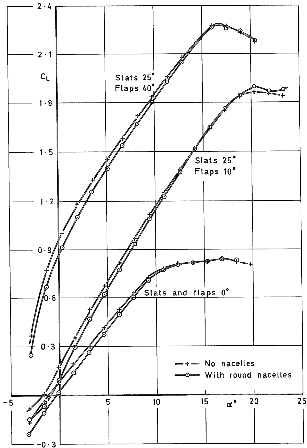
FIG. 23. Effect of round nacelles on lift coefficient of low-wing model without tailplane.
