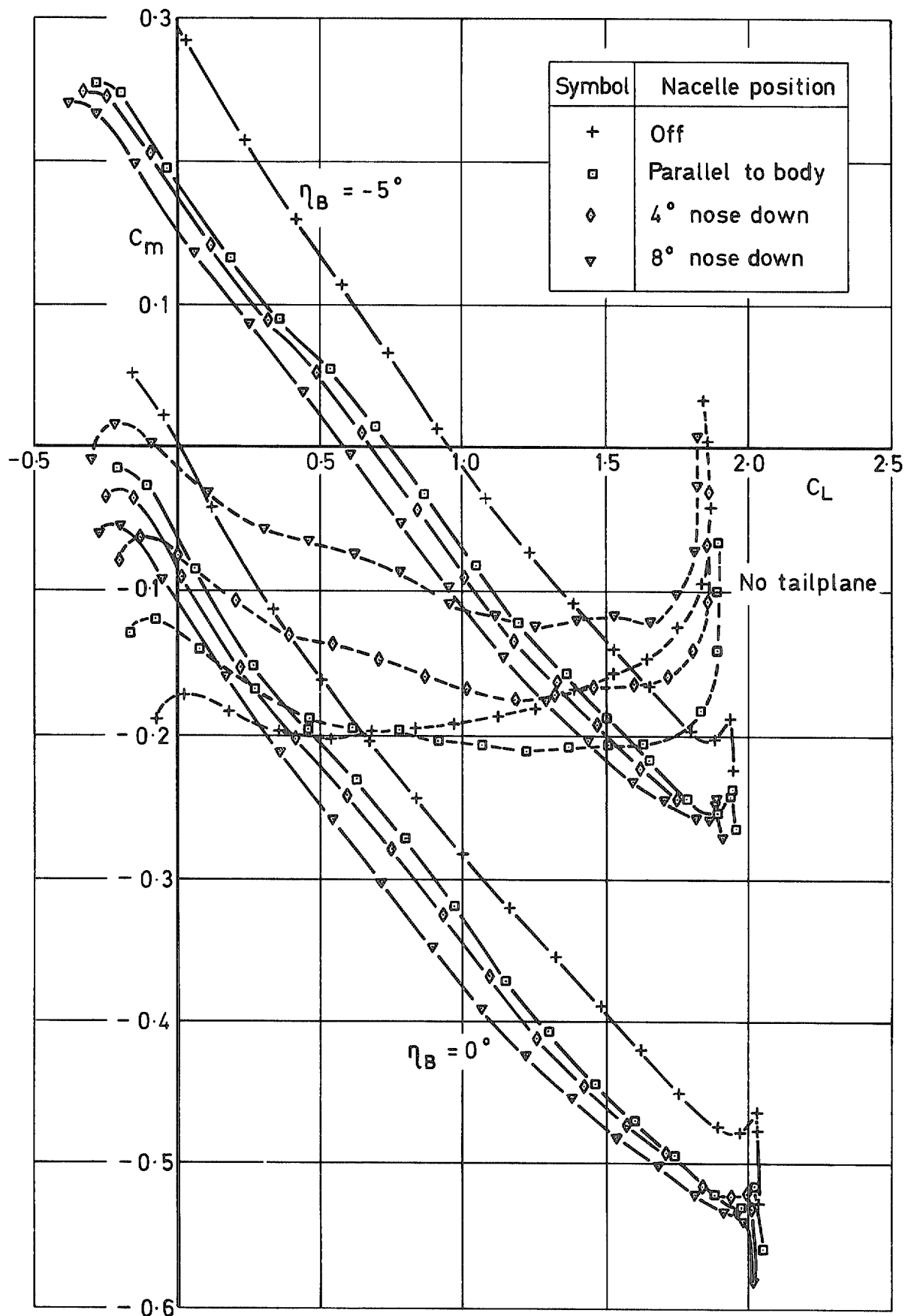
FIG. 38. Effect of flat nacelles on pitching moment coefficient of low-wing model with slats 25^\circ and flaps 10^\circ .
