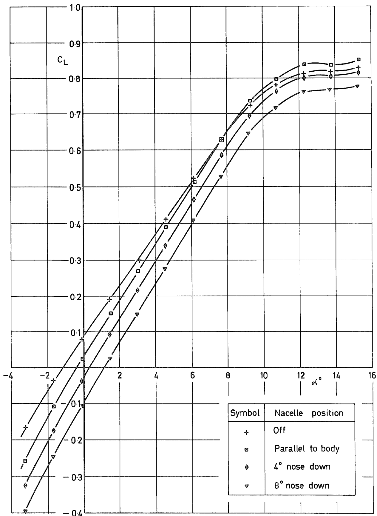
FIG. 32. Effect of flat nacelles on lift coefficient of low-wing model without tailplane, slats and flaps 0°.
