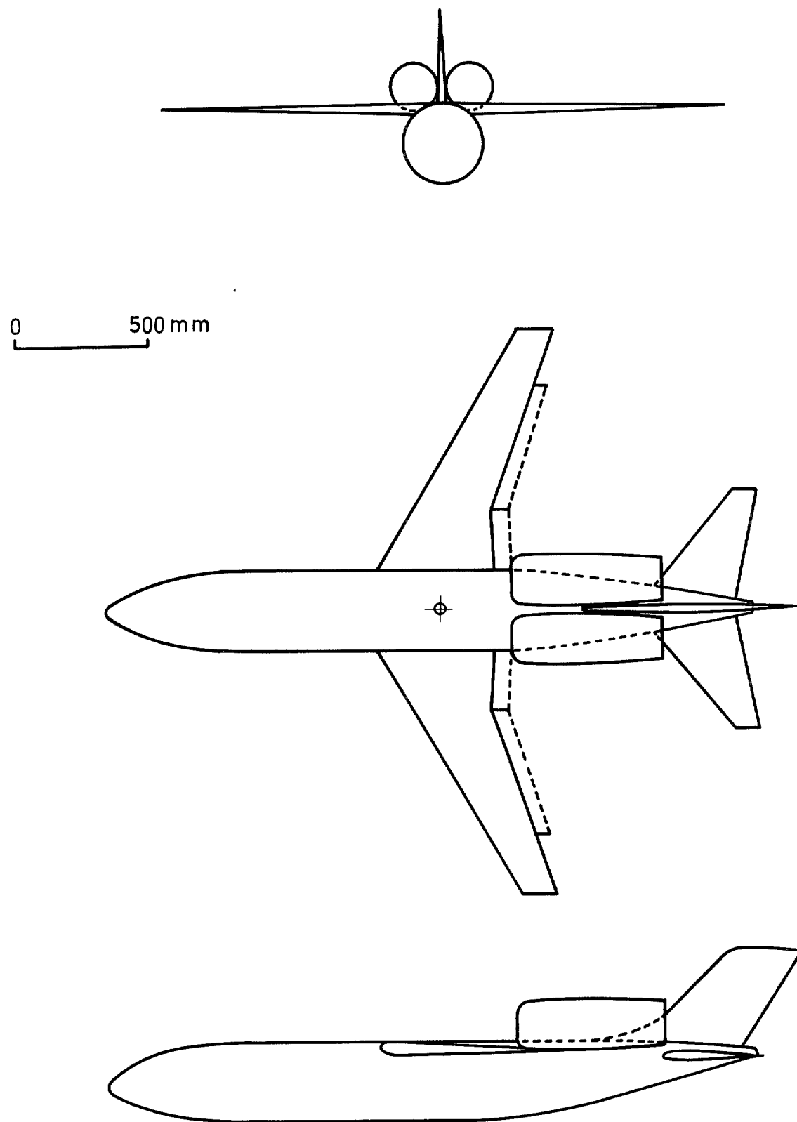
FIG. 1. G.A. of high-wing model.
