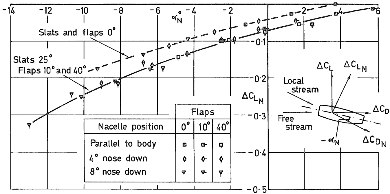
a Lift coefficient
