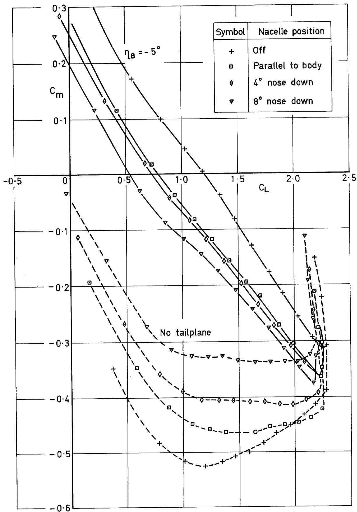
FIG. 39. Effect of flat nacelles on pitching moment coefficient of low-wing model with slats 25° and flaps 40°
