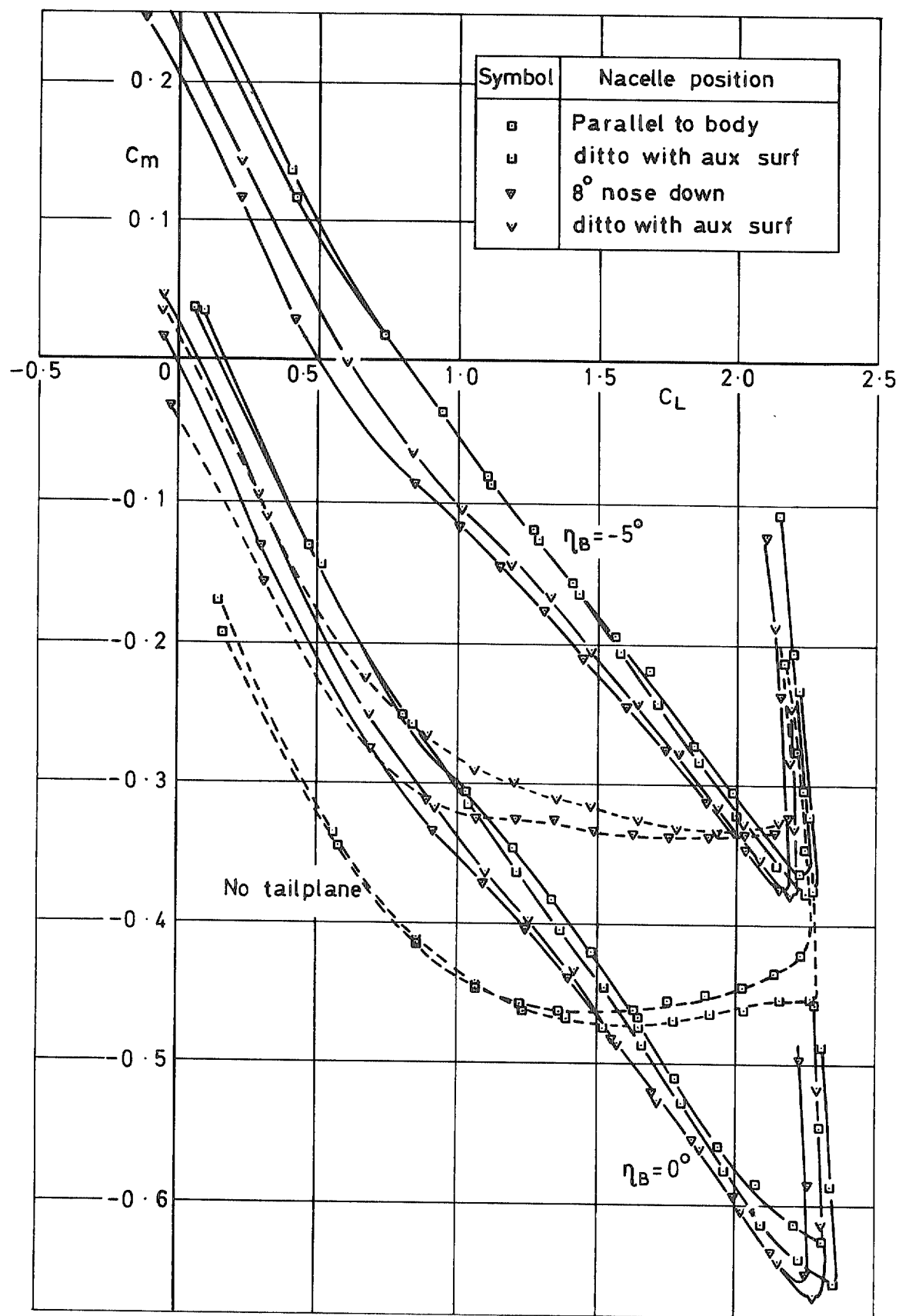
FIG. 42. Effect of adding auxiliary noise-shielding surfaces on pitching moment coefficient of low-wing model with flat nacelles, slats 25° and flaps 40°.
