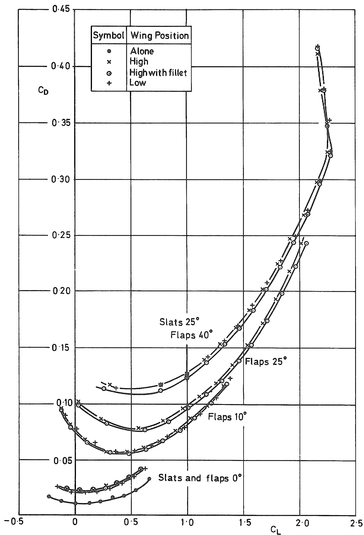
FIG. 8. Drag coefficient for various wing conditions.
