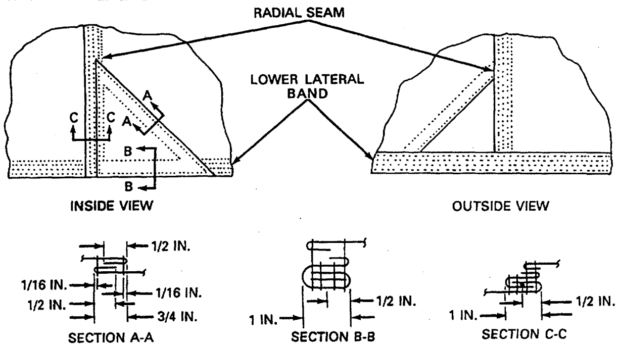
H TRIANGULAR PATCH INCLUDING RADIAL SEAM AND LOWER LATERAL BAND, CONTINUOUS-LINE CANOPY.
