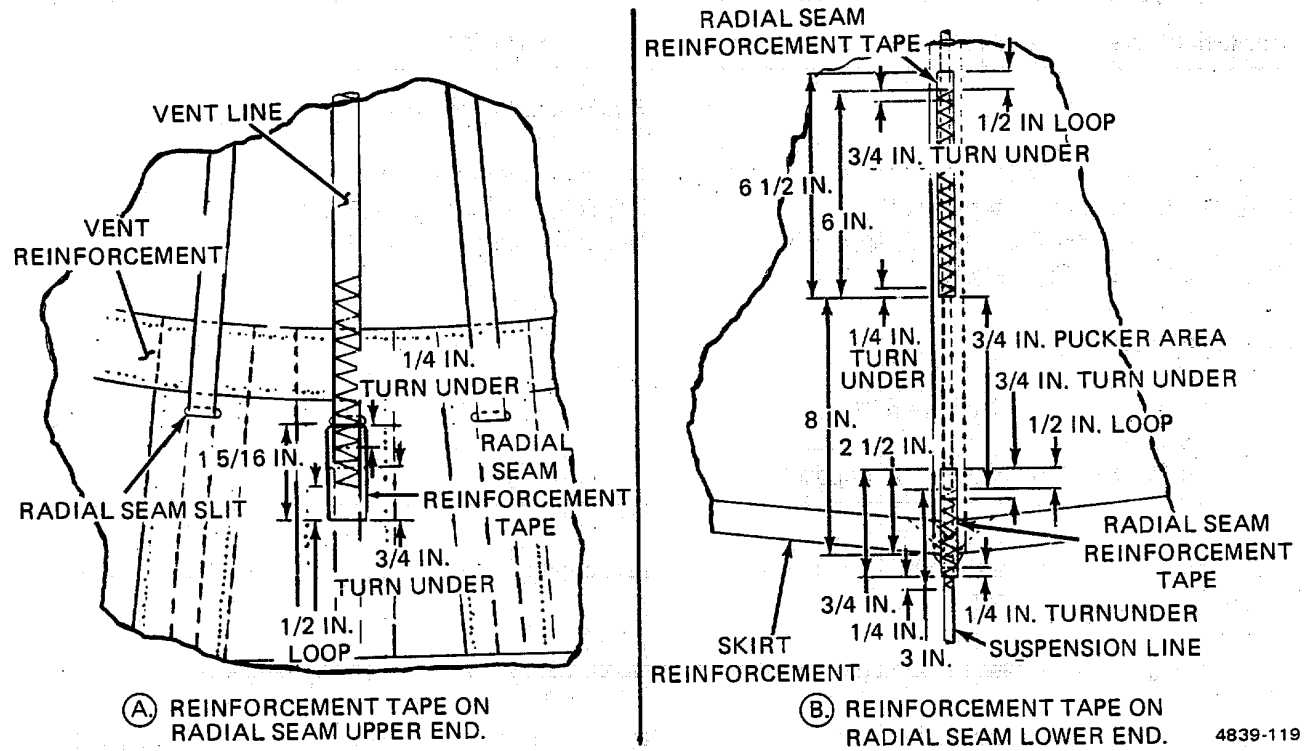
Figure 2-120. Radial Seam Reinforcement Tape Replacement Details.
