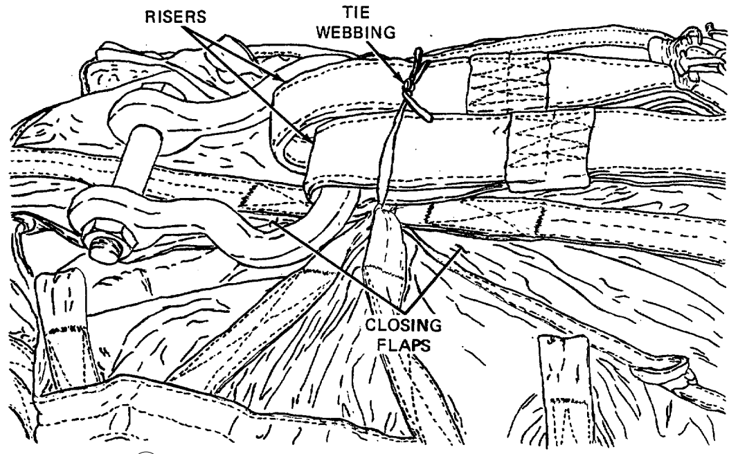
(B) SECURING RISERS ON TOP OF CLOSING FLAPS
