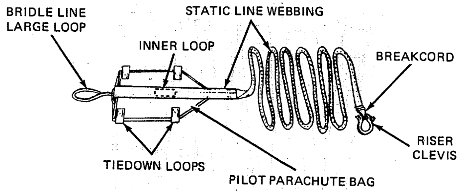
Figure 1-8. 68-Inch Diameter Pilot Parachute Static Line.
