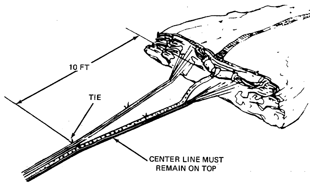
Figure 2-72. Tying Both Groups of Suspension Lines .
