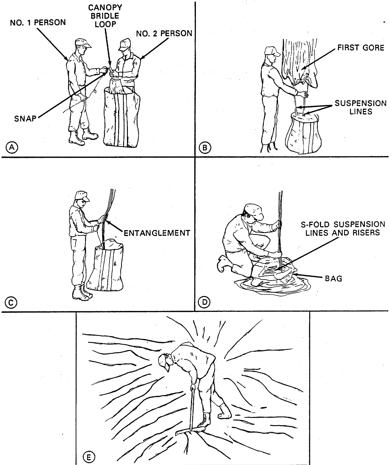
Figure 2-7. Shakeout.
