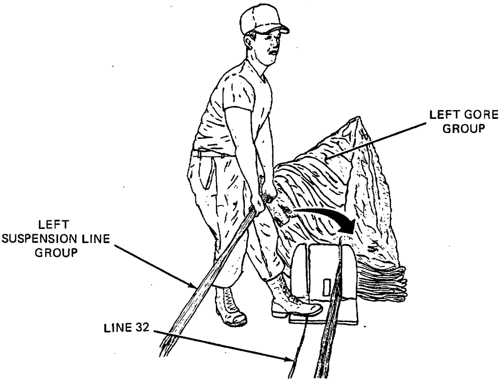
Figure 2-21. Preparing to Throw Left Group of Gore and Suspension Lines.
