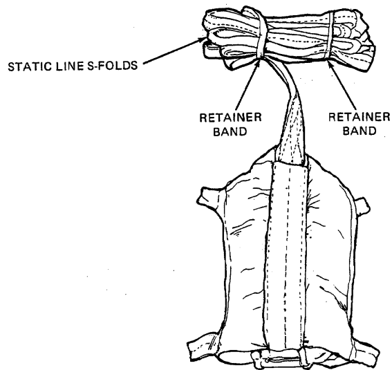
Figure 2-102. Packing Completed.
