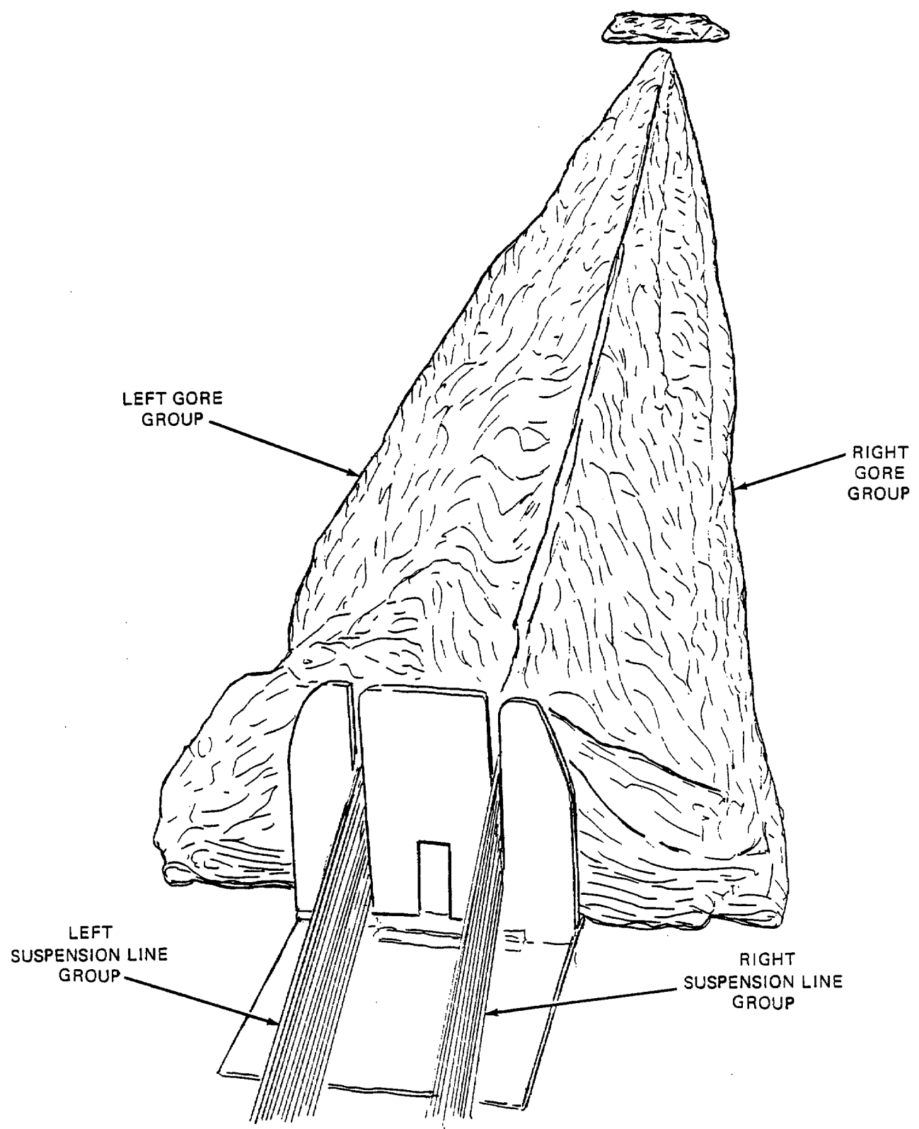
Figure 2-65. Gore Folding Completed .
