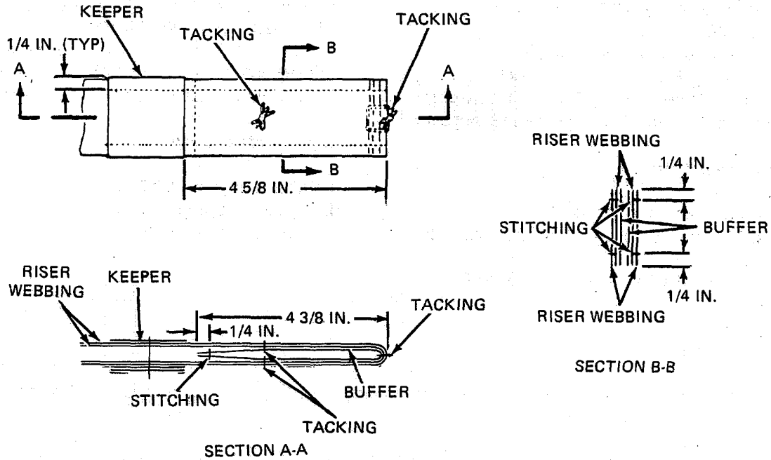
Figure 2-126. Clevis Attaching Loop Buffer Replacement Details.
