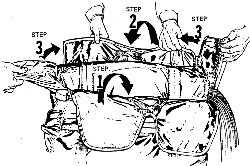
Figure 2-90. Folding Deployment Bag Closing Flaps.
