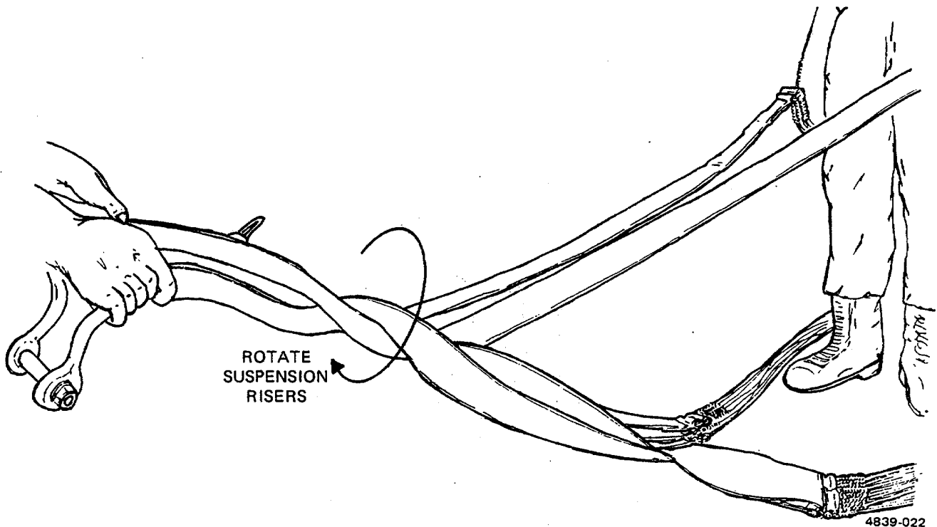
Figure 2-56. Removing Twists from Suspension Lines.
