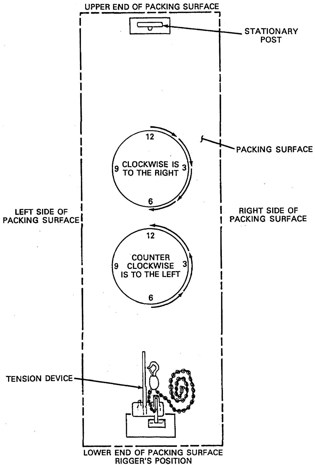
Figure 2-8. Rigger's Orientation.
