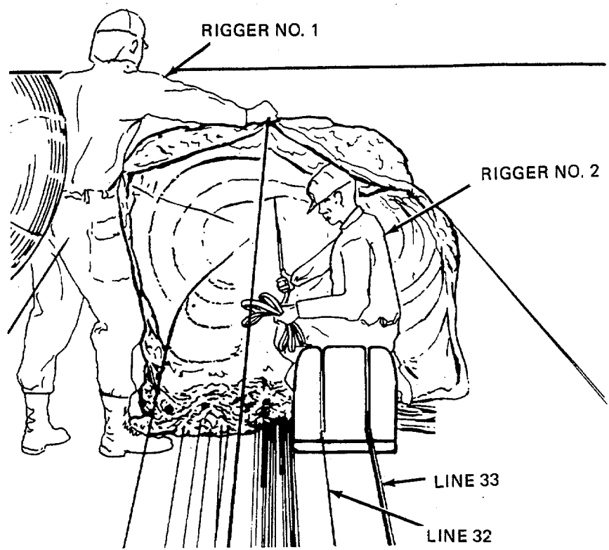
Figure 2-60. Placing the Center Line .
