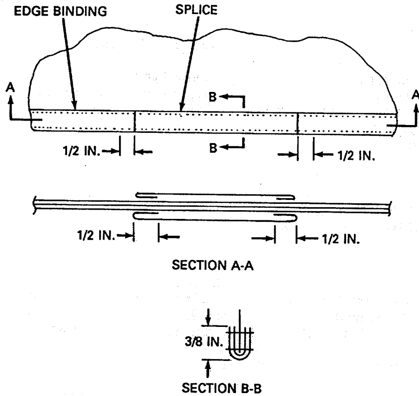
Figure 2-129. Deployment Bag Edge Binding Splicing Details.
