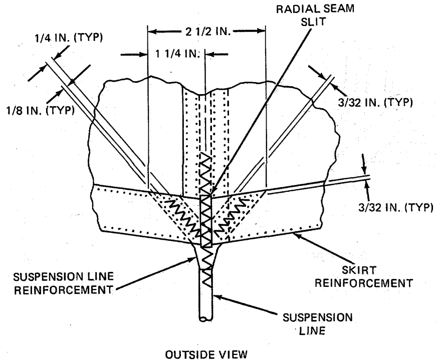
Figure 2-124. Suspension Line Reinforcement (V-Tab) Construction Details.
