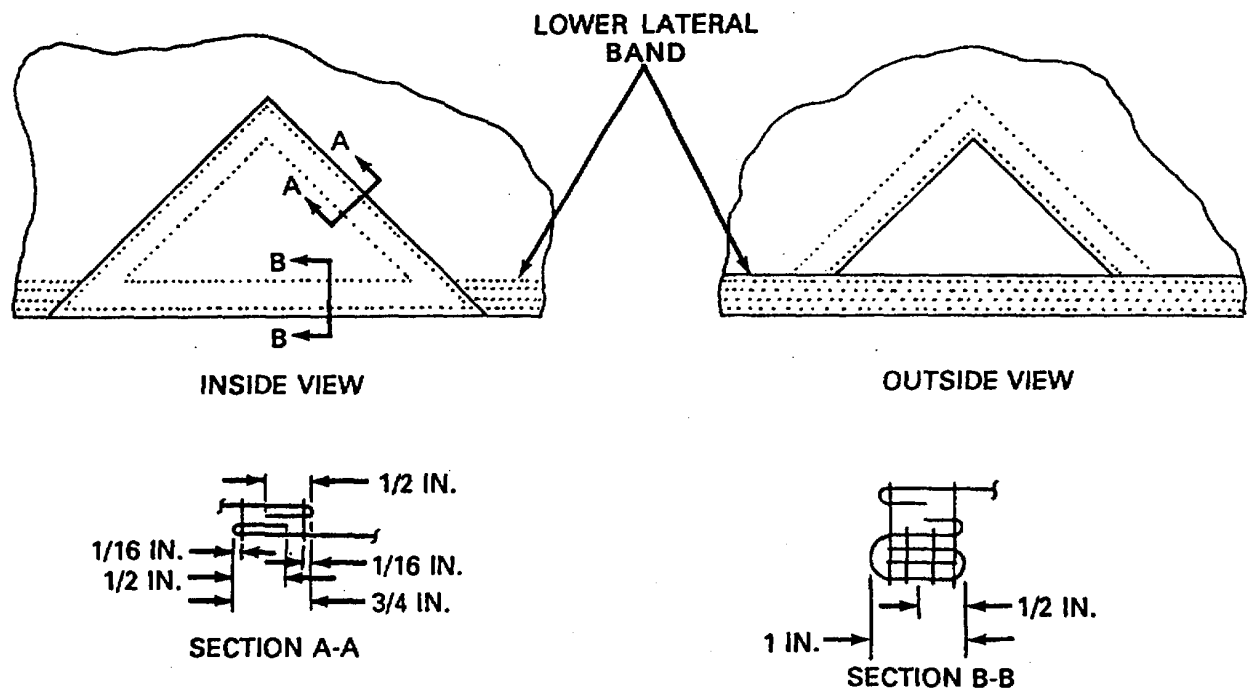
G TRIANGULAR PATCH INCLUDING LOWER LATERAL BAND.
