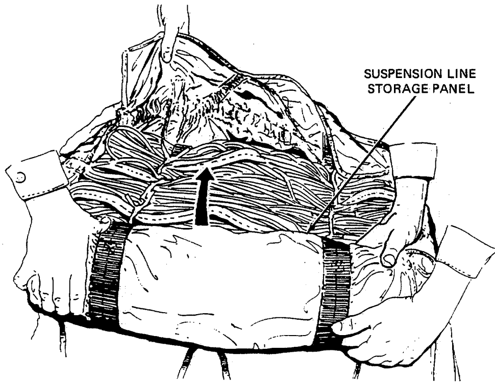
Figure 2-89. Rolling the Suspension Line Stowage Flap.
