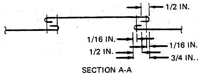
Figure 2-139. Basic Patch Application.
