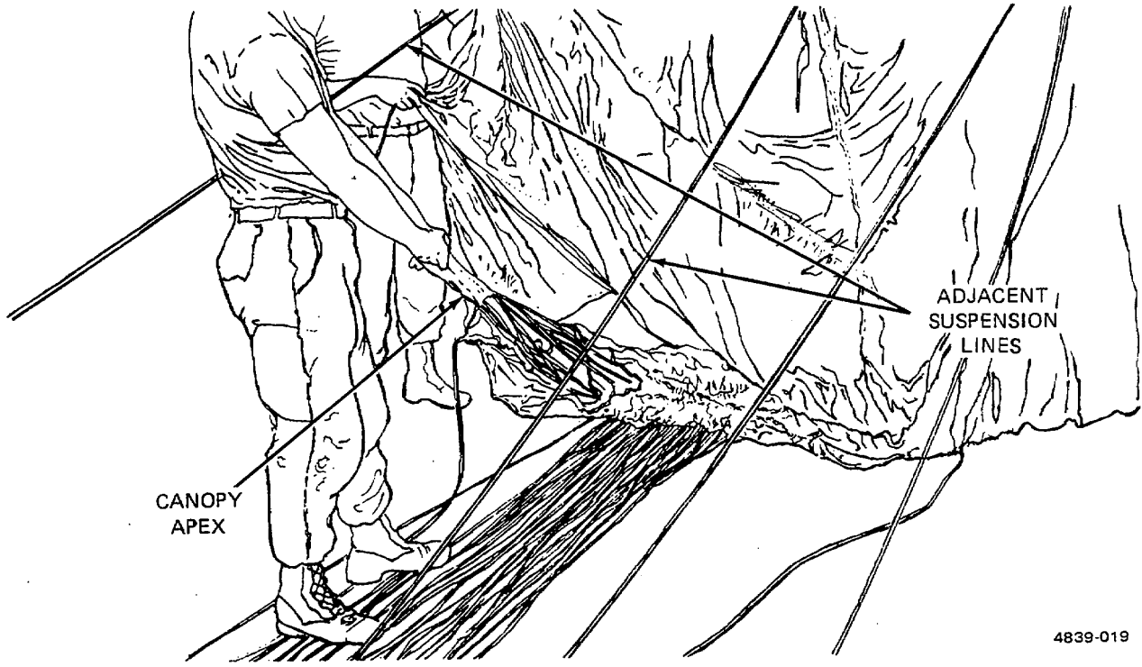
Figure 2-53. Removing Canopy Inversion.
