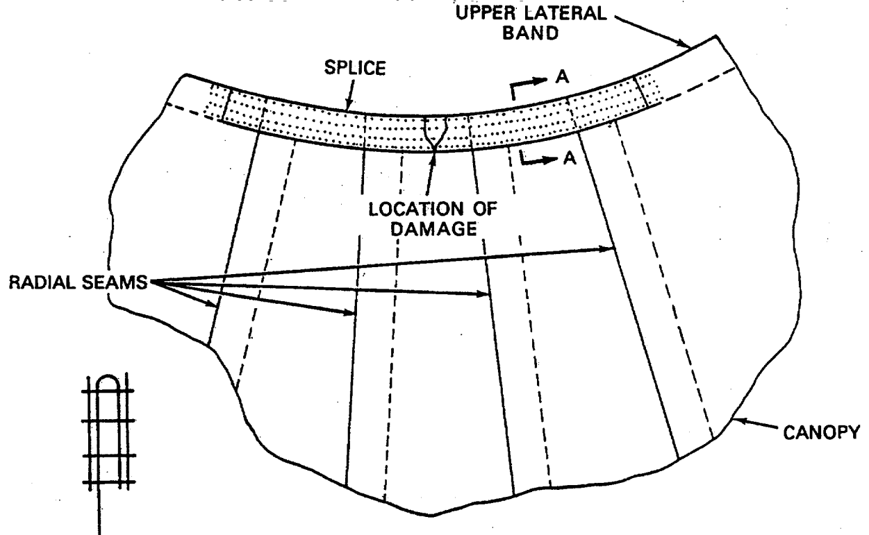
(A) DAMAGE BETWEEN RADIAL SEAMS
