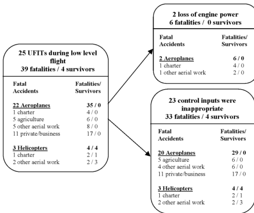
Figure 29: UFIT fatal accidents during low-level flight sorted by loss of control initiating event
