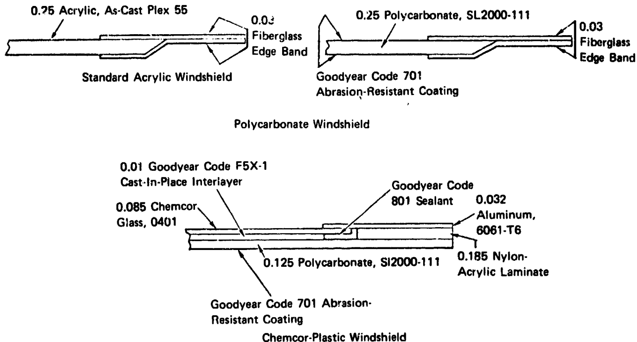
Figure 1. UH-1 windshield test configurations.
