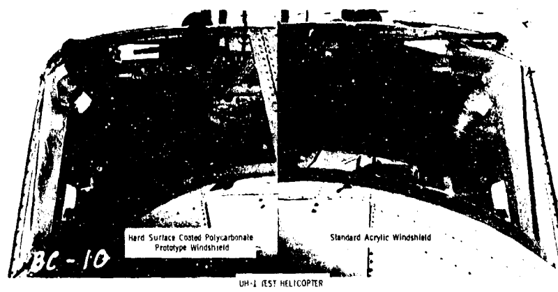
Figure 2. Windshields during flight testing - 385 flight hours. 19-066-141/AMC-74
