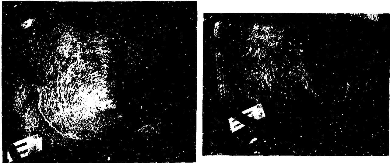
Figure 17. Bird-impacted UH-1 Chemcor-plastic windshields.
