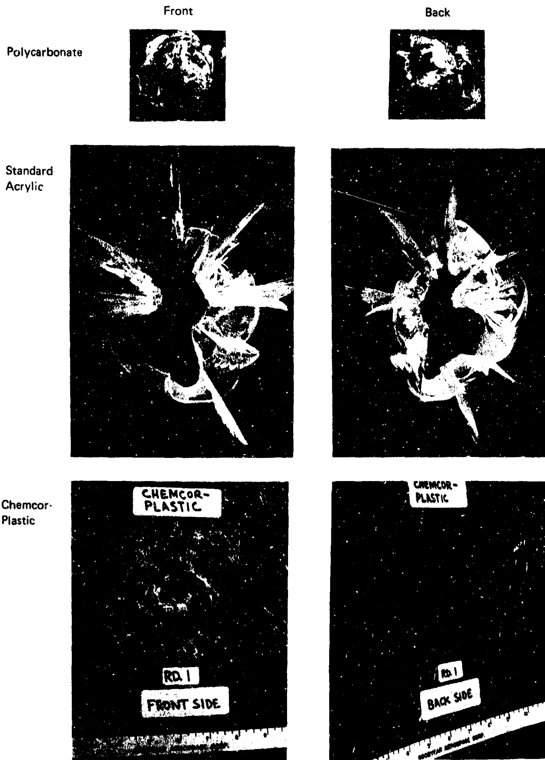
Figure 10. Ballistic penetration of UH-1 windshields, front- and back-side details.
