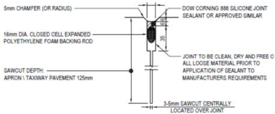
Detail of Chamfered Joint
