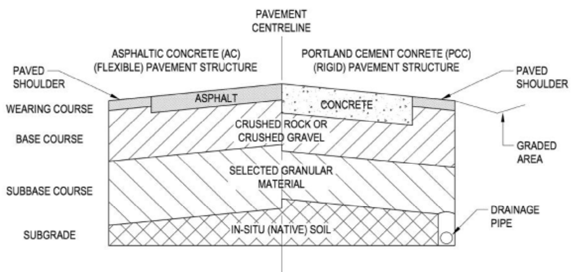
Cross Section of a Typical Pavement Construction
