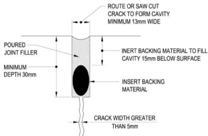
Typical Crack Repair Method
