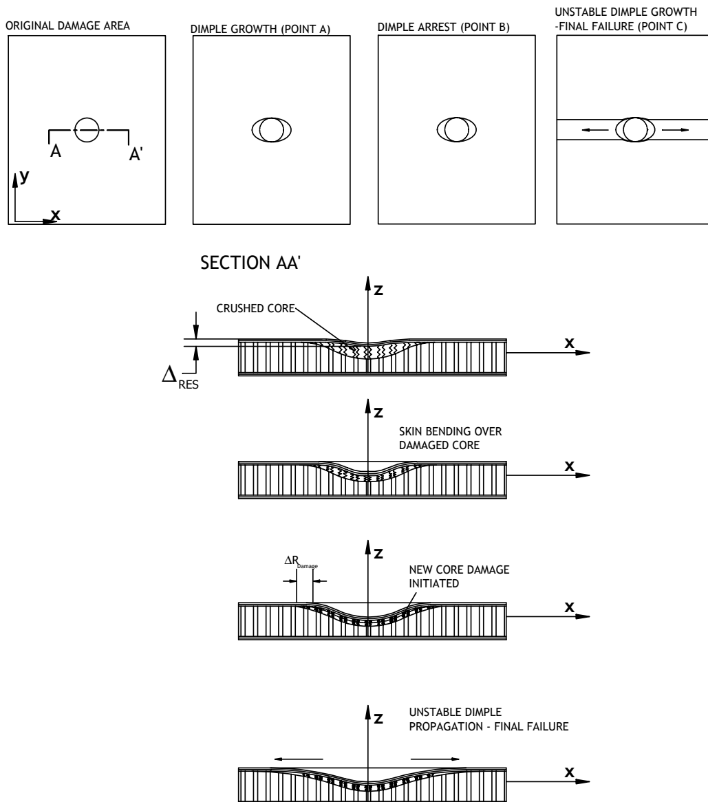
FIGURE 2-6. DAMAGE GROWTH MECHANISM AND FINAL FAILURE MODE OBSERVED IN [(90/45)_2/CORE]_s SANDWICH PANEL WITH HONEYCOMB CORE
