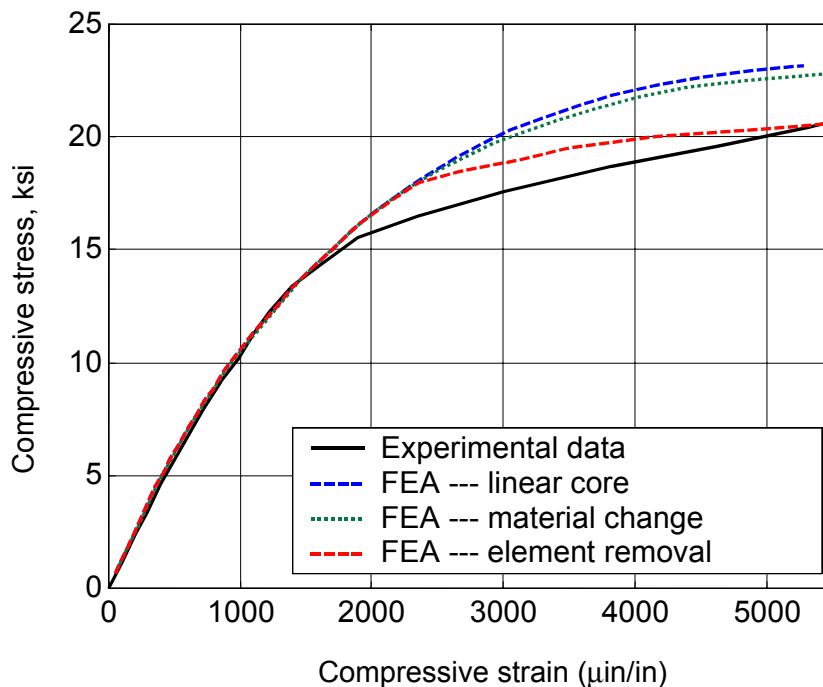
FIGURE 5-6. CORRELATION BETWEEN ANALYSIS WITH DIFFERENT CORE PROPERTIES AND EXPERIMENT
