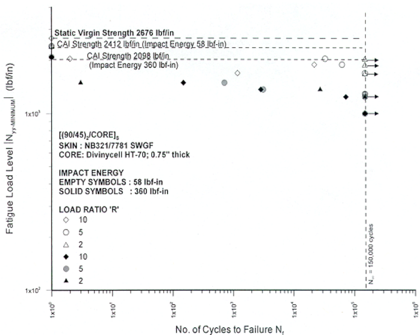
FIGURE 2-24. FATIGUE LIFE DATA FOR [(90/45) 2 /CORE] s SANDWICH PANELS WITH FOAM CORE
