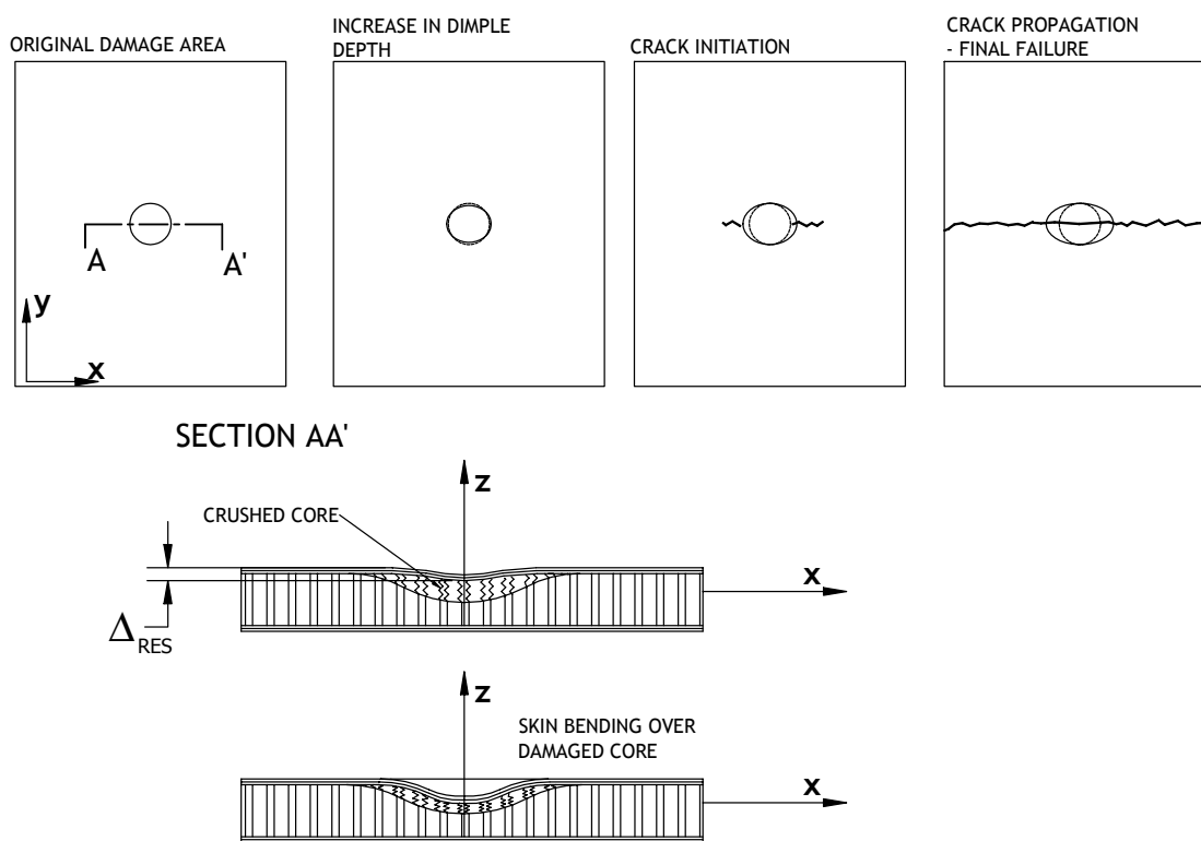
FIGURE 2-4. DAMAGE GROWTH MECHANISM AND FINAL FAILURE MODE OBSERVED IN [(90/45)/CORE]_s SANDWICH PANEL WITH HONEYCOMB CORE (SHARP IMPACTOR)
