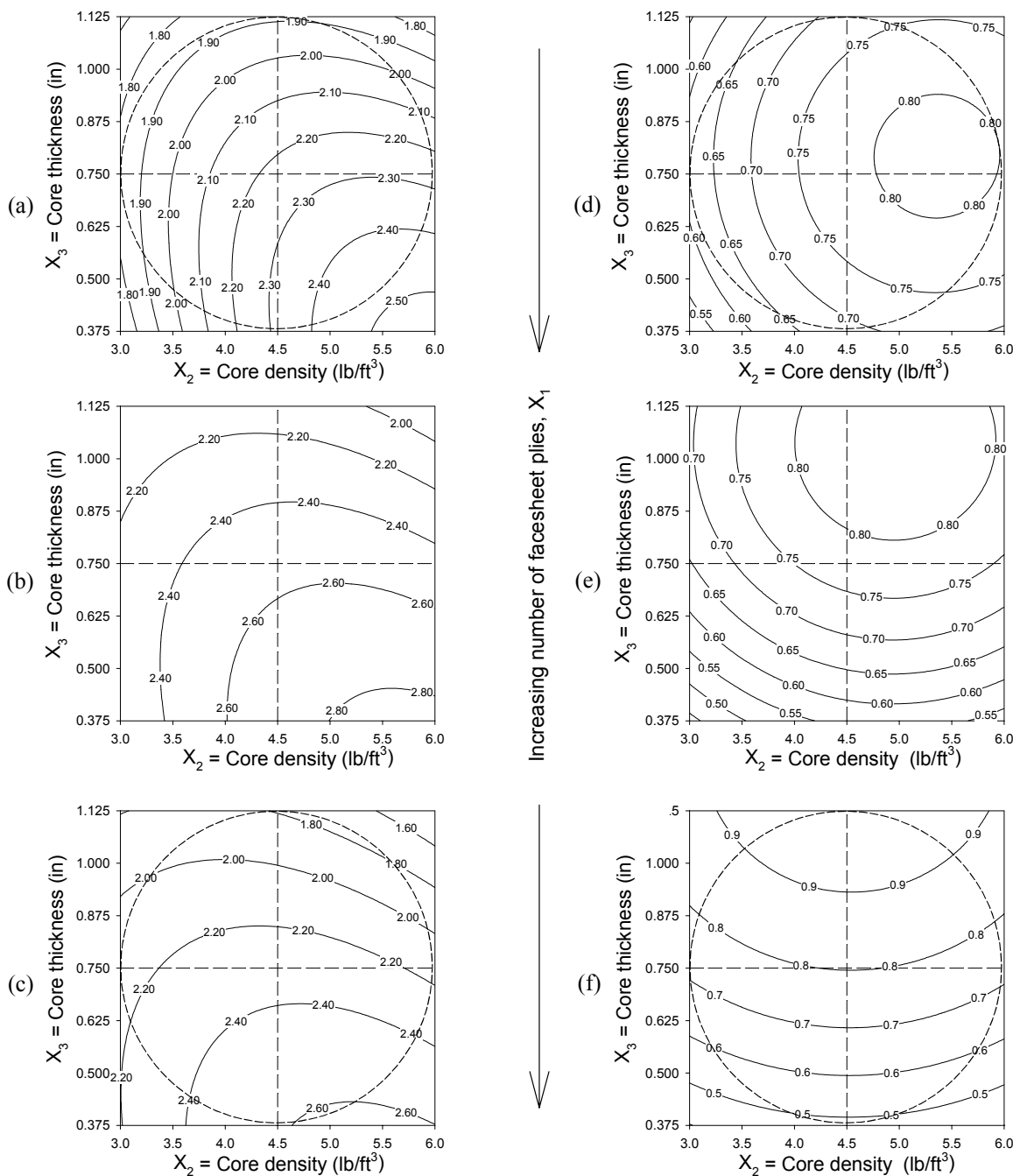
FIGURE 3-3. PREDICTED DAMAGE DIAMETER (in.) FOR X_1 = (a) 2, (b) 4, AND (c) 6 PLYS [13]. PREDICTED NORMALIZED RESIDUAL STRENGTH FOR X_1 = (d) 2, (e) 4, AND (f) 6 PLYS.
