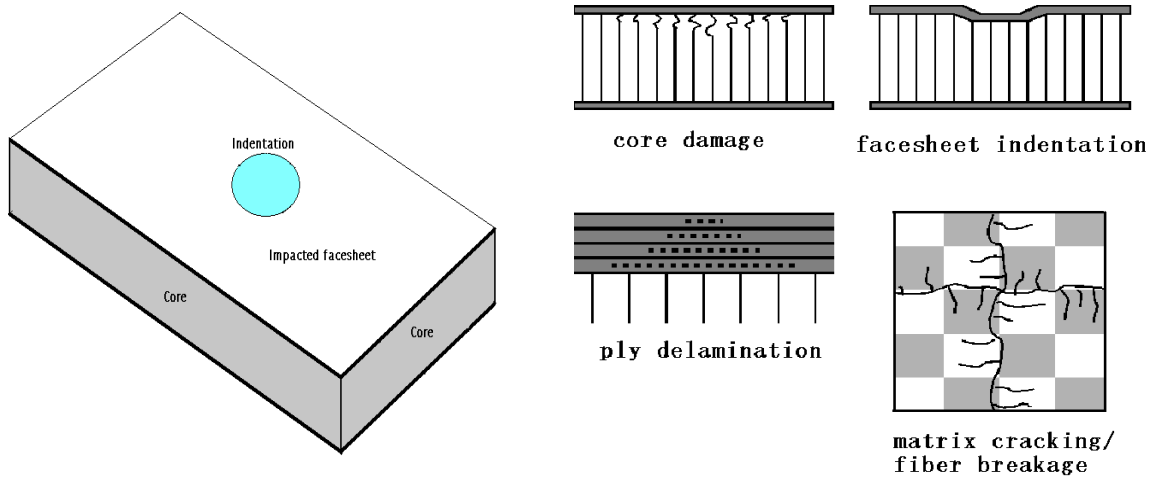
FIGURE 5-1. COMPOSITE SANDWICH PANEL WITH LOW-VELOCITY IMPACT DAMAGE
