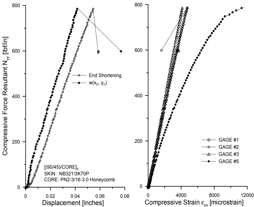
FIGURE 2-3. CAI TEST DATA FOR [(90/45)/CORE]_s SANDWICH PANEL WITH PLAIN-WEAVE CARBON FACESHEETS
