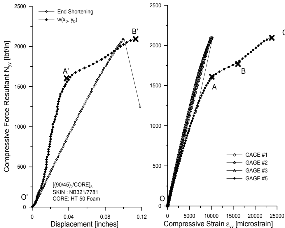
FIGURE 2-7. CAI TEST DATA FOR [(90/45)_2/CORE]_s SANDWICH PANEL WITH GLASS FABRIC FACESHEETS AND FOAM CORE
