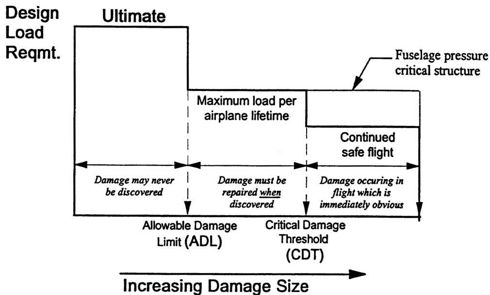
FIGURE 1-1. DAMAGE-TOLERANT DESIGN PHILOSOPHY
