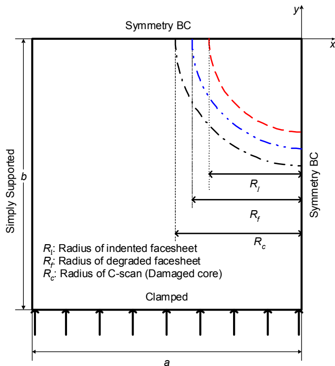
FIGURE 5-2. PLAN VIEW SCHEMATIC OF FINITE ELEMENT MODEL
