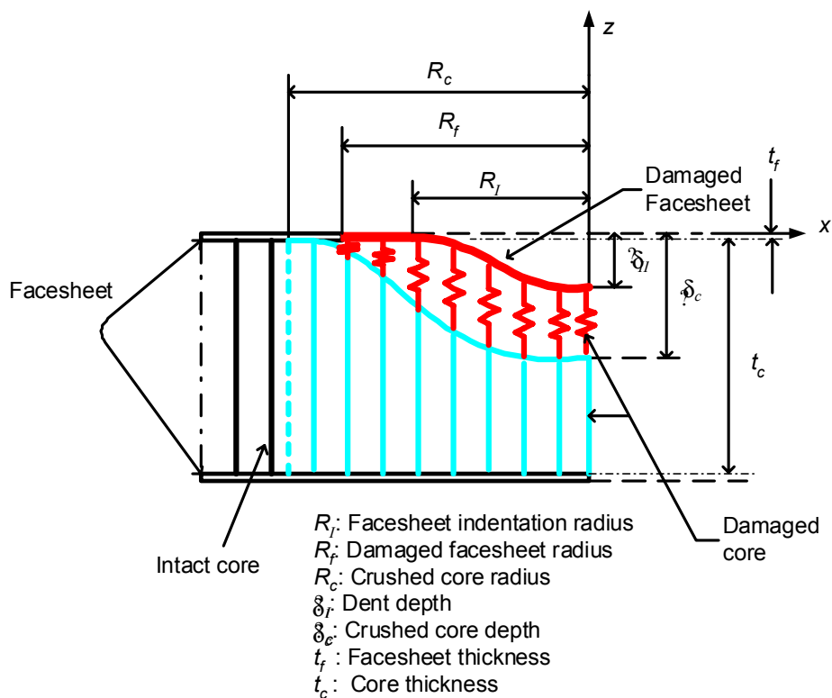
FIGURE 5-3. IMPACT-DAMAGED REGION
