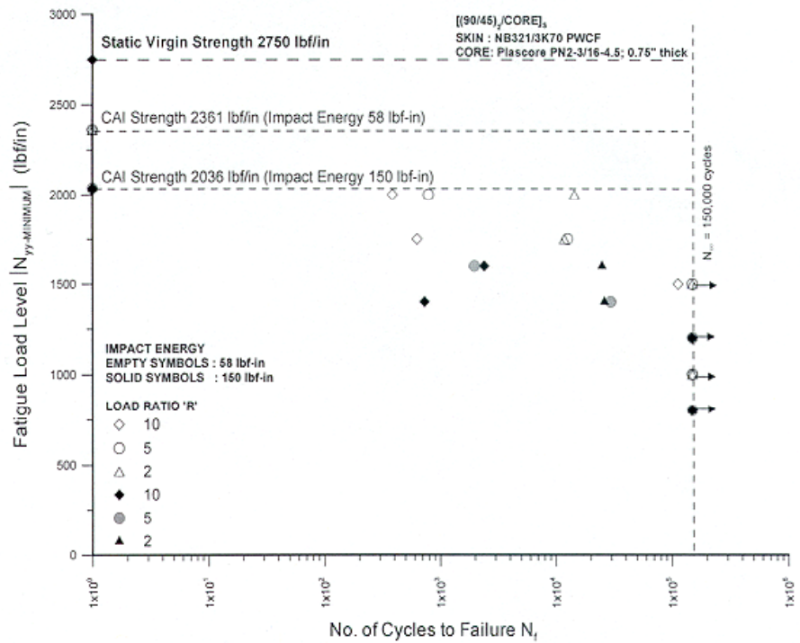
FIGURE 2-22. FATIGUE LIFE DATA FOR [(90/45) 2 /CORE] s SANDWICH PANELS WITH HONEYCOMB CORE
