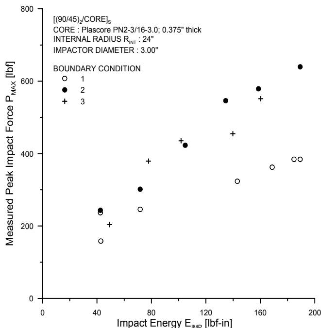
FIGURE 2-17. PEAK IMPACT FORCE AT VARIOUS ENERGY LEVELS FOR [(90/45) 2 /CORE] s SPECIMENS WITH DIFFERENT BOUNDARY CONDITIONS
