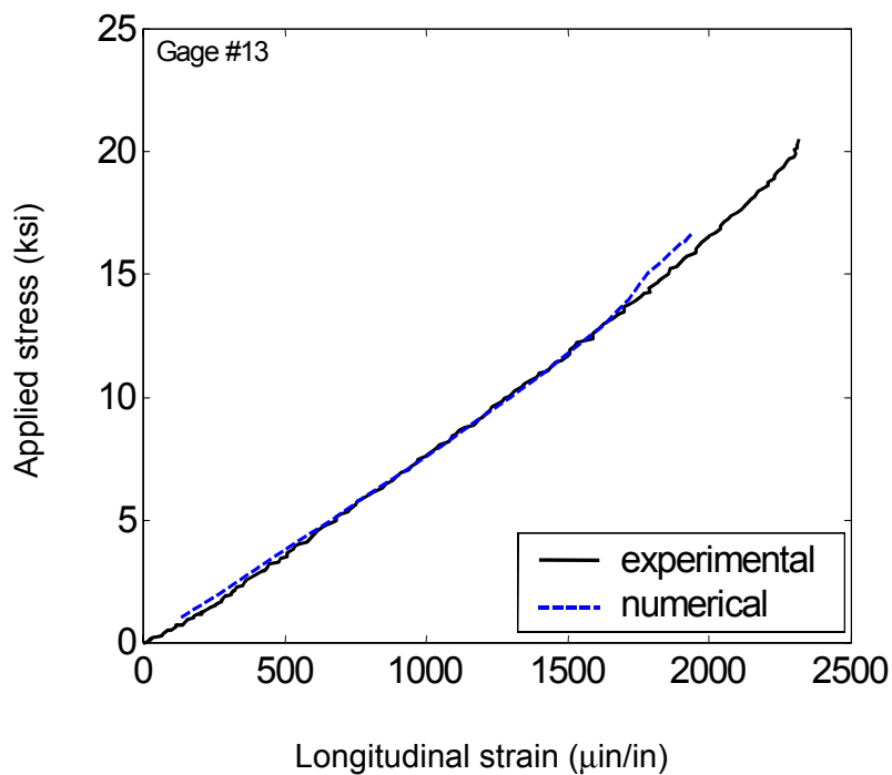
FIGURE 5-21. COMPARISON OF STRAINS AT GAGE NO. 13
