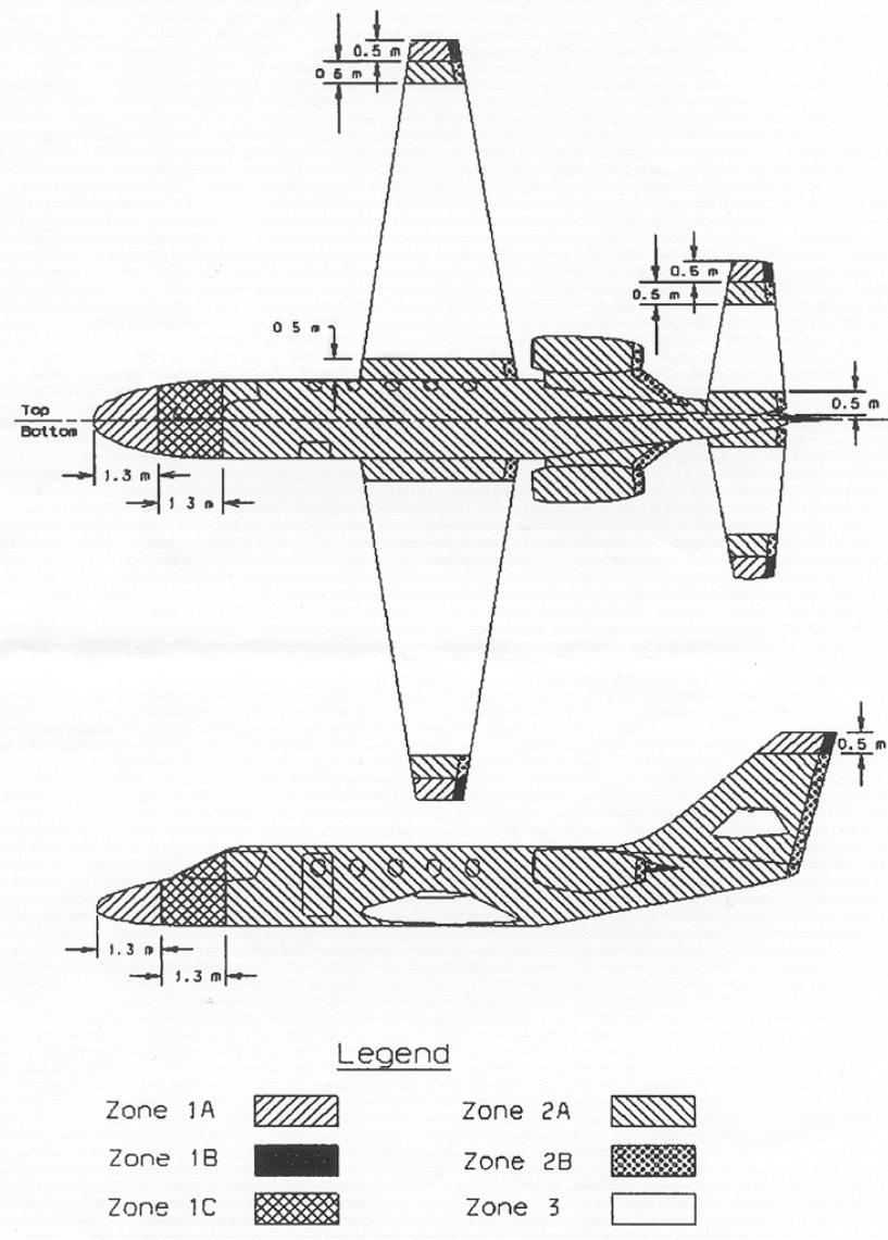
FIGURE C-1. LIGHTNING STRIKE ZONE DETAILS FOR STRAIGHT-WING BUSINESS JET AIRCRAFT
