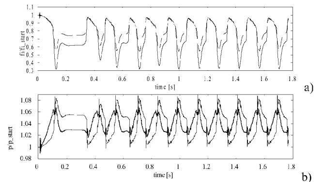
Fig.6: Compression system instability. a) flow coefficient, b) static pressure
