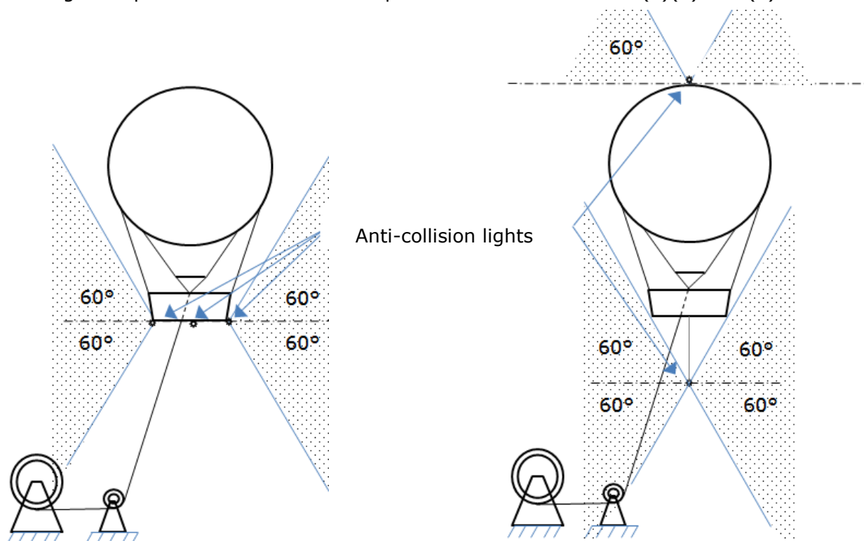
Option 2 Anti-collision light on top of the envelope and a complementary light suspended below the gondola
