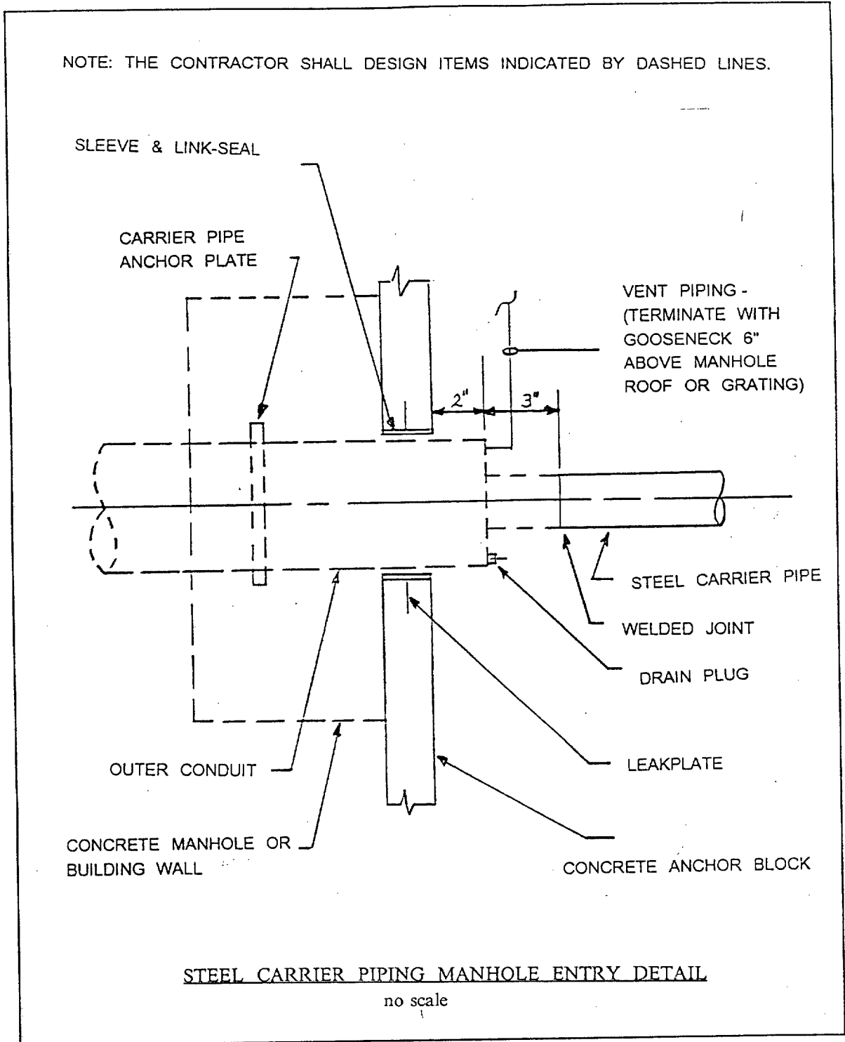
Figure 24 Steel Carrier Piping Manhole Entry Detail (no scale)
