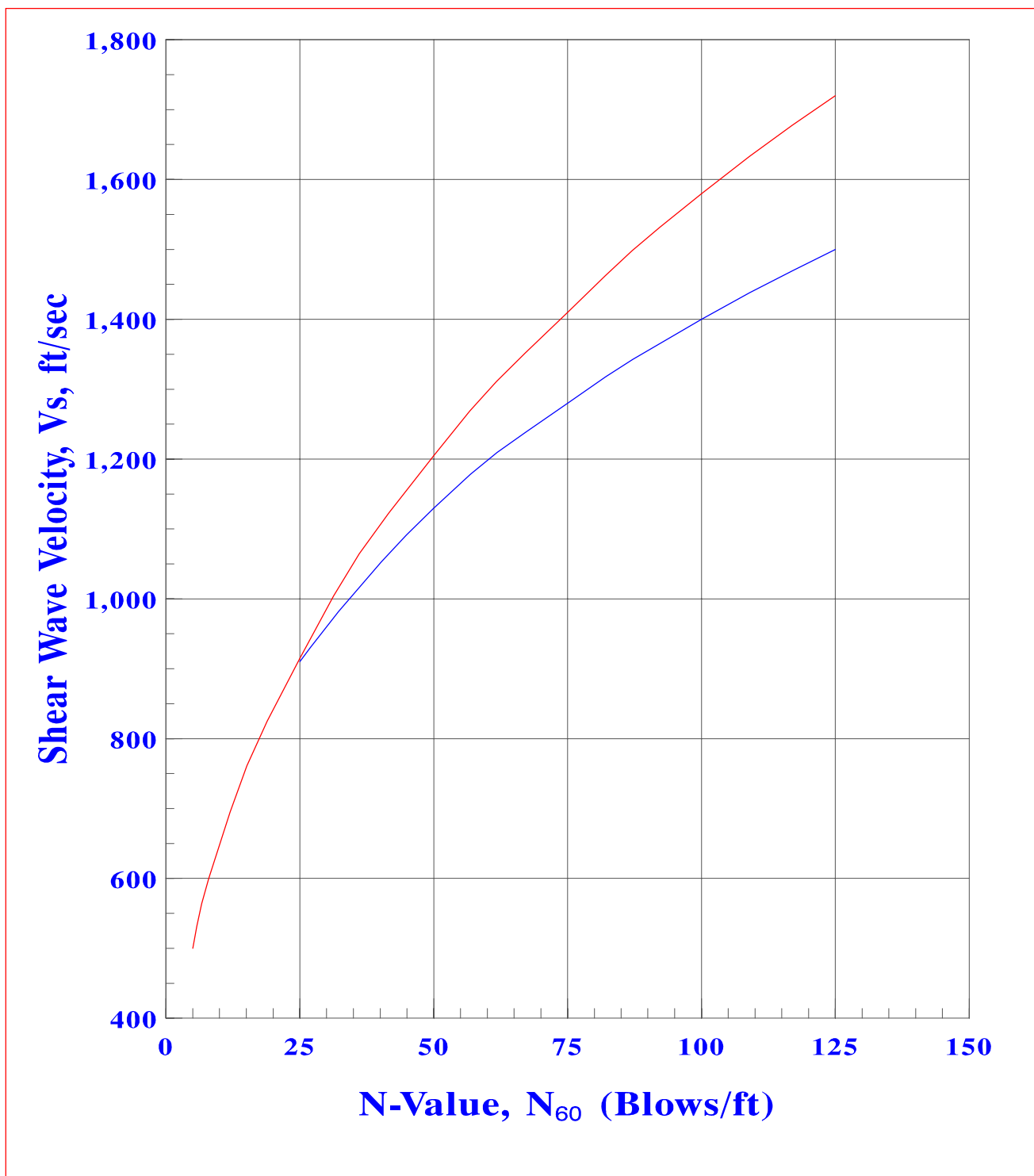
Figure 2 Relation Between Number of Blows Per Foot in Standard Penetration Test and Velocity of Shear Waves
