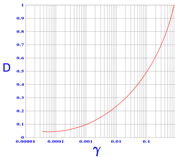
(B-2) Cyclic Shear Strain vs. the Value of Initial Damping Ratio
