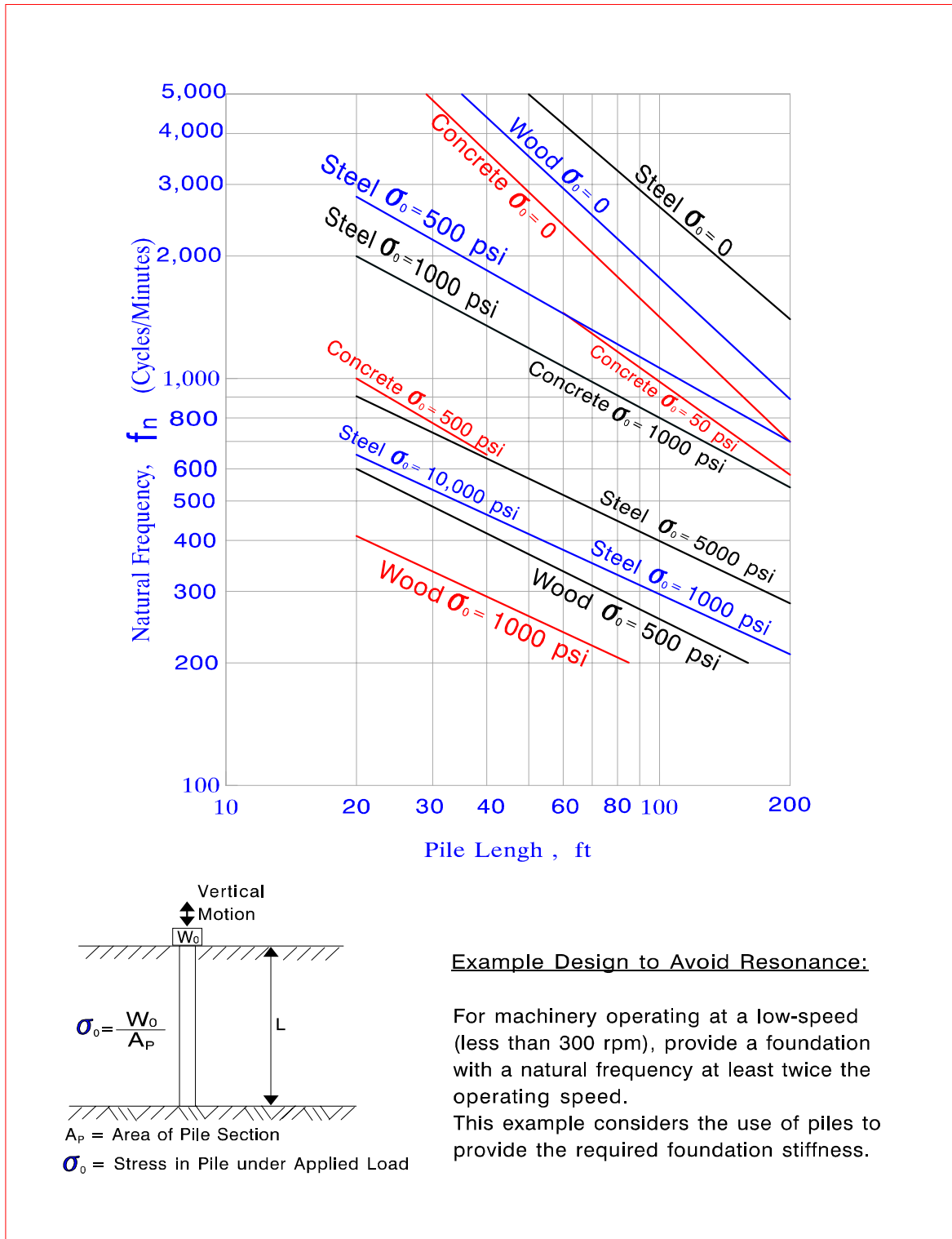
Figure 9 Natural Undamped Frequency of Point Bearing Piles on Rigid Rock
