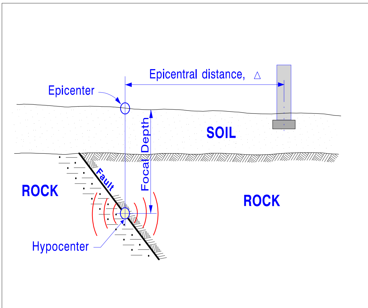
Figure 17 Definition of Earthquake Terms
