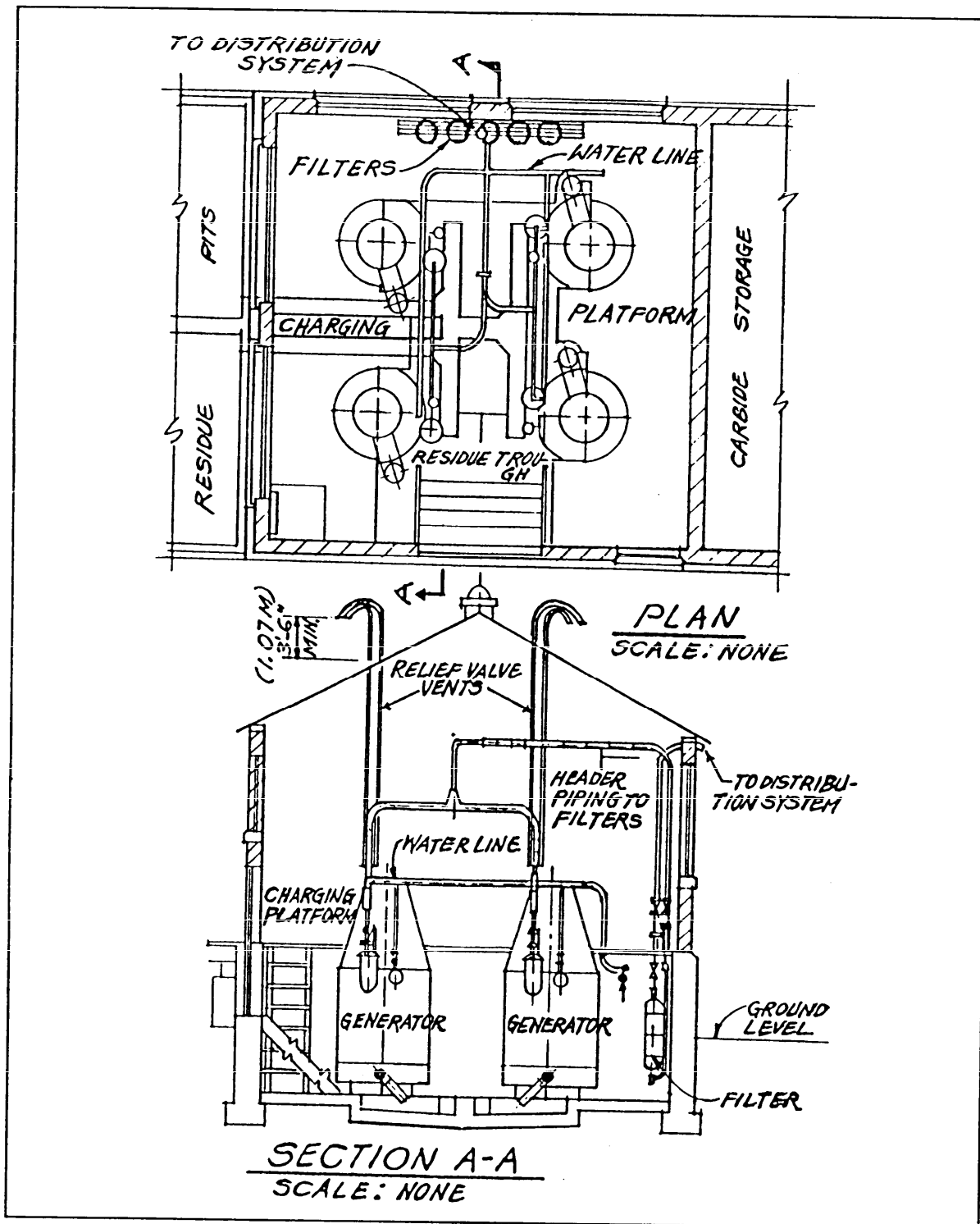
FIGURE 1 Medium Pressure Acetylene Generator Installation
