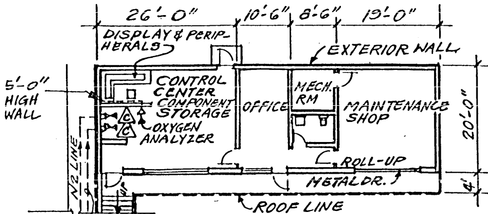
PARTIAL FLOOR PLAN
