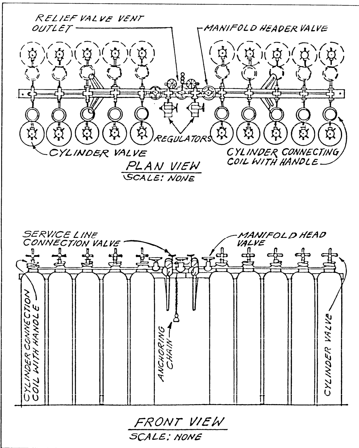
FIGURE 3 Ten-Cylinder Duplex Unit Type Oxygen Manifold
