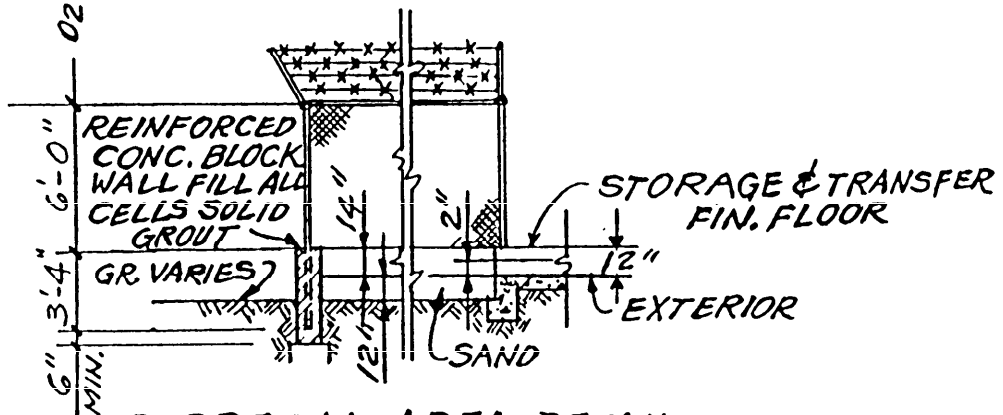
DISPOSAL AREA DETAIL
