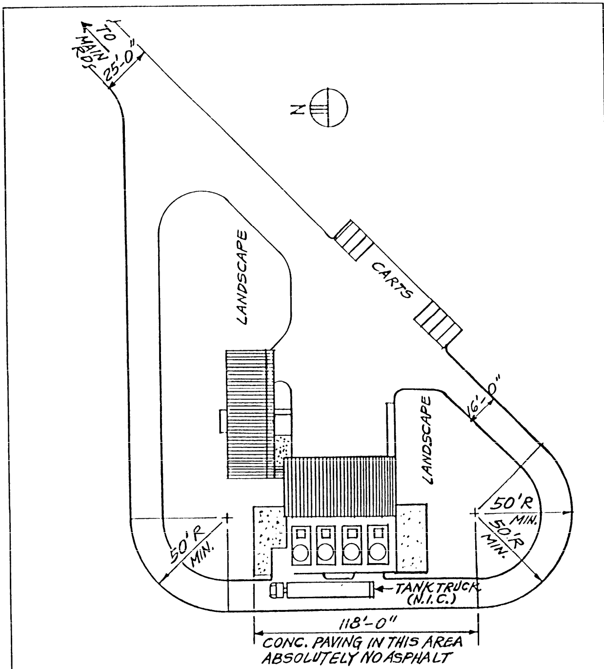
PLOT PLAN SCALE: NONE
