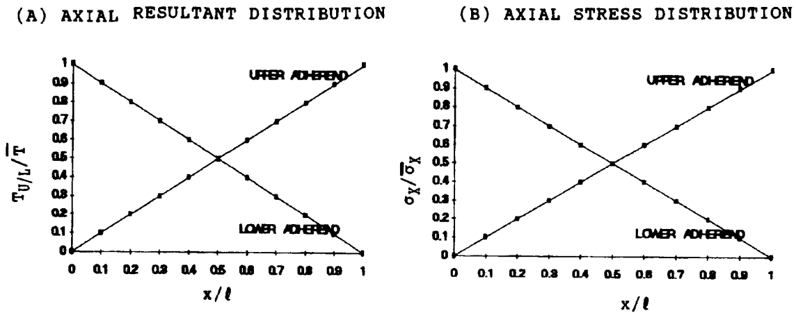
FIGURE 6.2.3.2(b) Axial stresses in joint with rigid adherends.
