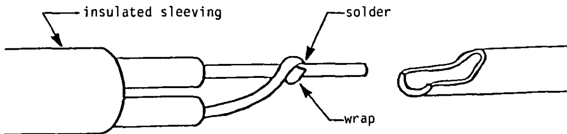
FIGURE 29. Offset method.
