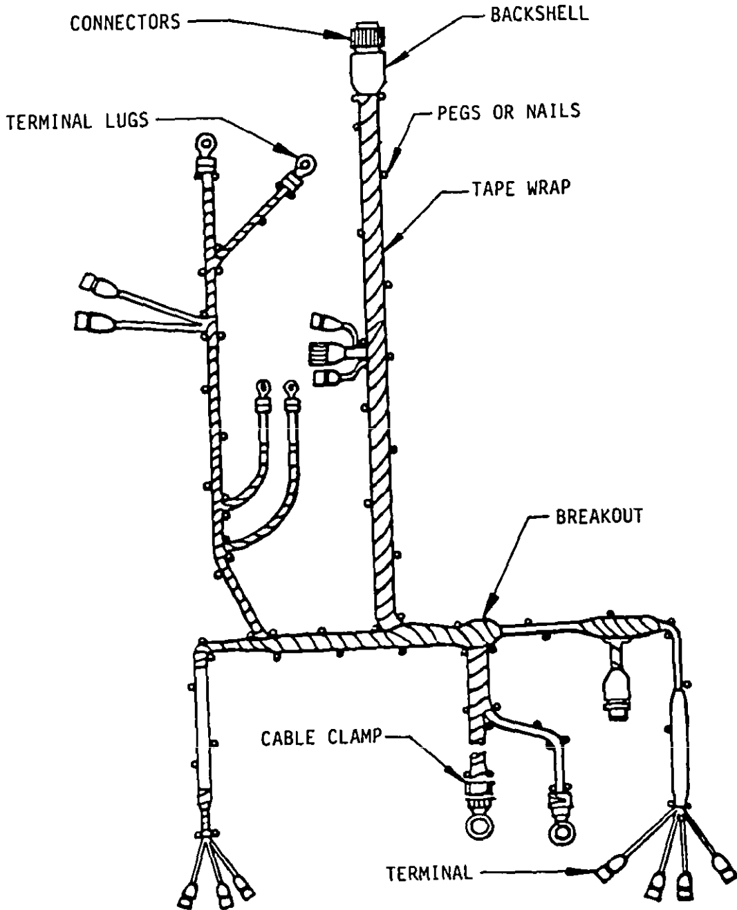
FIGURE 2. Wiring harness.
