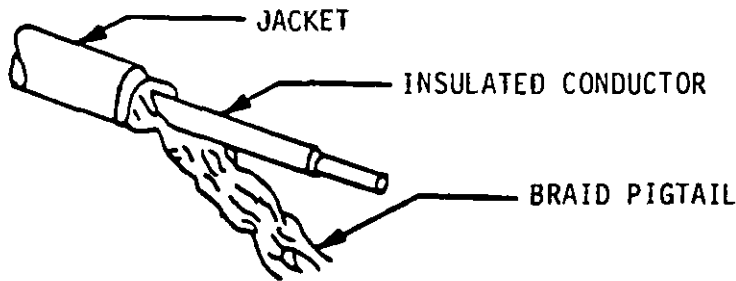
FIGURE 18. Pigtailed braid.
