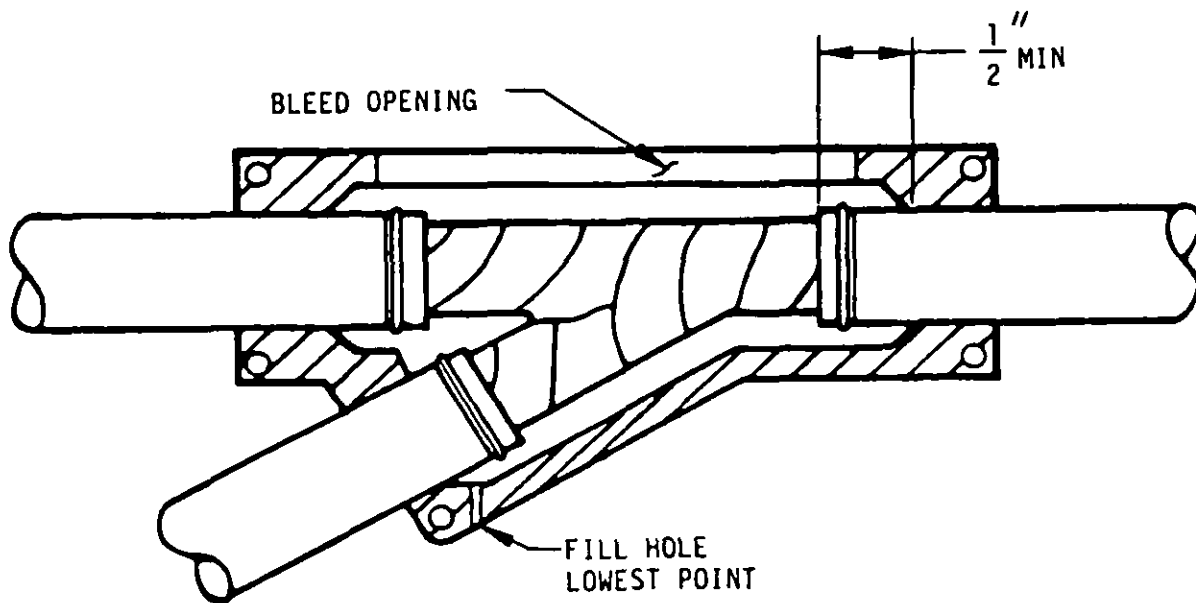
LOADING MOLD
