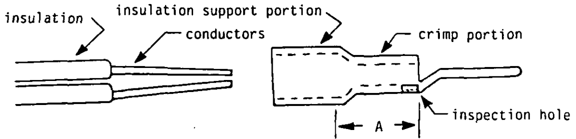
FIGURE 20. First two-conductor method using typical terminal.
