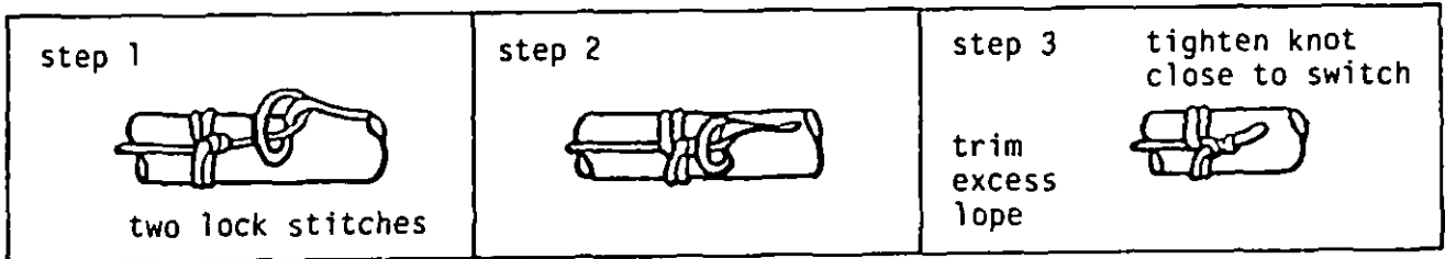
FIGURE 24. Finishing tie .
