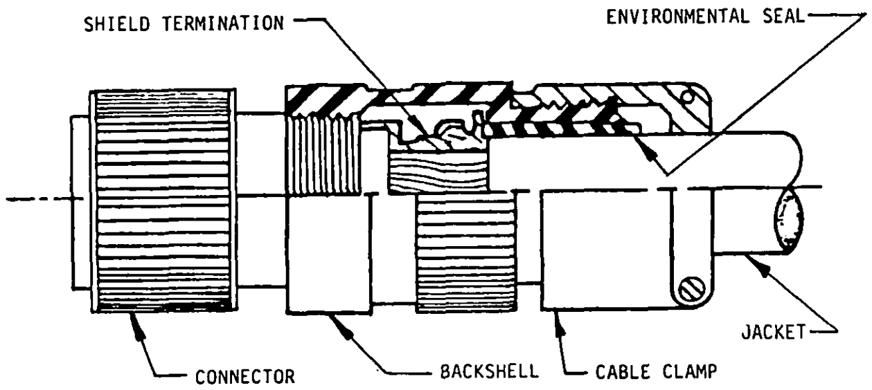
STANDARD BACKSHELL
