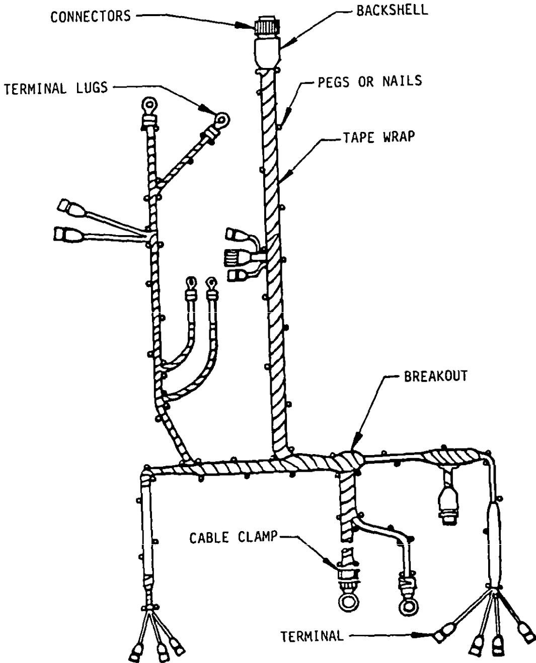
FIGURE 2. Wiring harness.
