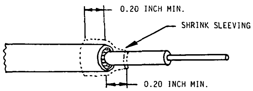
FIGURE 13. Floating shield .
