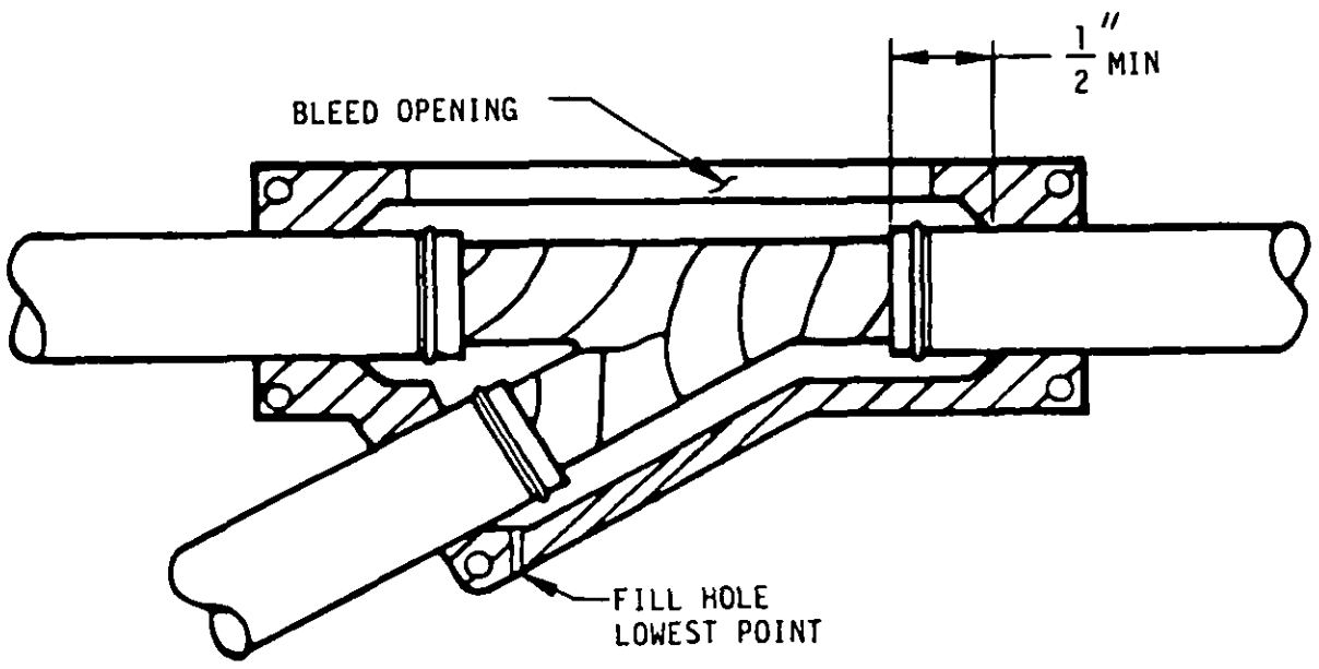
LOADING MOLD
