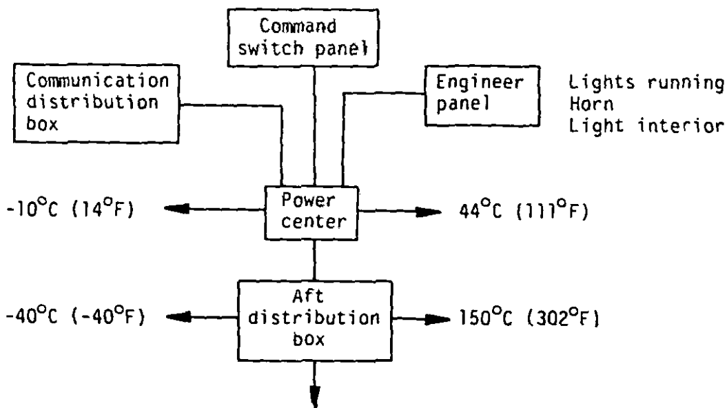
FIGURE 1. Functional wire block diagram.
