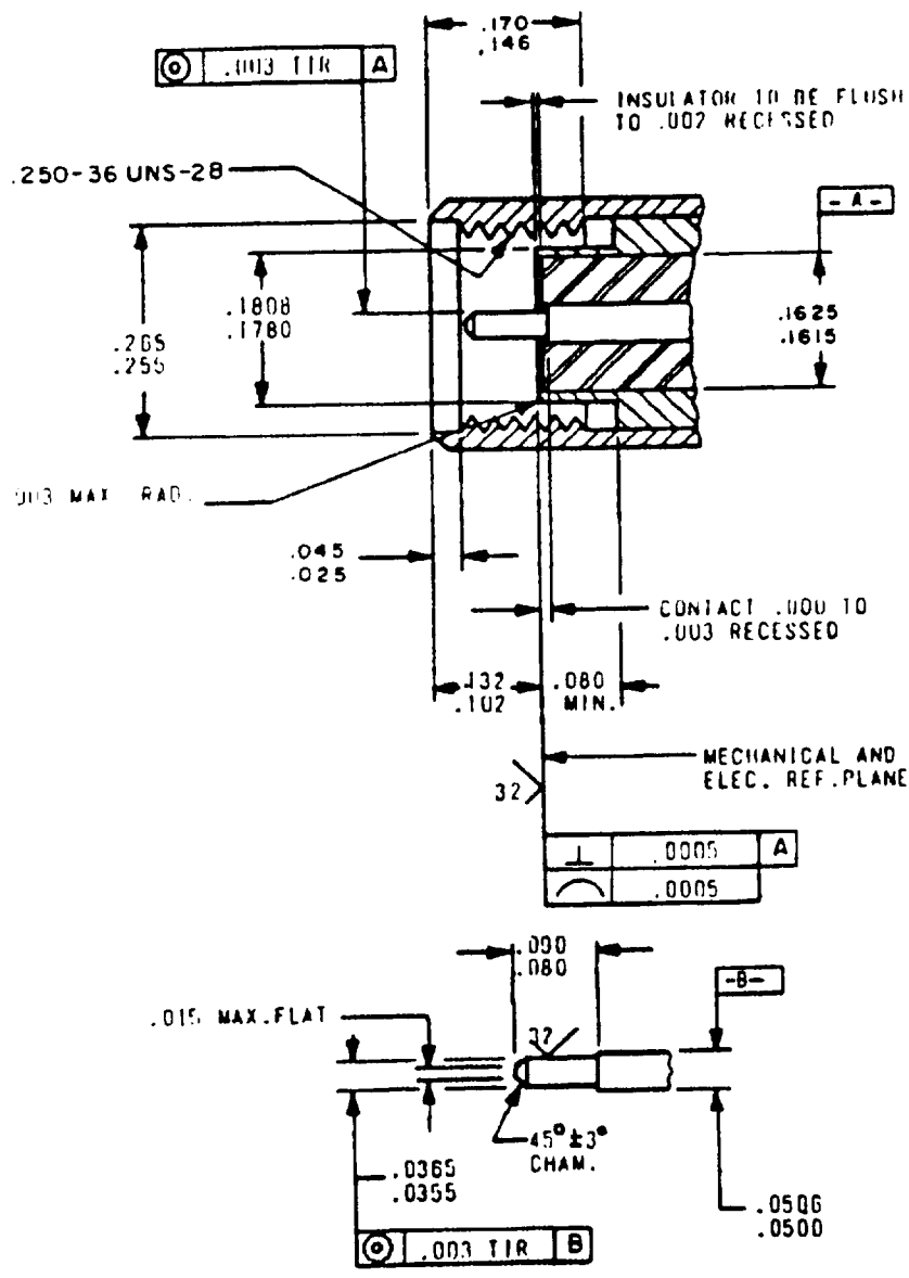
DETAIL OF INNER CONTACT
