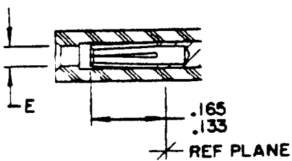
ALTERNATE CLOSED ENTRY INSULATOR DETAIL A
