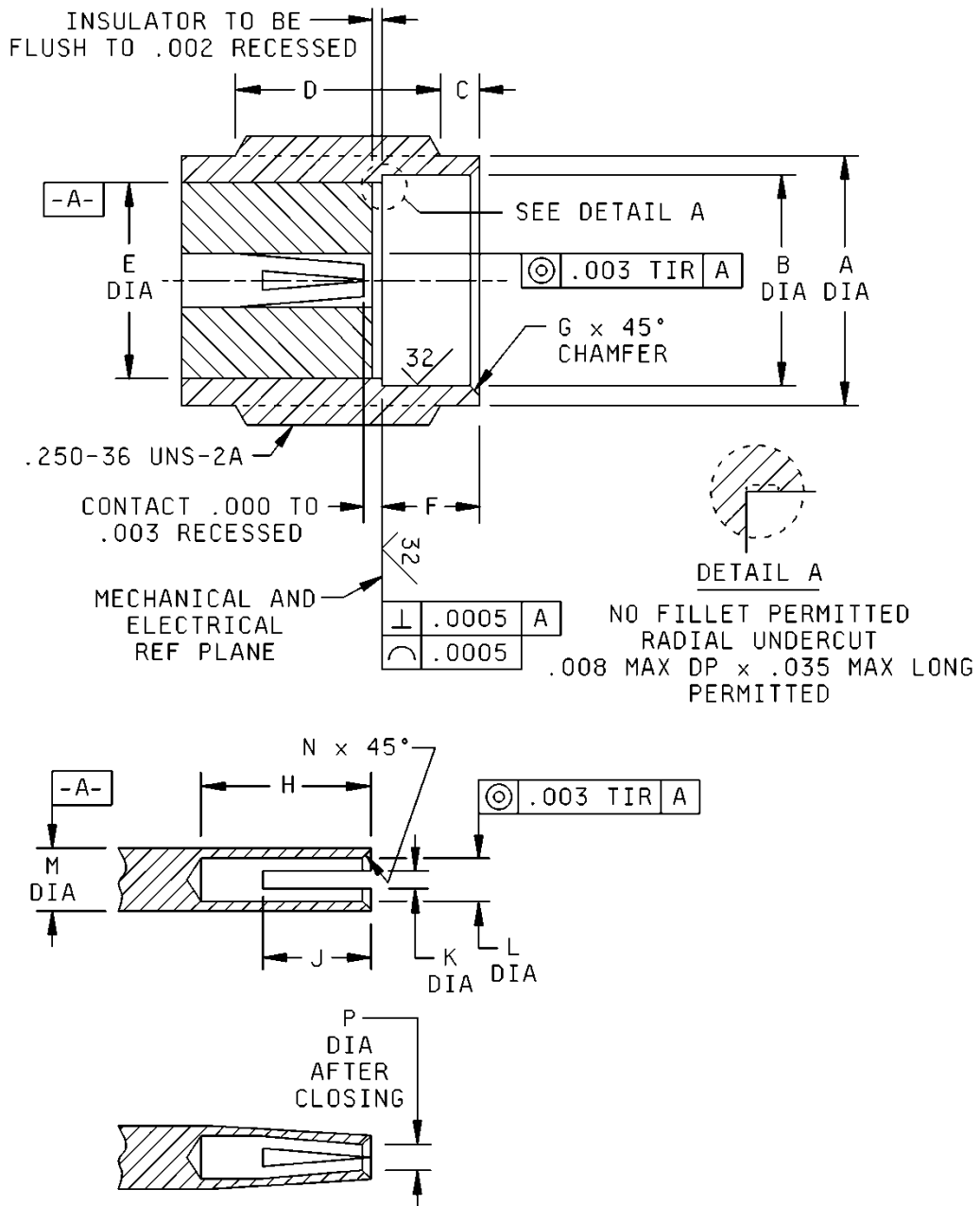
DETAIL OF INNER CONTACT
