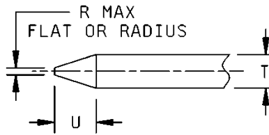
CENTER CONDUCTOR DETAIL A
