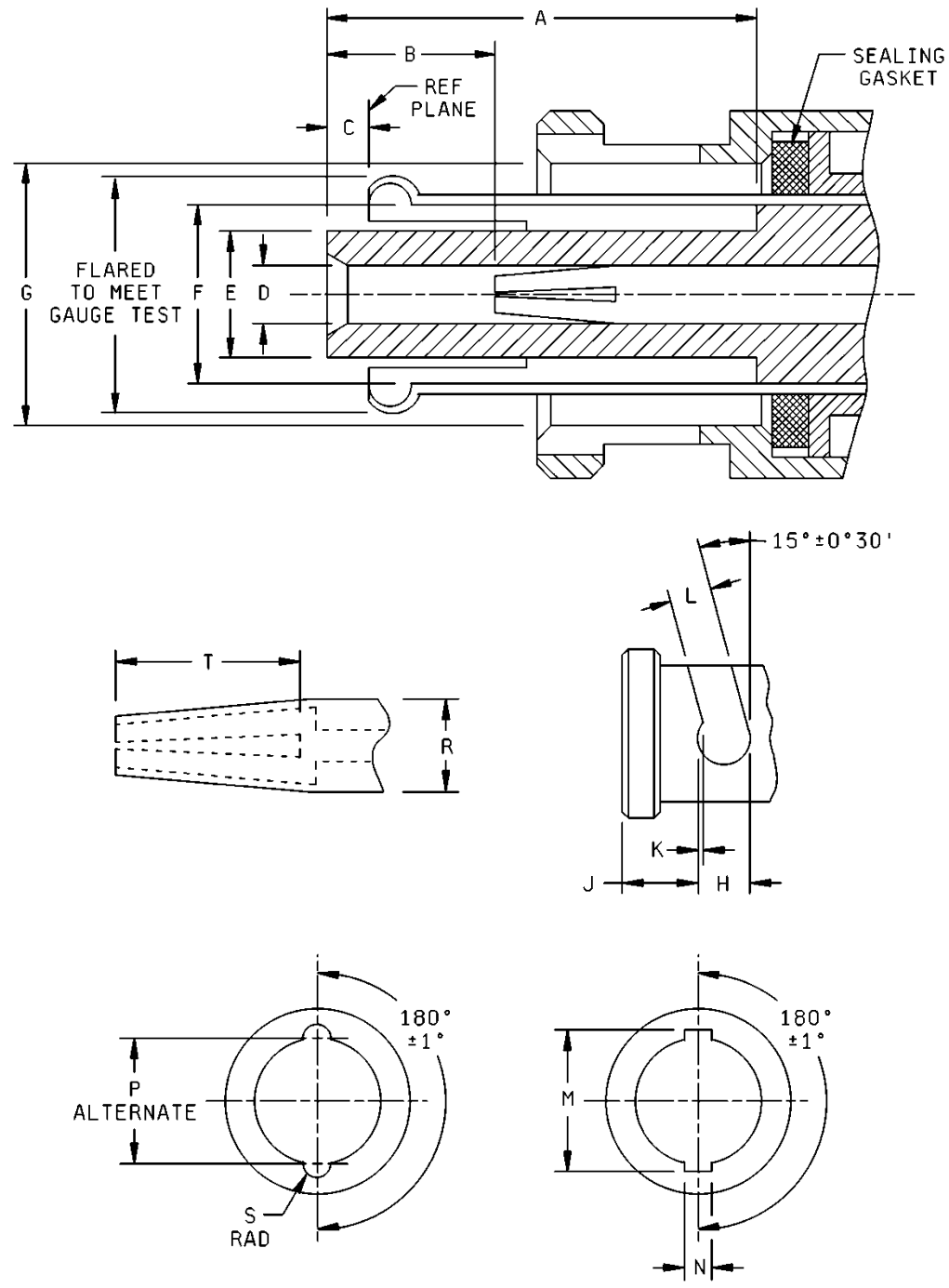
FIGURE 314-2. Interface, series SHV, socket contact.
