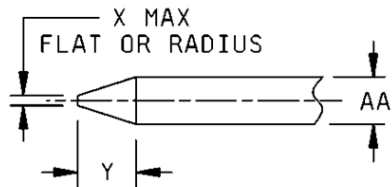
CENTER CONDUCTOR DETAIL A
