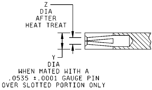
FIGURE 406-2. Interface, test connector, series TNC, socket contact.
