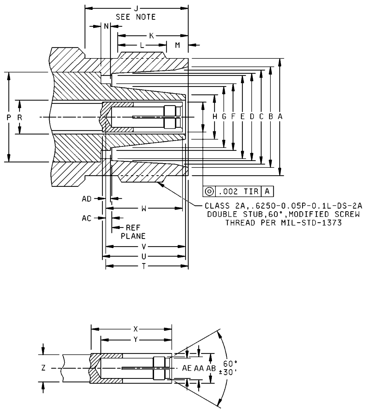
FIGURE 410-2. Interface, test connector, series QSC, socket contact.
