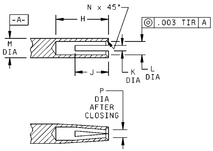
DETAIL OF INNER CONTACT
