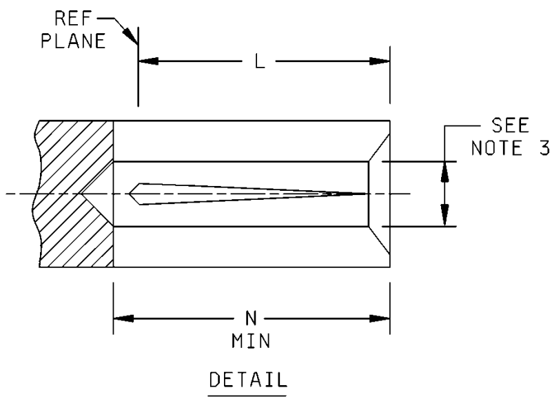
FIGURE 304-2. Interface, series N, socket contact.
