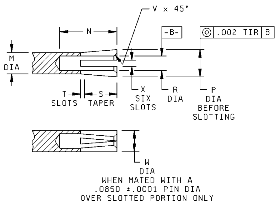
FIGURE 402-2. Interface, test connector, series N, socket contact.
