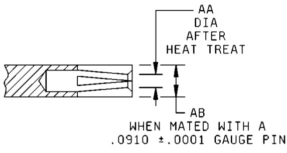
FIGURE 401-2. Interface test connector, series C, socket contact.
