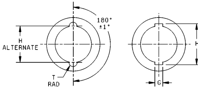
FIGURE 301-1. Interface, series BNC, pin contact.
