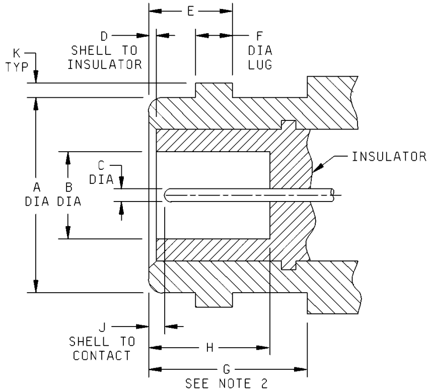
RECEPTACLE WITH PIN CONTACT
