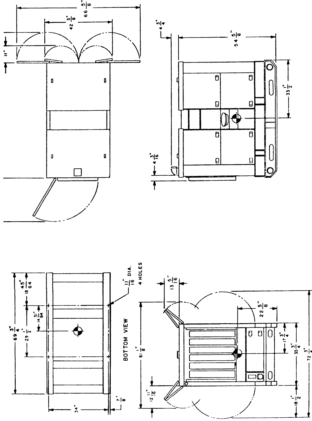
FIGURE 24. MEP-004A (15 kW, 50/60 Hz, DED).
