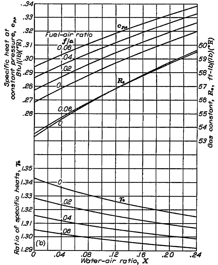
(b) Exhaust gas-water vapor mixture. Temperature, 1650° R; hydrogen-carbon ratio, 0.175. FIGURE 3.—Concluded. Thermodynamic properties of mixtures at pressure of 0 pound per square inch absolute.
