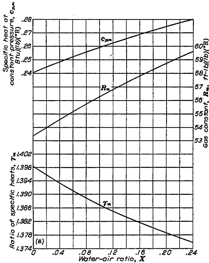
(a) Air-water vapor mixture. Temperature, 600° R.
