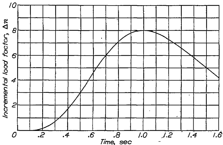
FIGURE 2.—Variation of load-factor increment. \Delta n = 8(t)^{1/2} e^{-0.7t} .
