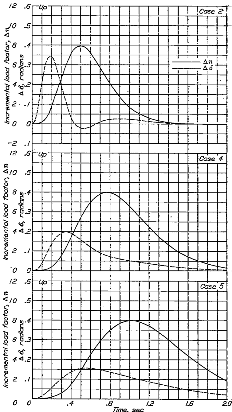
FIGURE 8.—Effect of t 1 on incremental-tail-load components. Center of gravity, 0.247.
