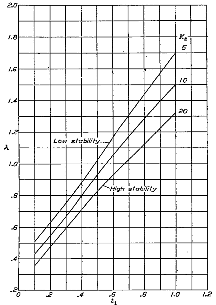
FIGURE 4.—Variation of \lambda with t_1 .
