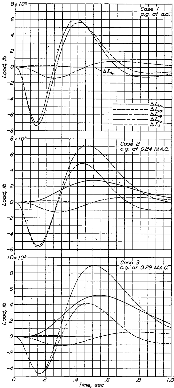
FIGURE 7.—Effect of center-of-gravity position on incremental-tail-load components.
