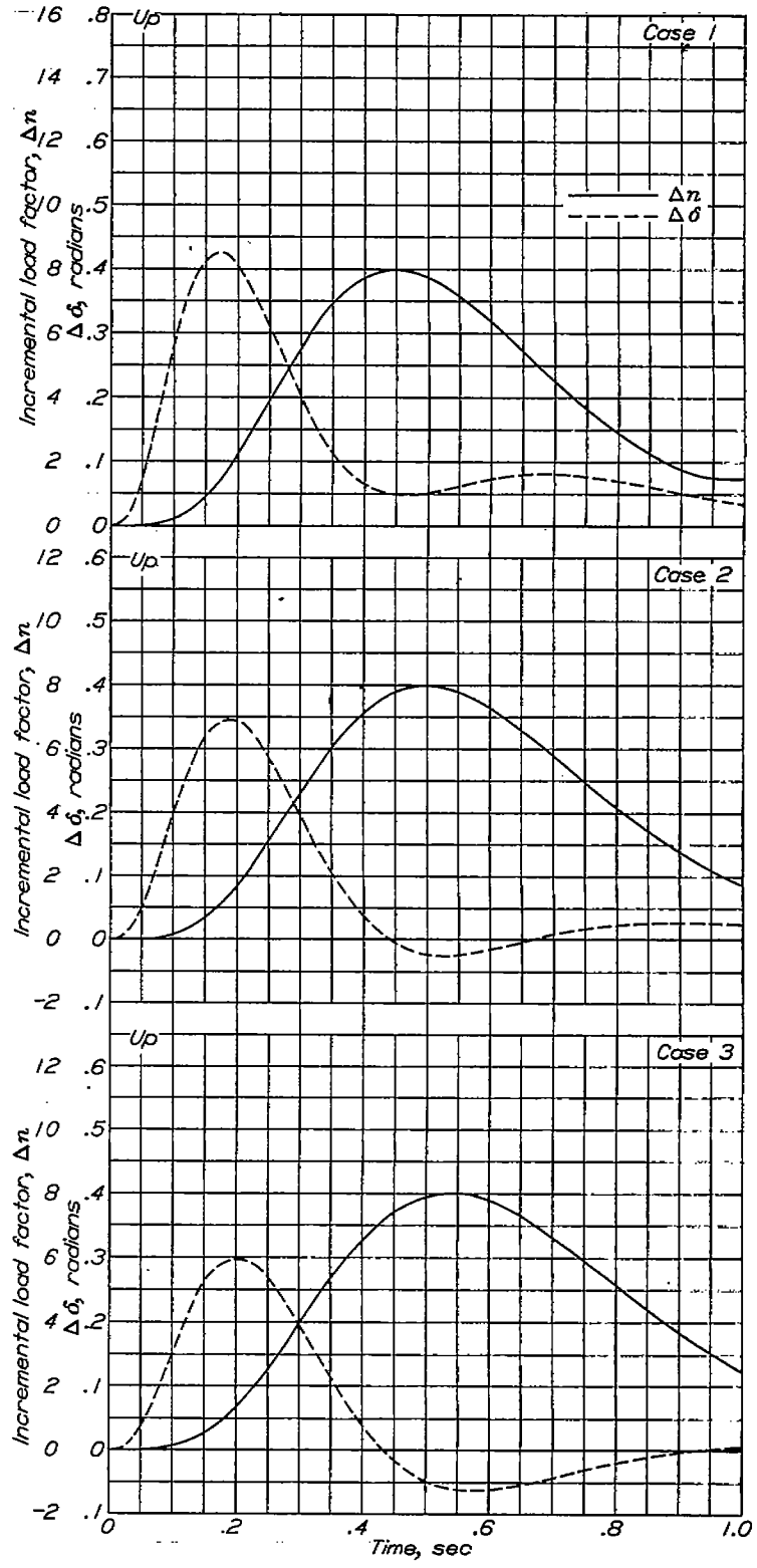
FIGURE 7.—Effect of center-of-gravity position on incremental-tail-load components.
