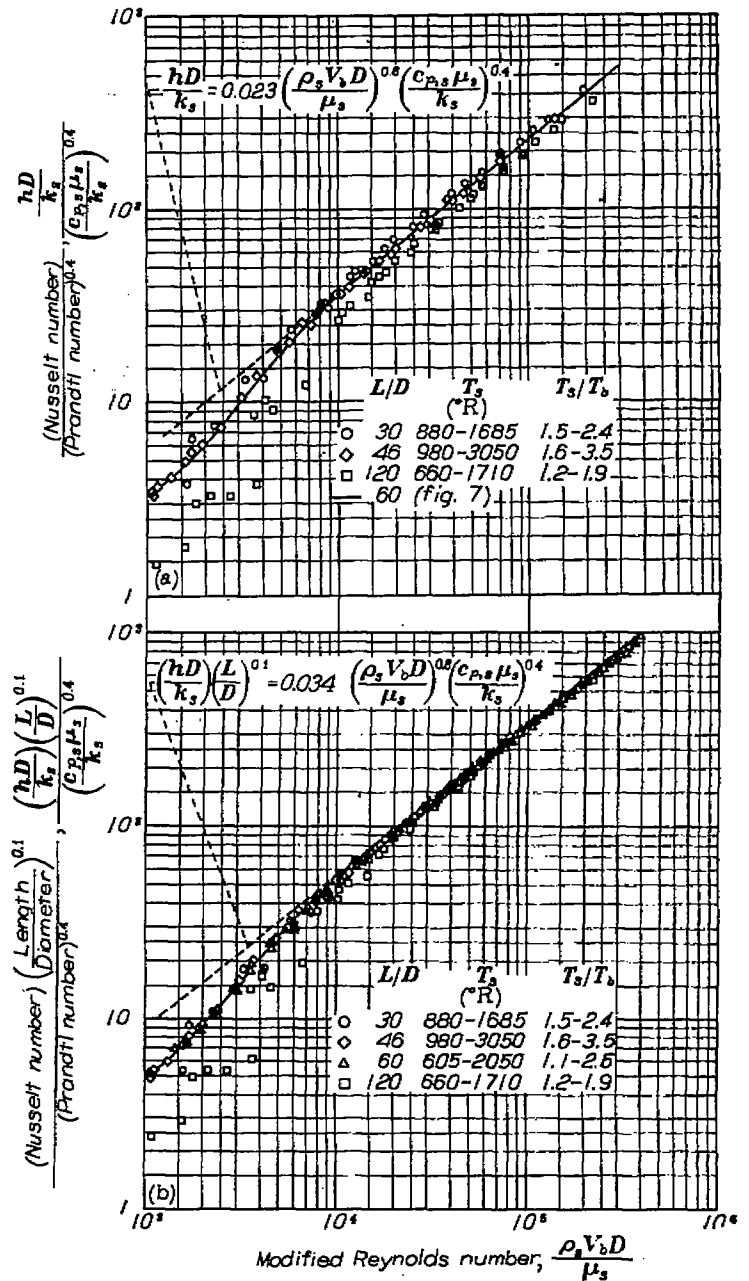
FIGURE 9.—Effect of ratio of length to diameter using modified method of correlating heat transfer coefficients. Inconel and platinum tubes; inlet-air temperature, 535° R; physical properties of air evaluated at surface temperature.
