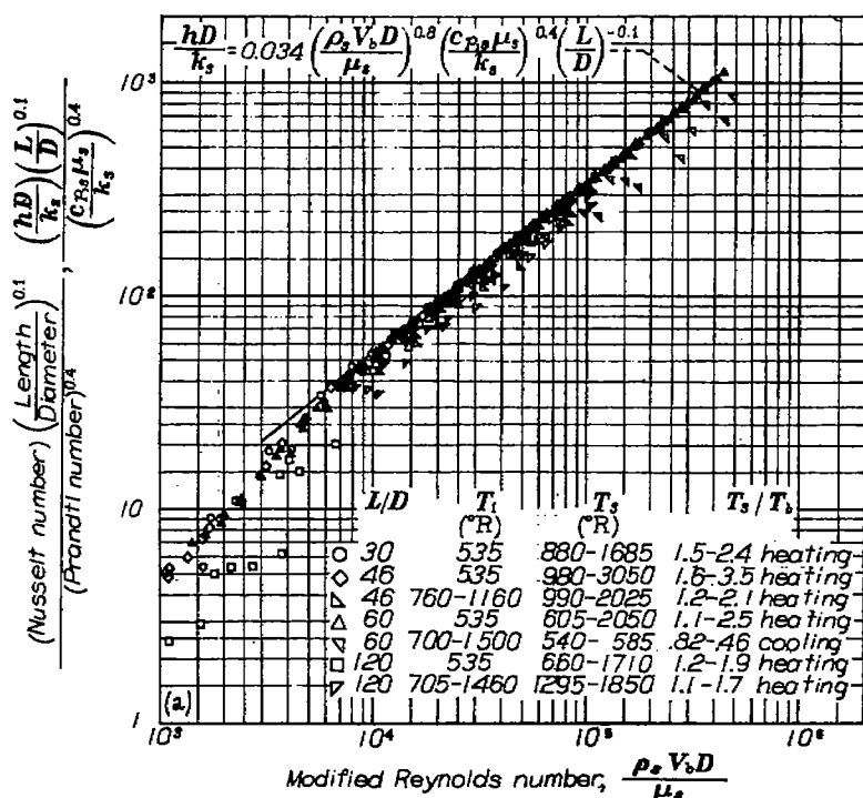
(a) Physical properties of air evaluated at surface temperature T_s ; thermal conductivity proportional to T^{0.84} .
