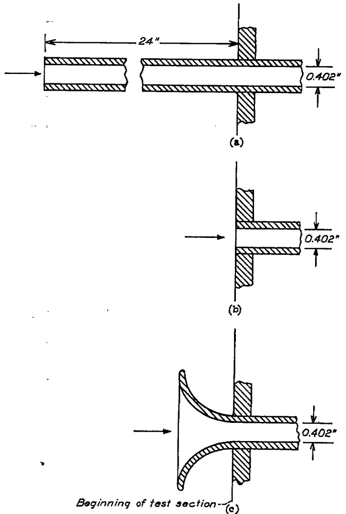
FIGURE 2.—Entrances to test sections.
