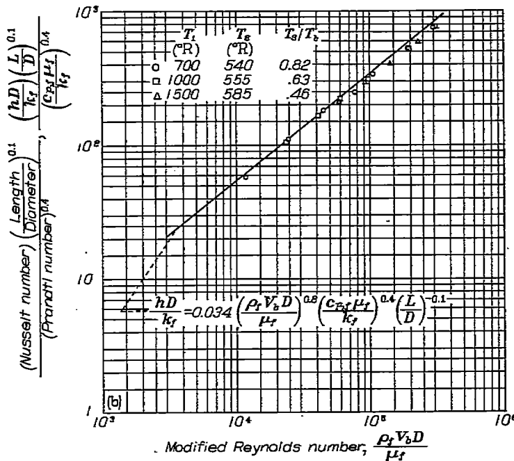
(b) Physical properties of air evaluated at film temperature T_f ; thermal conductivity proportional to \sqrt{T} .
