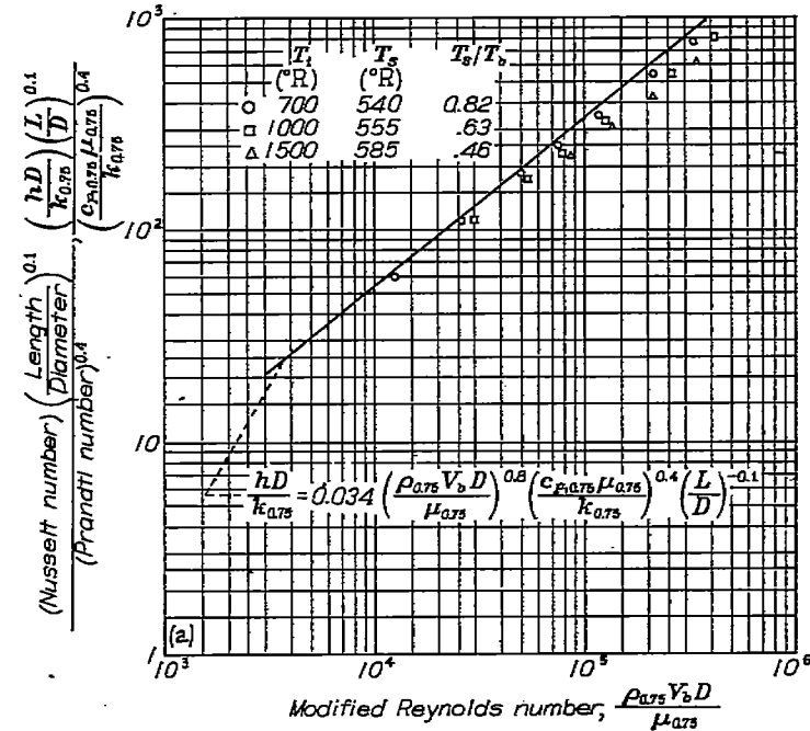
(a) Physical properties of air evaluated at film temperature T_{f,0.75} ; thermal conductivity proportional to T^{0.75} .
