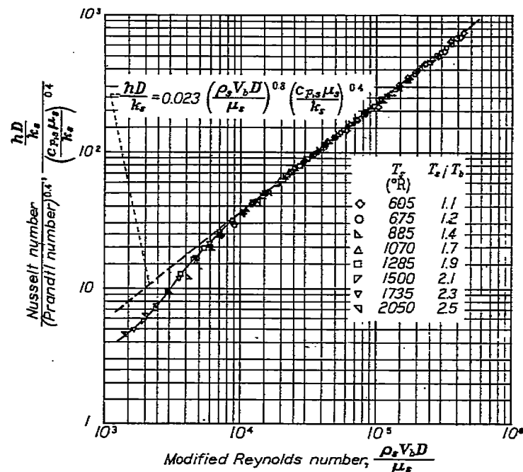
FIGURE 7.—Modified method of correlating heat-transfer coefficients. Inconel tube; length-diameter ratio, 60; bellmouth entrance; inlet-air temperature, 535° R; physical properties of air evaluated at surface temperature.
