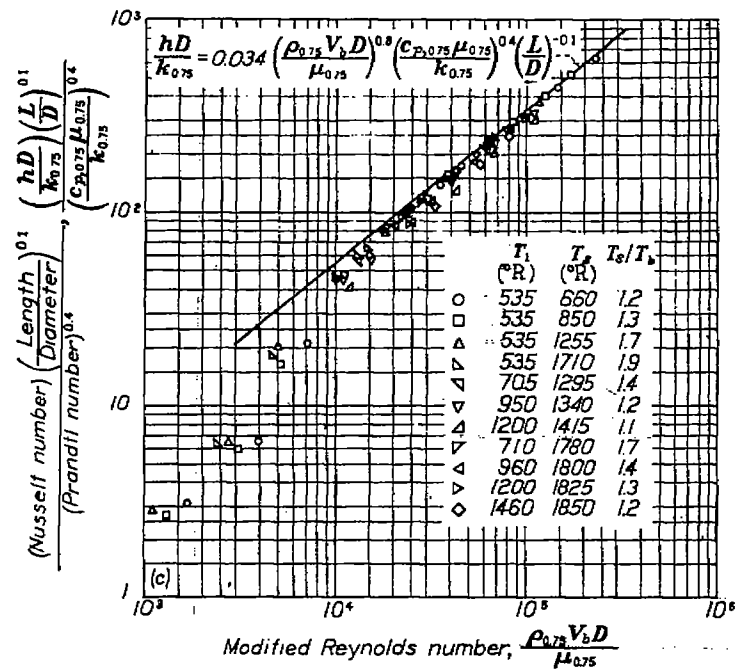
(c) Physical properties of air evaluated at film temperature T_f ; thermal conductivity proportional to T^{0.75} ; Inconel tube.
