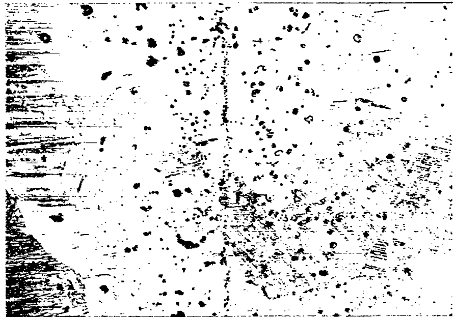
FIGURE 8.—Central portion of diffusion zone of specimen 10. Annealed 7.17 days at 1297° C; etchant, 5-percent nitric acid in ethyl alcohol followed by aqua regia in glycerine; magnification, X100. Photograph shows accumulation of oxides near center of diffusion zone. (Magnification increased 6.2 percent in printing.)
