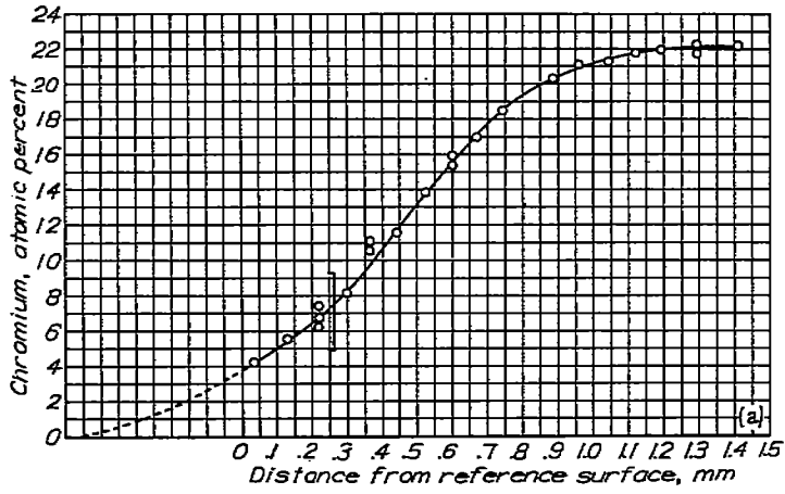
(a) Specimen 1; annealed at 1360° C for 3.334×10 5 seconds (3.92 days). Data to left of bracket are inaccurate because of quench crack that formed after diffusion took place.
