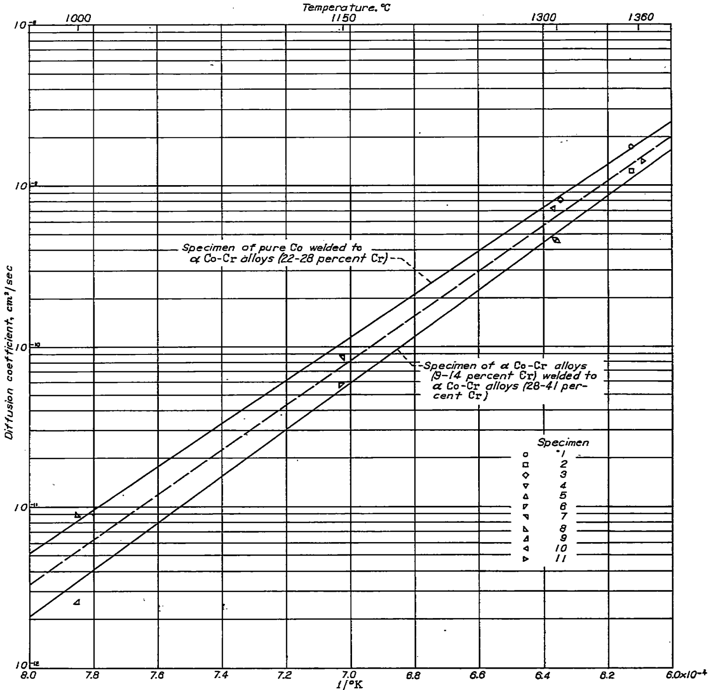
FIGURE 13.—Diffusion coefficients against 1/K . Diffusion coefficients were plotted from data for 16-atomic-percent chromium.
