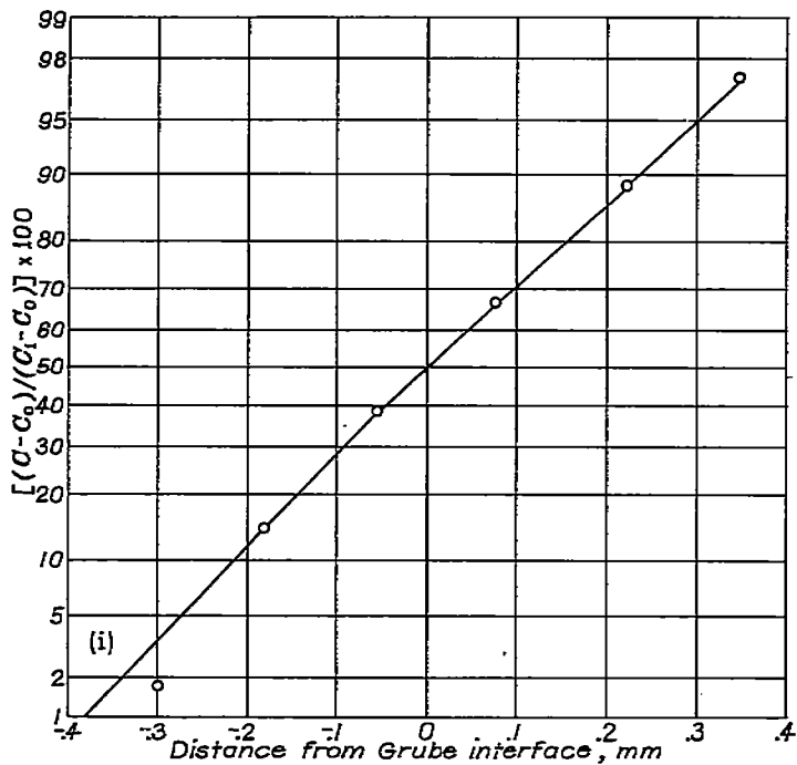
(i) Specimen 7; annealed at 1151° O for 24.91 days.
