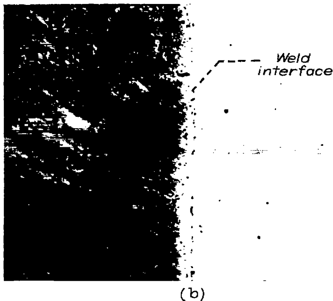
FIGURE 4.—Appearance of satisfactory and unsatisfactory welds. (Magnification increased 10.4 percent in printing.)
