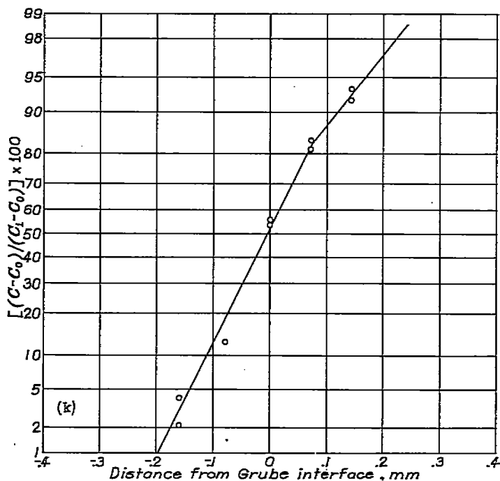
(k) Specimen 9; annealed at 1000° O for 87.7 days.
