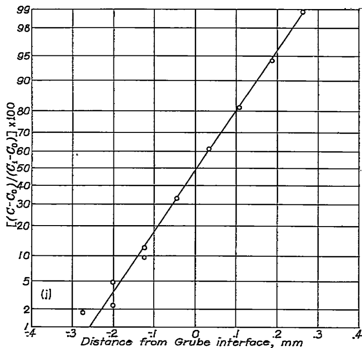
(j) Specimen 8; annealed at 1000° O for 87.7 days.
