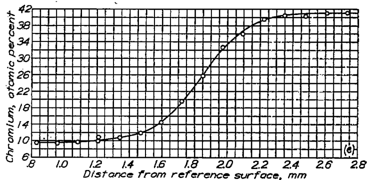
(e) Specimen 4; annealed at 1298° C for 6.218 \times 10^4 seconds (7.19 days).
