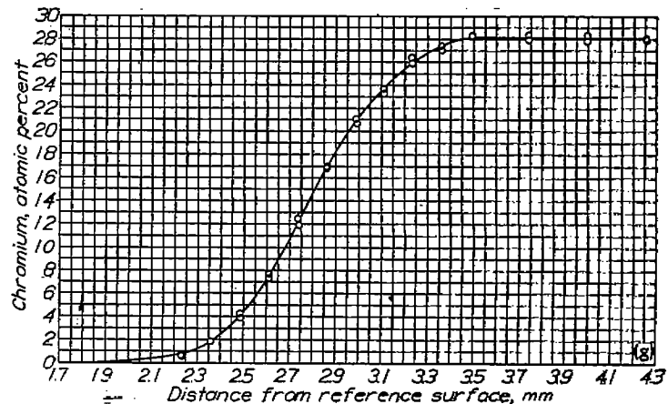
(g) Specimen 10; annealed at 1297° C for 6.108 \times 10^4 seconds (7.17 days).
