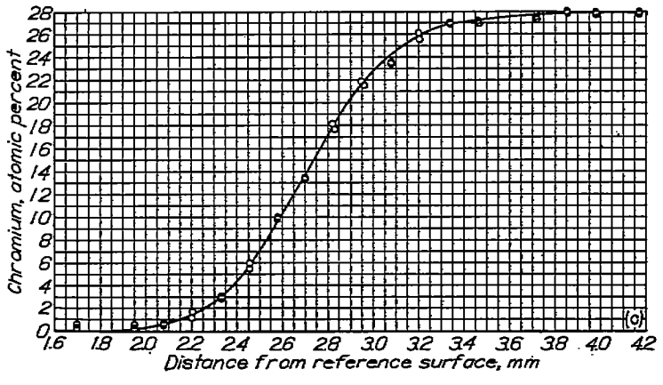
(c) Specimen 11; annealed at 1360° C for 3.321×10 5 seconds (3.84 days).
