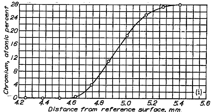
(i) Specimen 7; annealed at 1151° C for 2.152 \times 10^6 seconds (24.91 days).
