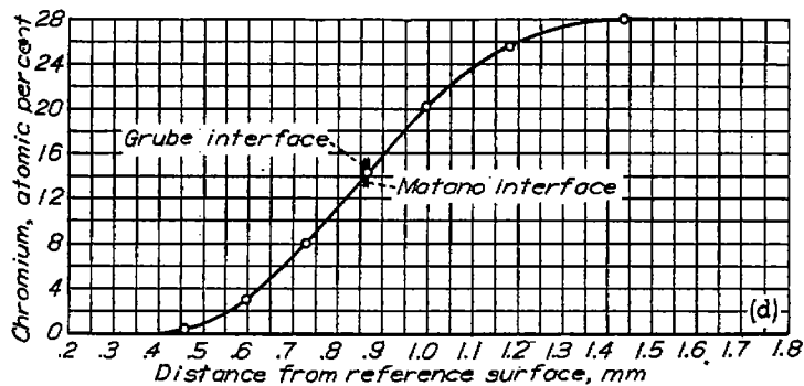
(d) Specimen 3; annealed at 1303° C for 3.622 \times 10^4 seconds (4.08 days).
