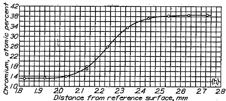
(h) Specimen 6; annealed at 1180° C for 1.0446 \times 10^6 seconds (12.09 days).
