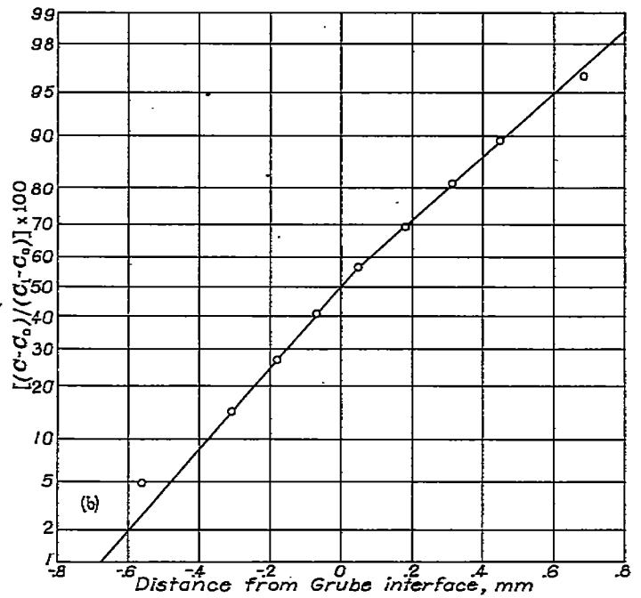
(b) Specimen 2; annealed at 1360° C for 3.92 days.
