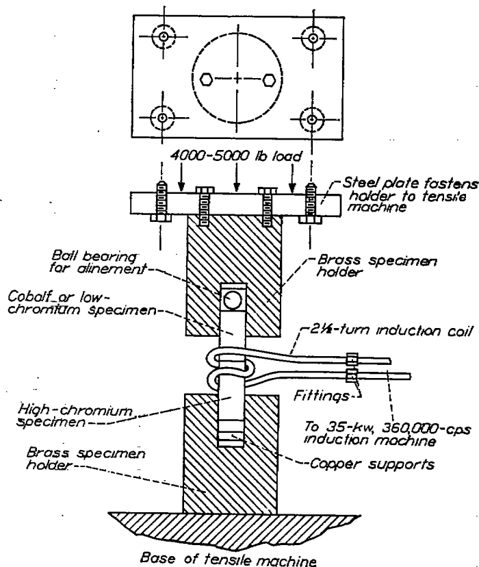
FIGURE 2.—Pressure-welding apparatus.
