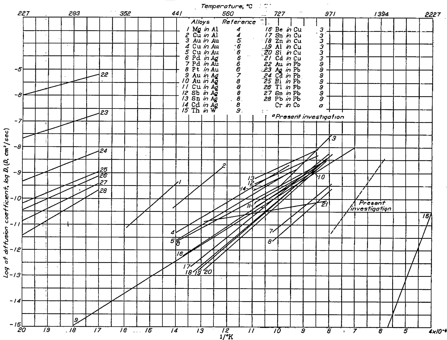
FIGURE 14.—Comparison of diffusion behavior of chromium in \alpha cobalt-chromium alloys with other substitutional solid-solution alloys.
