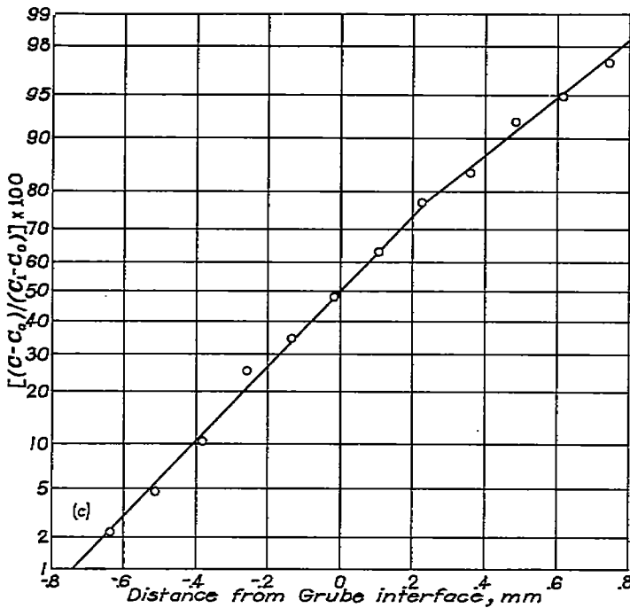
(c) Specimen 11; annealed at 1360° C for 3.84 days.
