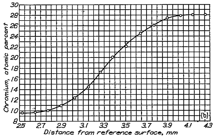
(b) Specimen 2; annealed at 1360° C for 3.334×10 5 seconds (3.92 days).
