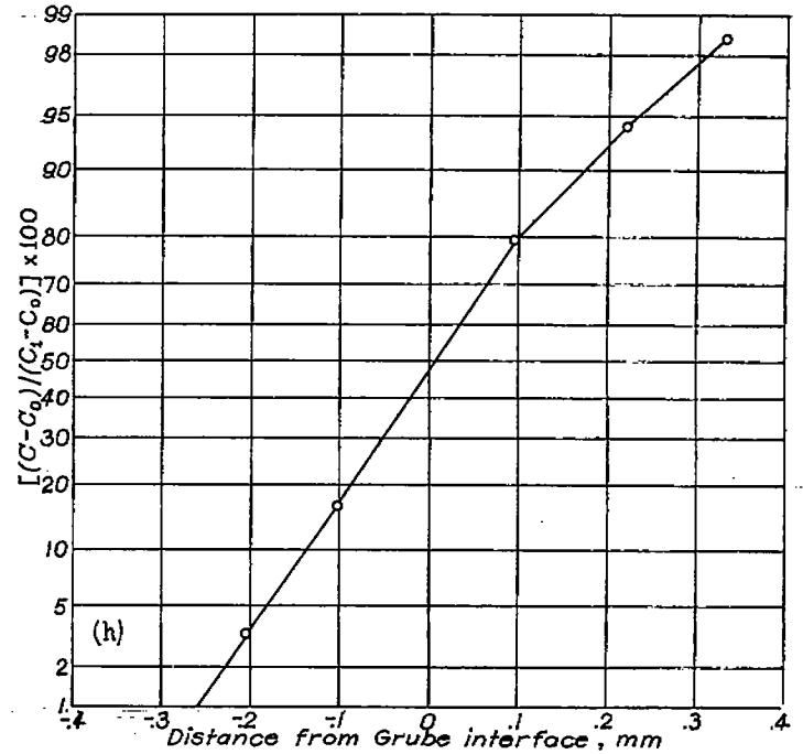
(h) Specimen 6; annealed at 1150° C for 12.09 days.
