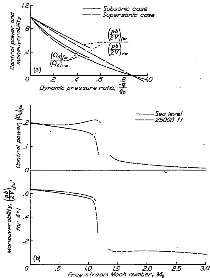
FIGURE 6.—Control power and effectiveness of example wing. (a) Variation with dynamic pressure ratio. (b) Variation with Mach number and altitude.
