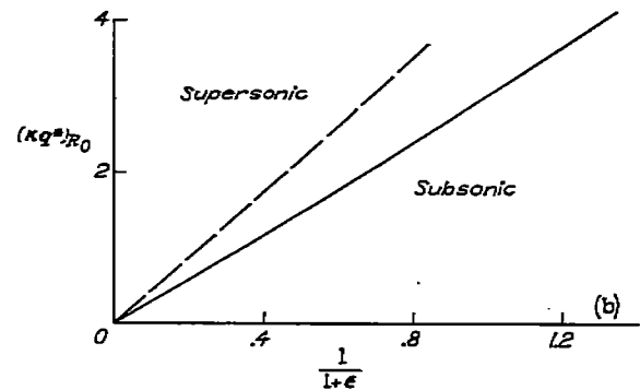
(a) Effect of sweep on reversal parameter (\kappa q^*)_R . (b) Effect of moment-arm ratio \epsilon on reversal parameter (\kappa q^*)_R for unswept wings. FIGURE 7.—Effects of sweep and moment-arm ratio on reversal speed.
