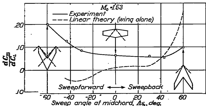
FIGURE 7.—Effect of sweep on moment-curve slope.
