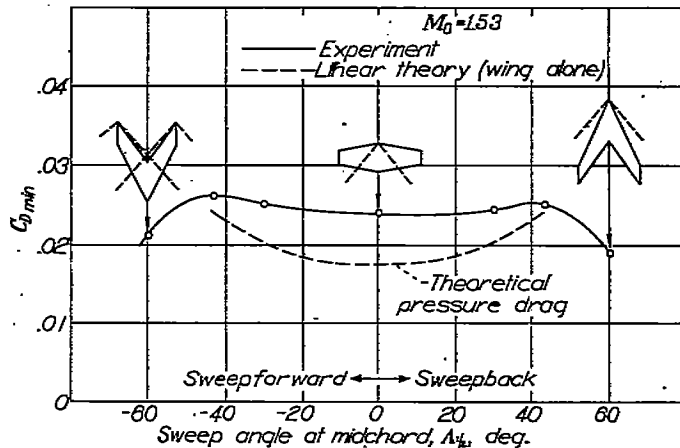
FIGURE 8.—Effect of sweep on minimum drag.
