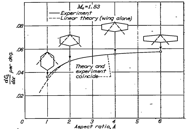
FIGURE 4.—Effect of aspect ratio on lift-curve slope.
