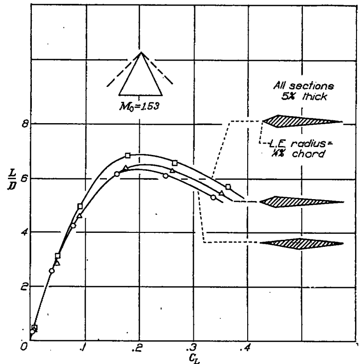
FIGURE 12.—Effect of wing section on lift-drag ratio of triangular wings.
