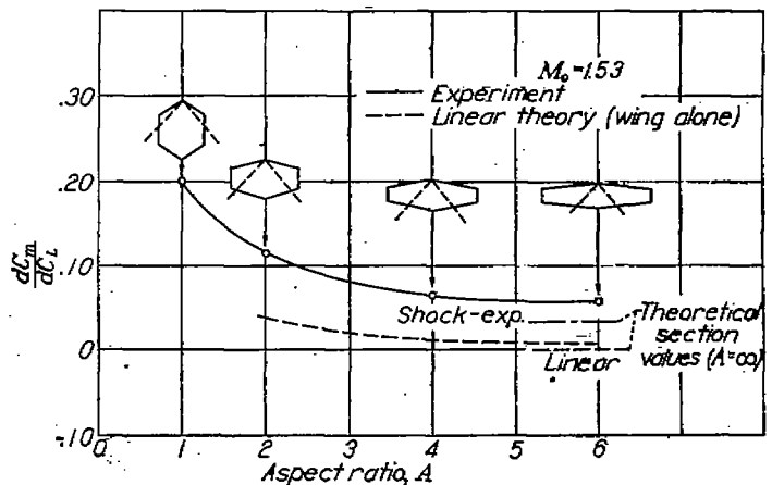
FIGURE 6.—Effect of aspect ratio on moment-curve slope.
