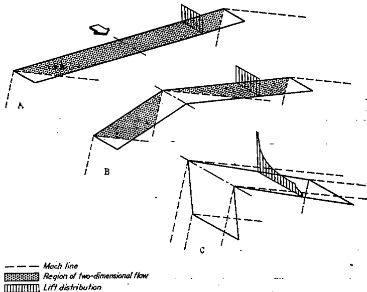
FIGURE 1.—Flat lifting surfaces in supersonic flow (linear theory).
