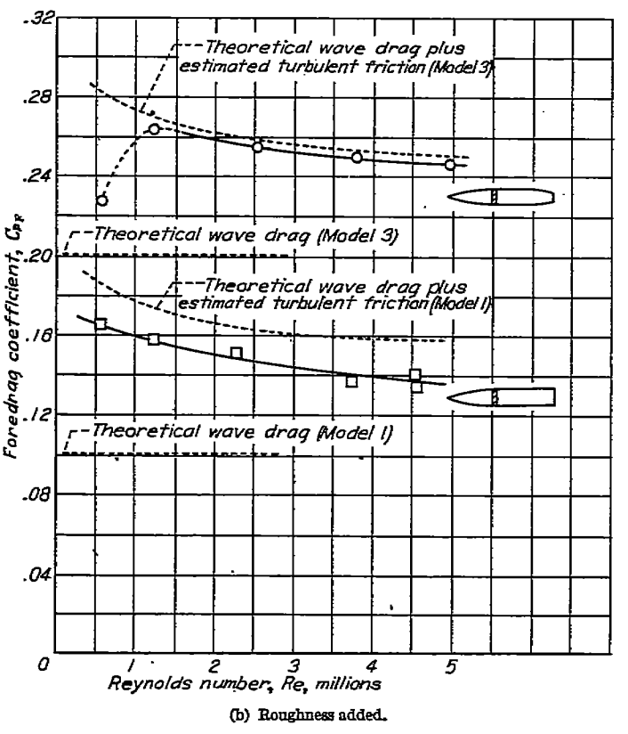
FIGURE 24.—Comparison of theoretical and experimental foredrag coefficients for models 1 and 3.
