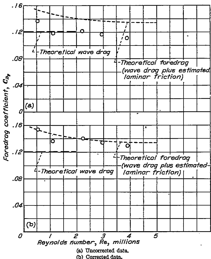
FIGURE 6.—Comparison of the foredrag coefficient of model 9 with and without corrections applied for the axial variation of the test-section static pressure.
