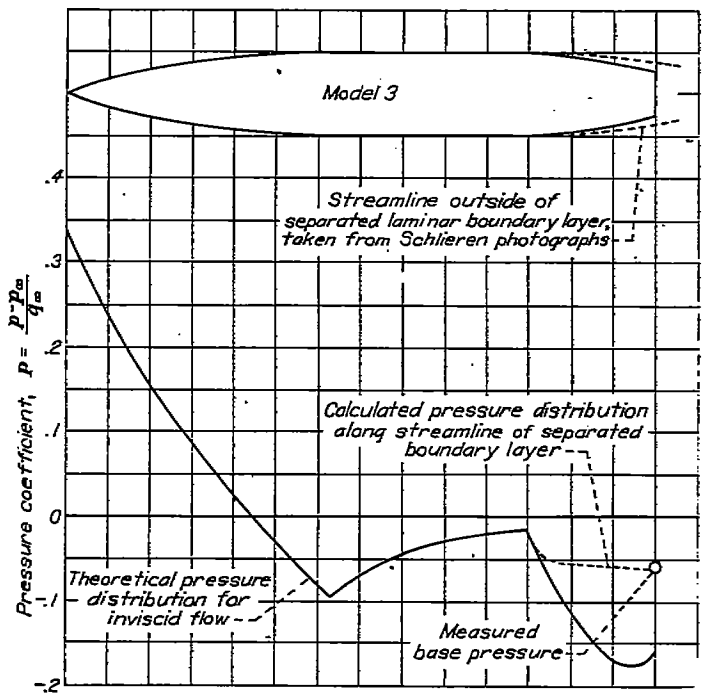
FIGURE 15.—Calculated pressure distribution for model 3 at a Reynolds number of 0.6 \times 10^6 .
