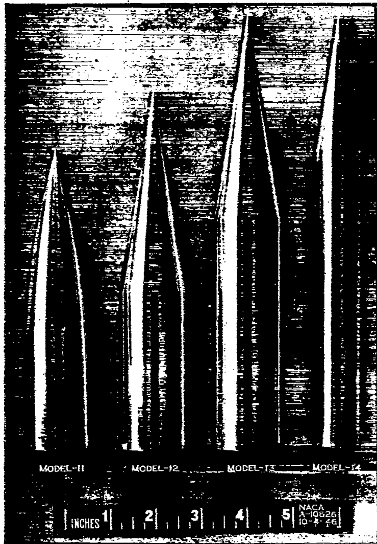
(b) Models used to evaluate effect of length-diameter ratio on base pressure.
