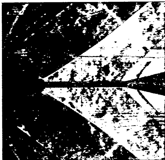
Re=3.9 \times 10^6
