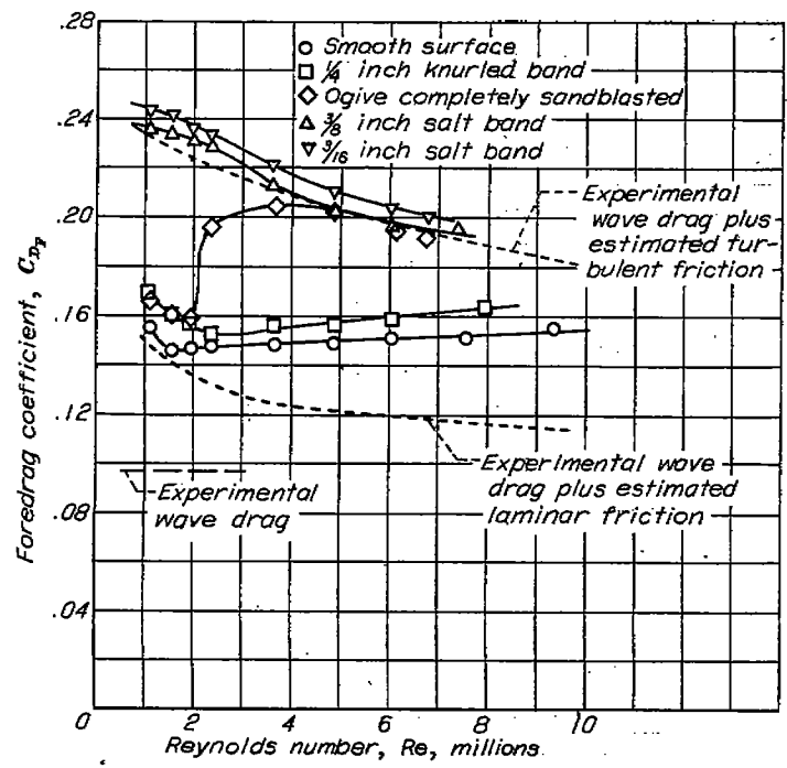
FIGURE 14.—Variation of foredrag coefficient with Reynolds number for model 8 with various amounts of roughness.
