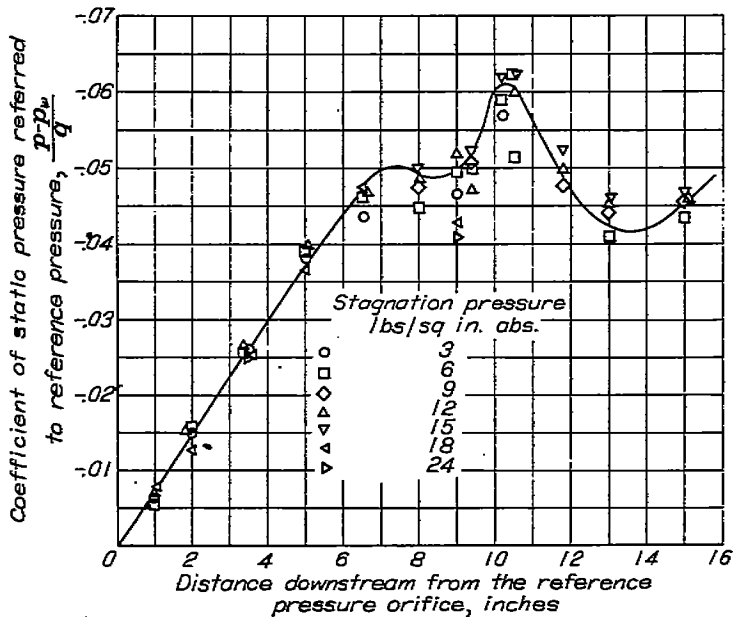
FIGURE 5.—Axial variation of the static pressure in the test section of the M=1.5 nozzle.
