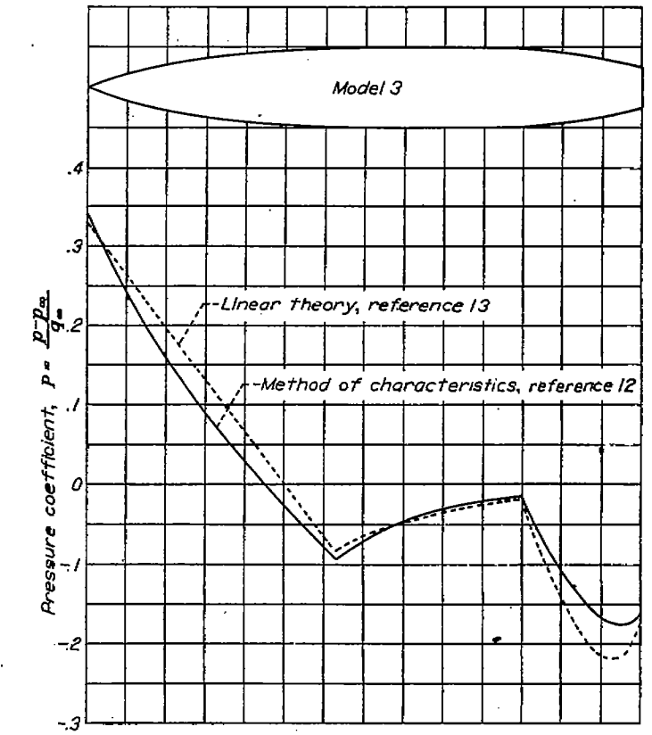
FIGURE 8.—Typical pressure distribution for a boattailed body at 1.5 Mach number.
