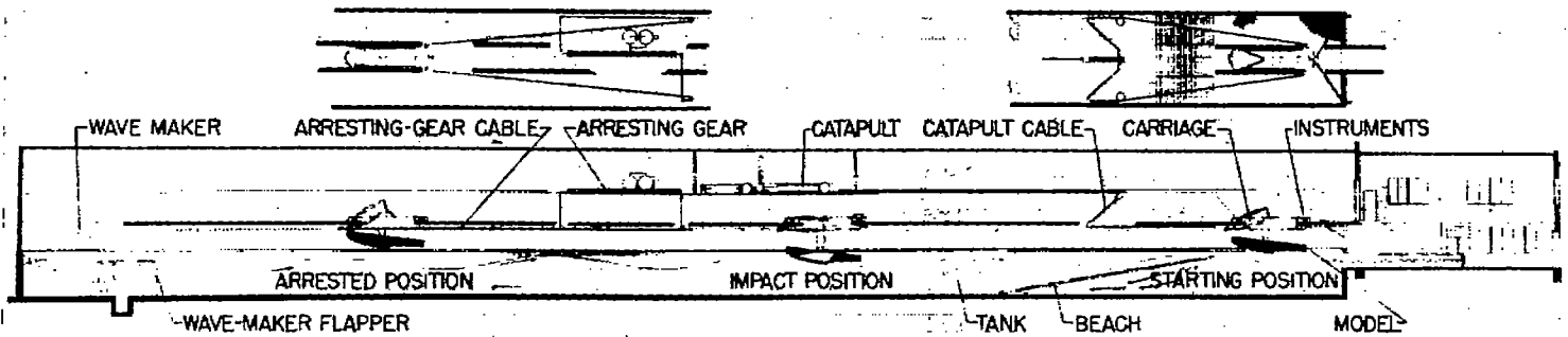
FIGURE 1.—Sketch of Langley impact basin. Length, 360 feet; width, 24 feet; depth, 11 feet; water depth, 8 feet.
