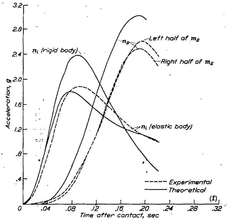
(e) Run 18: \tau=9^\circ ; \gamma_0=5.87^\circ ; \frac{t_n}{t_i}=0.79 ; V_0=58.8 feet per second.
