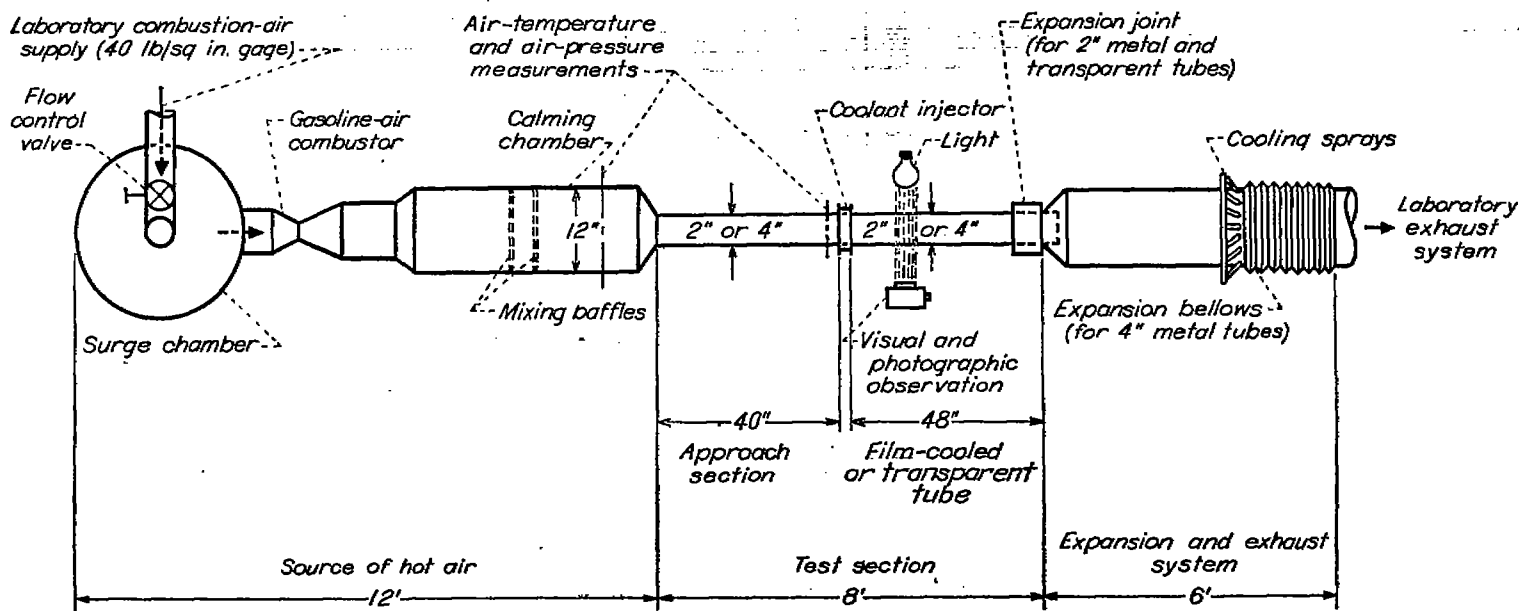
FIGURE 2.—Flow system.
