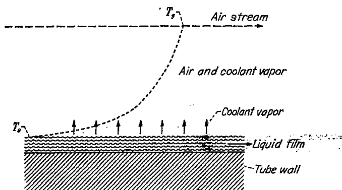
FIGURE 1.—Schematic representation of liquid film vaporizing in air stream.
