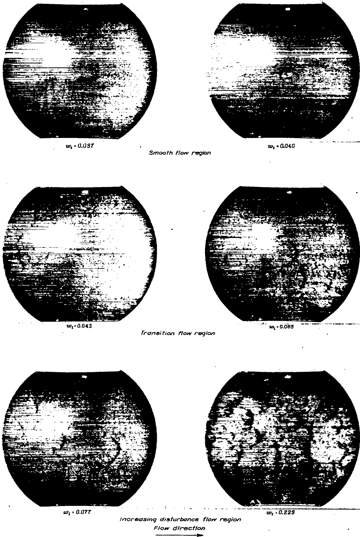
FIGURE 3.—Shadowgraphs of water films with cocurrent air flow in horizontal tube. Clear plastic tube of 4-lbth diameter; air-stream Reynolds number, 11.8 \times 10^4 ; air temperature, 80^\circ \text{F} ; liquid flow w_f , pounds per second per foot of circumference.
