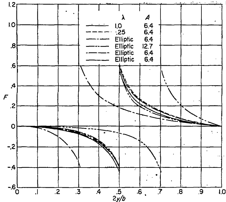
FIGURE 6.—Factor for altering two-dimensional data for several wings.
