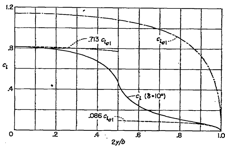
FIGURE 5.—Typical curves used to obtain factor for altering two-dimensional data.
