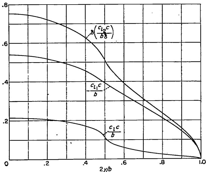
FIGURE 1.—Typical lift distributions for a wing with 0.5-span flaps.
