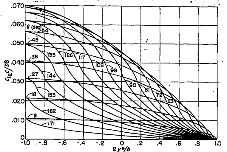
FIGURE 4.—Values of the lift distribution per degree of discontinuity in induced angle of attack as a function of the spanwise location of the discontinuity 2y^*/b .
