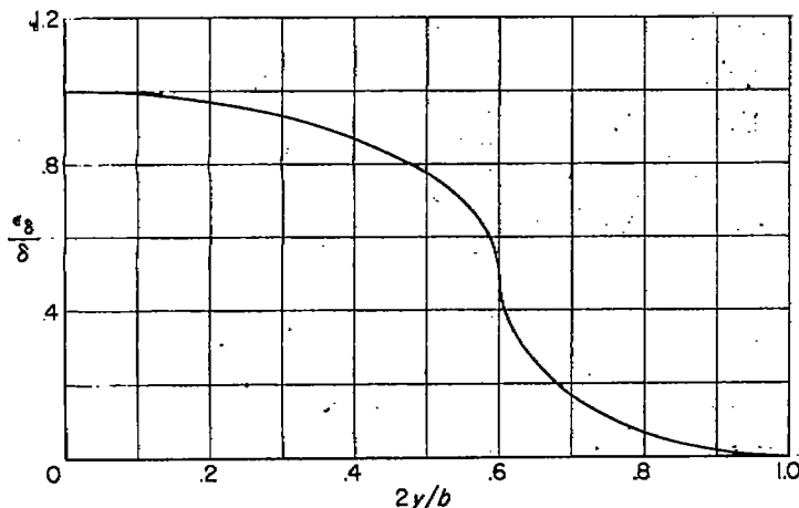
FIGURE 11. Fairing of discontinuity due to flap deflection for initial approximation.
