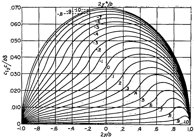
FIGURE 3.—Lift distribution per degree of discontinuity in induced angle of attack for various spanwise locations of the discontinuity 2y^*/b .
