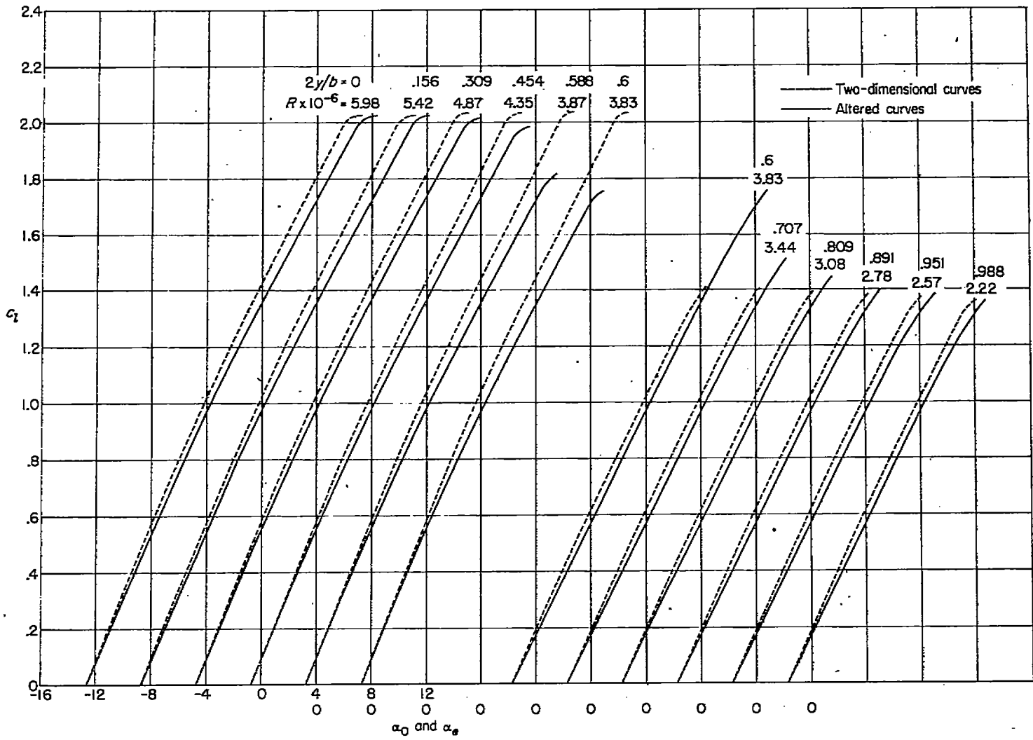
FIGURE 10.—Unaltered two-dimensional and altered section lift curves for example wing with 0.6-span flaps.
