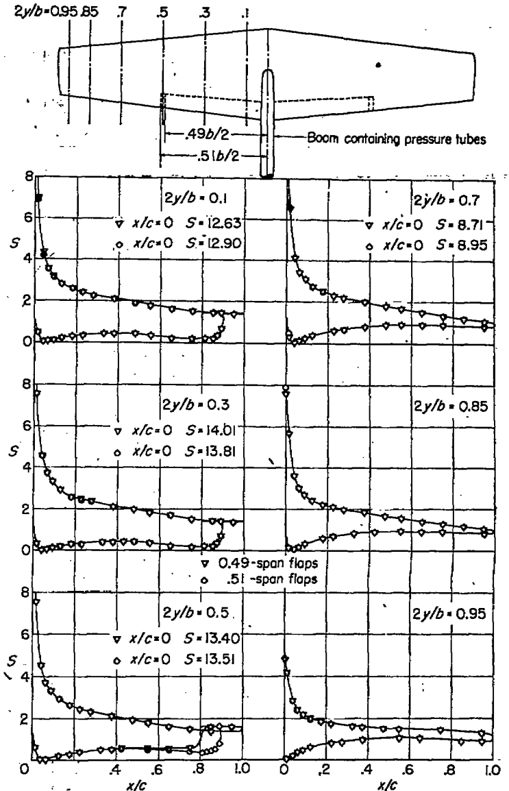
FIGURE 7.—Experimental pressure distributions at an angle of attack of 13.1^\circ for a wing having NACA 64-210 airfoil sections, an aspect ratio of 6.0, a taper ratio of 0.5, and partial-span split flaps.
