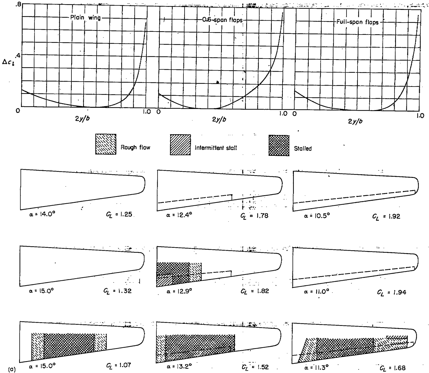
(a) NACA 64-210 sections; split flaps. FIGURE 14.—Experimental and calculated stalling characteristics for wings with and without flaps; aspect ratio, 9.021; taper ratio, 0.4; washout, 2°.
