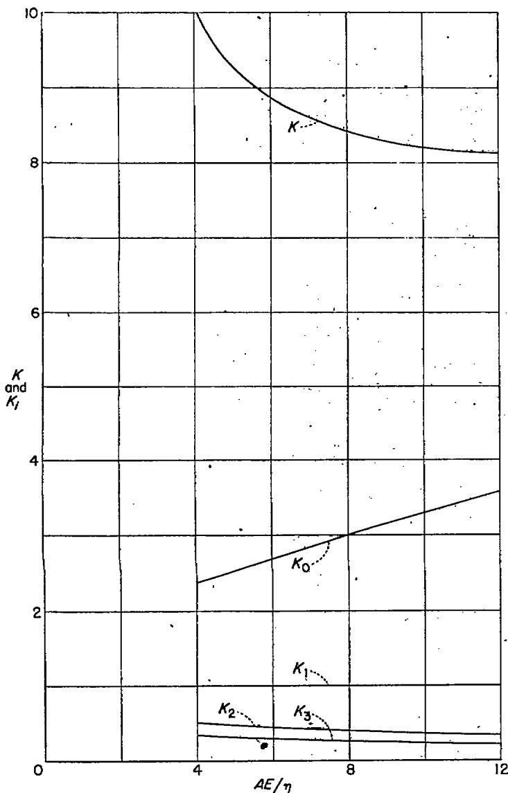
FIGURE 12.—Coefficients used to obtain succeeding approximations. r=20 .
