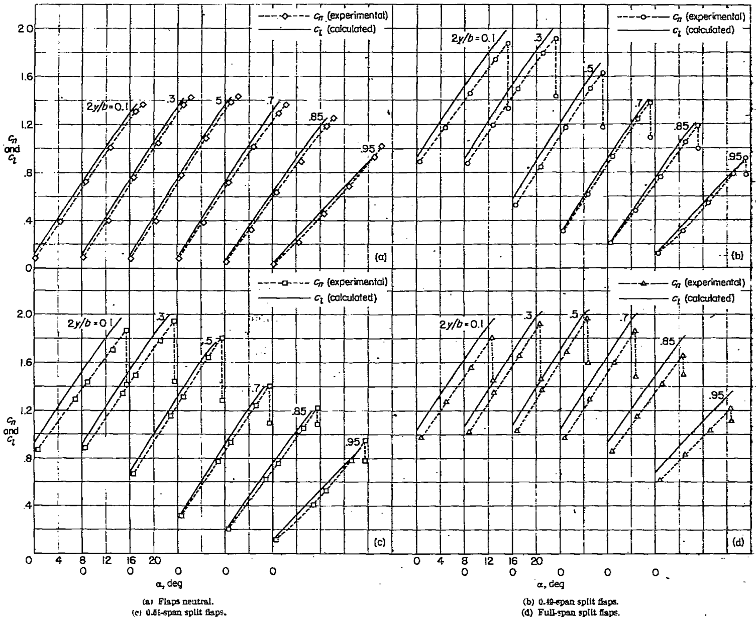
FIGURE 8.—Comparison of experimental and calculated section characteristics for a wing having NACA 64-210 airfoil sections, an aspect ratio of 6.0, and a taper ratio of 0.5.
