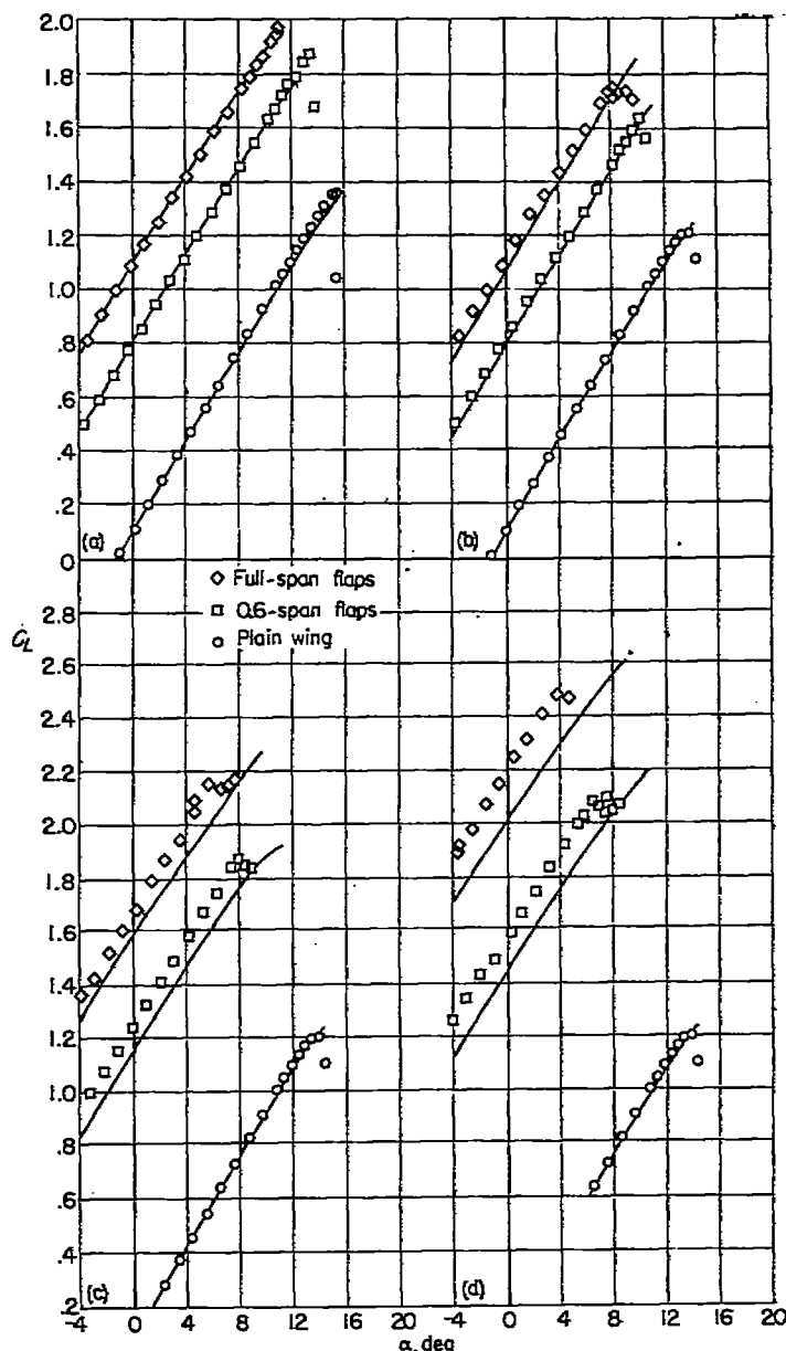
(a) NACA 64-210 sections; split flaps. (b) NACA 65-210 sections; split flaps. (c) NACA 65-210 sections; single slotted flaps. (d) NACA 65-210 sections; double slotted flaps.
