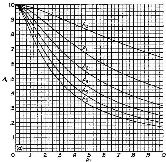
(a) A_i
