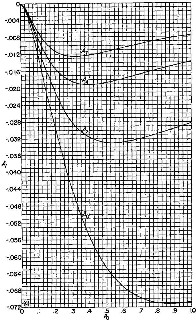
(c) \bar{A}_i .
