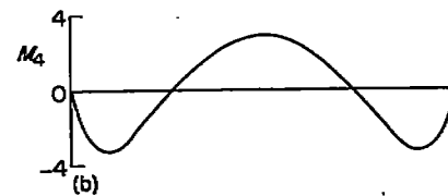
(b) Moment.
