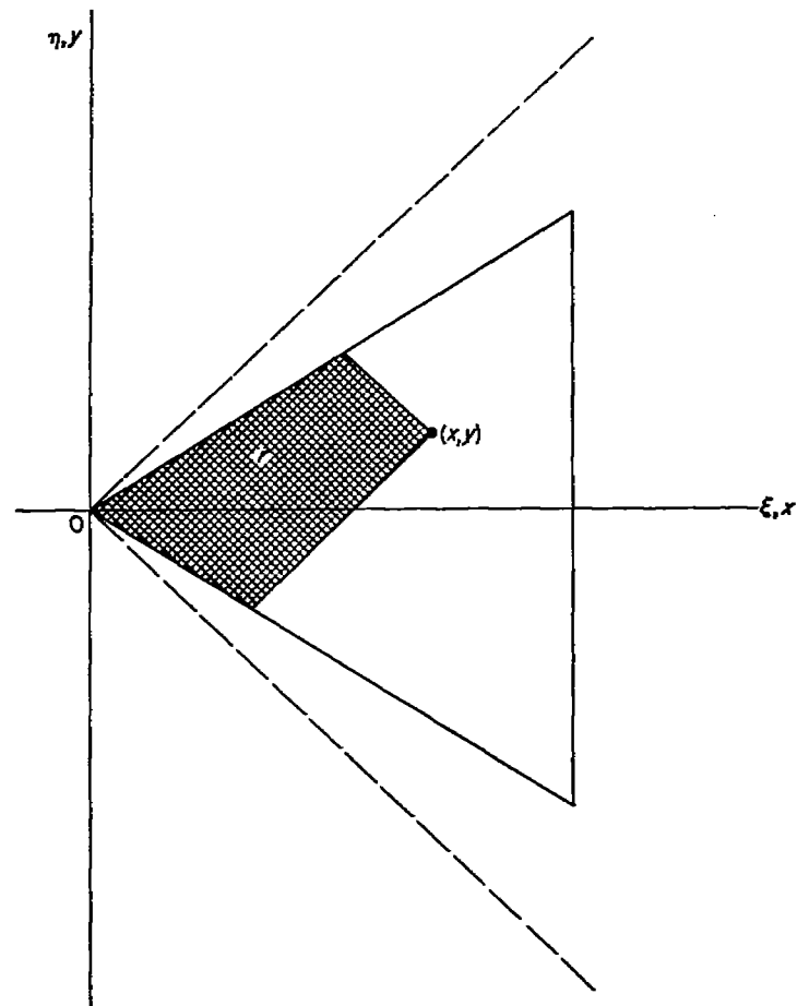
FIGURE 2.—Sketch illustrating region of integration for the velocity potential.
