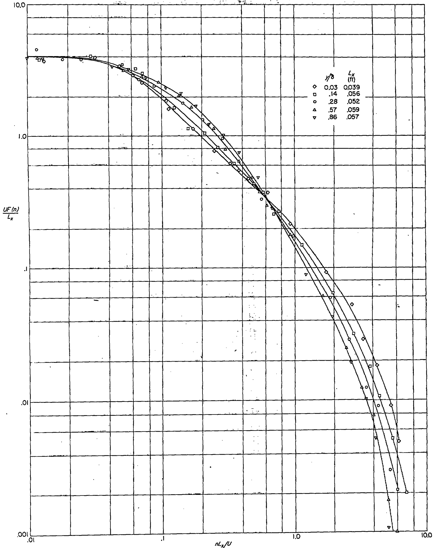
FIGURE 21.—Spectrum of \alpha -fluctuations in turbulent boundary layer resulting from free transition. x=10.5 feet; U_1=108 feet per second.
