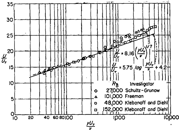
FIGURE 19.—Comparison of experimental results with \frac{1}{4} -power law and logarithmic law.
