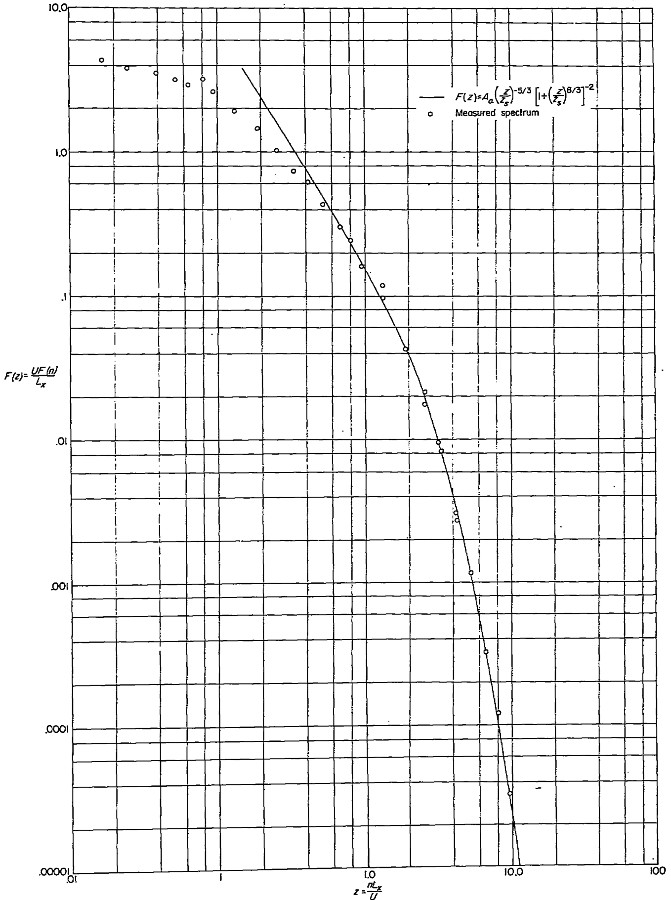
FIGURE 26.—Spectrum of isotropic turbulence compared with Heisenberg's interpolation formula. Measurements made 60 inches from 1-inch grid in uniform stream. A_0 = 0.0162 ; z_0 = 4.00 w'/U = 0.013 ; U = 60 feet per second; L_x = 0.047 foot; and \lambda = 0.010 foot
