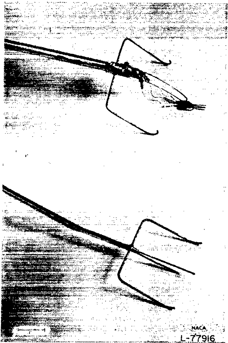
FIGURE 4.—Sliding hot-wire head and surface pitot-static tube.
