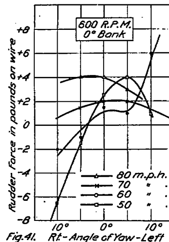
Fig. 41. Rt. - Angle of Yaw - Left
