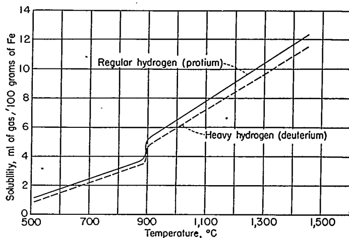
FIGURE 1.—Solubility-temperature curves for regular hydrogen and heavy hydrogen in ingot iron at atmospheric pressure as determined by Sieverts, Zapf, and Moritz (reference 6).
