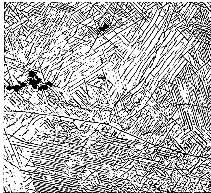
FIGURE 13.—Alloy 500 containing 65 percent chromium, 22 percent nickel, and 13 percent molybdenum. Etched and stained according to procedure 2; heavy Widmanstätten precipitate of sigma in epsilon phase; dark oxide inclusions and grain boundaries shown in epsilon phase; X500.
