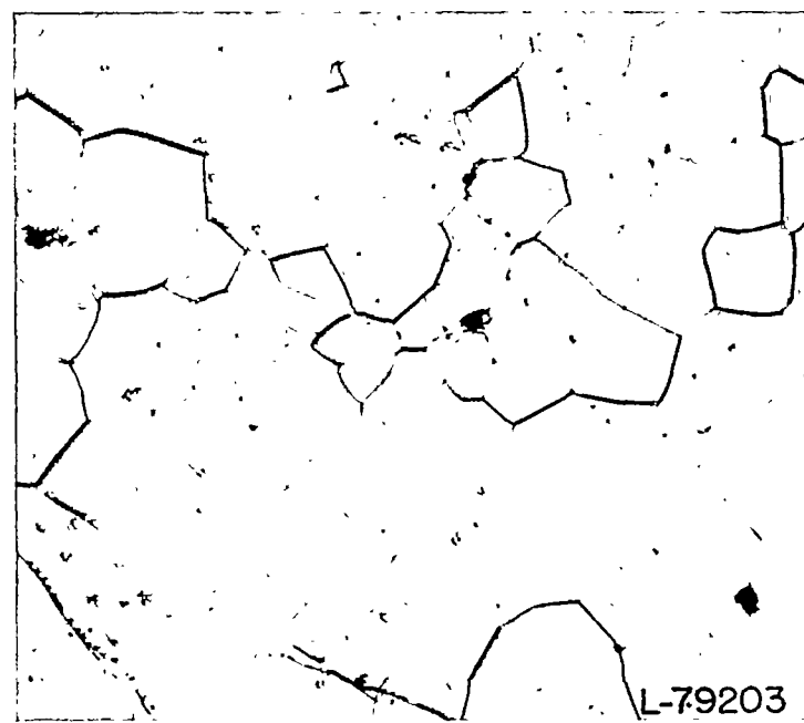
FIGURE 16.—Alloy 492 containing 20 percent chromium, 30 percent nickel, and 50 percent molybdenum. Etched and stained according to procedure 2; particles of sigma phase clearly delineated in matrix of P phase; grain boundaries revealed; X1,000.
