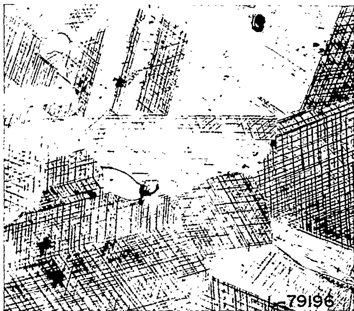
FIGURE 9.—Alloy 200 containing 38.02 percent chromium, 44.85 percent cobalt, 14.63 percent nickel, and 2.5 percent molybdenum. Etched according to procedure 1; small particles of second phase in an alpha matrix; transformation striations revealed in alpha phase; X600.
