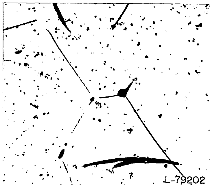
FIGURE 15.—Alloy 602 containing 25 percent chromium, 27.5 percent nickel, and 47.5 percent molybdenum. Etched and stained according to procedure 2; grain boundaries revealed in cracked matrix of sigma phase; X500.
