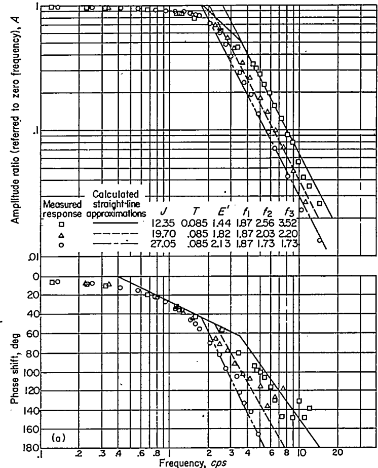
(a) Effect of load inertia J . Rotary servomotor; amplitude at zero frequency, 10°; pressure differential, 125 pounds per square inch.
