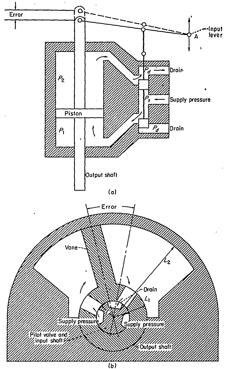
(a) Straight-line servomotor. (b) Rotary servomotor.
