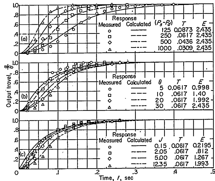
(a) Effect of pressure differential. Step input, 30°; moment of inertia of load, 12.35 pound inches per second per second. (b) Effect of magnitude of step. Moment of inertia of load, 12.35 pound inches per second per second; pressure differential, 250 pounds per square inch. (c) Effect of load inertia. Step input, 20°; pressure differential, 250 pounds per square inch.
