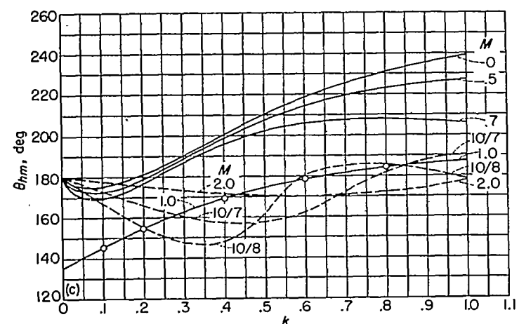
(c) Phase angle between moment vector due to vertical translation and vertical velocity vector \dot{h} .
