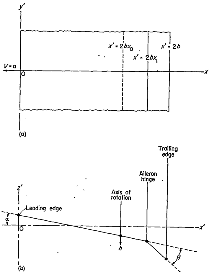
(a) Projection of wing strip on x'y' -plane. (b) Section y' = 0 . FIGURE 1.—Sketch illustrating coordinate system and the degrees of freedom \alpha , h , and \beta .
