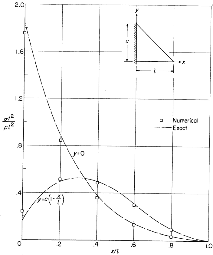
FIGURE 9.—Numerical and exact solutions of the differential equations (obtained by assuming linear chordwise deflections) for the maximum principal stresses along the free edges of a 45° delta plate of uniform thickness under uniform load.
