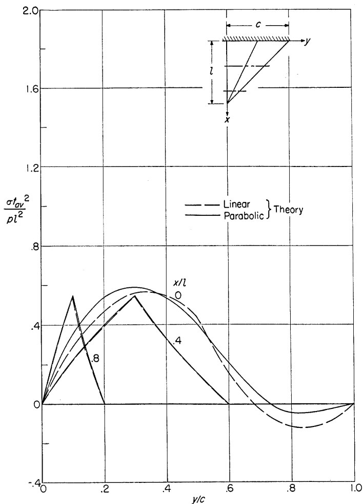
FIGURE 7.—Maximum principal stress in a 45° delta plate of symmetrical double-wedge airfoil section and constant thickness ratio under uniform load.
