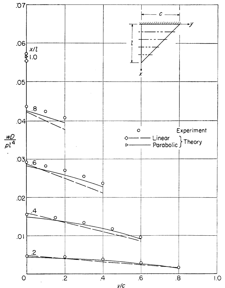
FIGURE 2.—Deflections of a 45° delta plate of uniform thickness uniform load.
