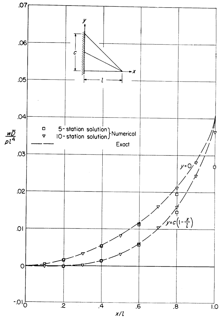
FIGURE 10.—Numerical and exact solutions of the differential equations (obtained by assuming linear chordwise deflections) for the deflections along the free edges of a 45° delta plate of symmetrical double-wedge airfoil section and constant thickness ratio under uniform load
