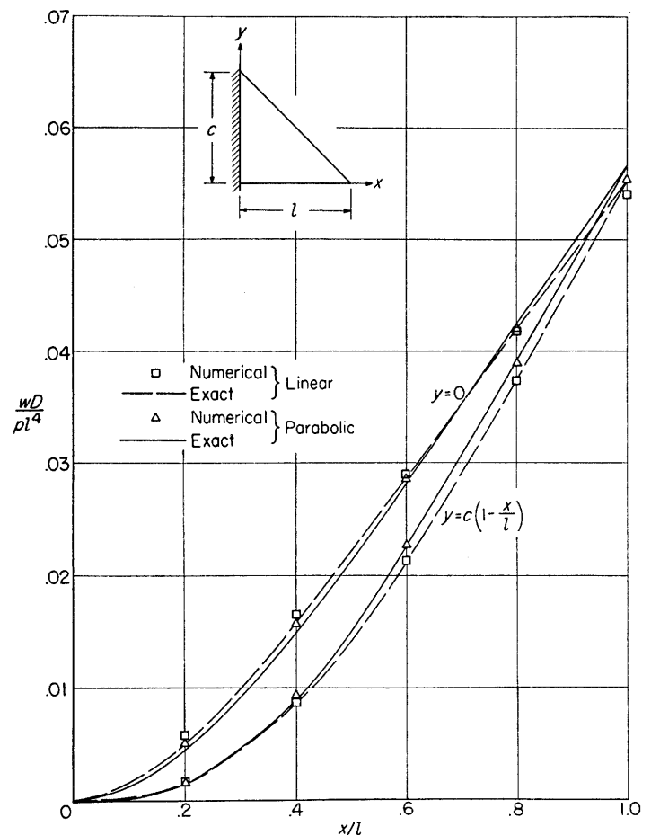
FIGURE 8.—Numerical and exact solutions of the differential equations for the deflections of the free edges of a 45° delta plate of uniform thickness under uniform load.
