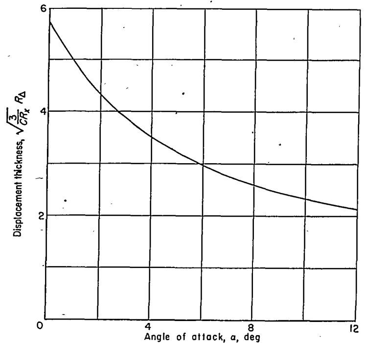
FIGURE 8.—Displacement thickness at \varphi=0 . M , 3.1; \theta , 7.5^\circ
