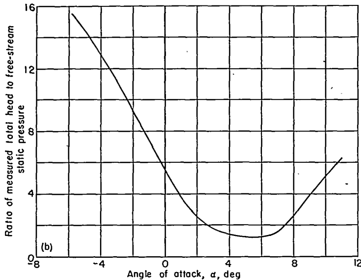
(a) Test configuration. (b) Variation of total head with angle of attack. FIGURE 4.—Variation with angle of attack of total head measured in boundary layer of cone. M , 3.095; \theta , 7.5°.
