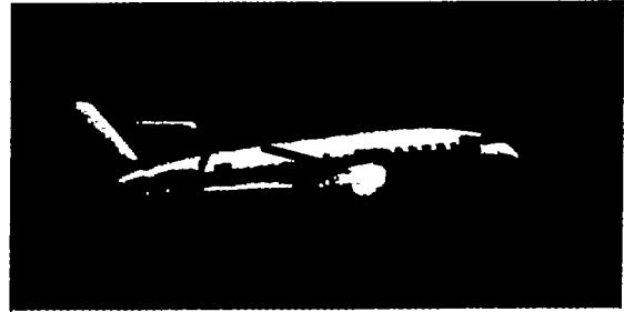
(b) Oil vapors emerging from nacelles; 3.88 seconds after initial impact. Airplane speed, approximately 3 feet per second.
