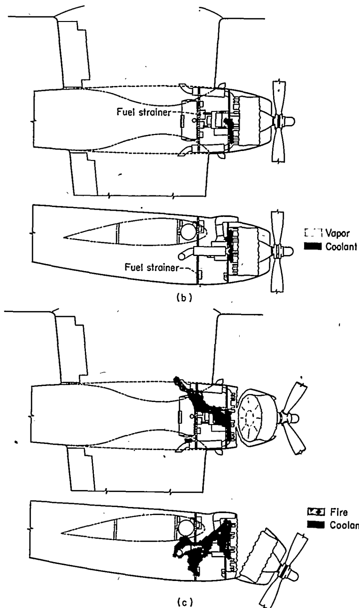
(b) Schematic diagram of nacelle showing location of combustible vapor and coolant in nacelle 0.75 second after initial impact. (c) Schematic diagram of nacelle showing fire indicated by detectors in nacelle 4.2 seconds after initial impact.
