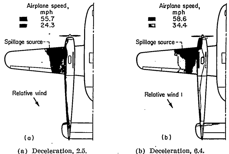
(a) Deceleration, 2.5. (b) Deceleration, 6.4. FIGURE 15.—Wetting pattern obtained with simulated fuel spillage during airplane taxiing tests.
