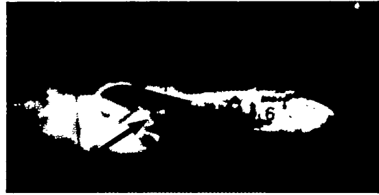
(b) Ignition on right side of airplane; 0.60 second after initial impact. Airplane speed, 135 feet per second.
