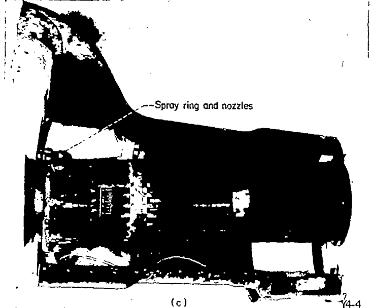
(b) Water-spray system for exhaust-collector ring. (c) Water sprays for exhaust heat exchanger.
